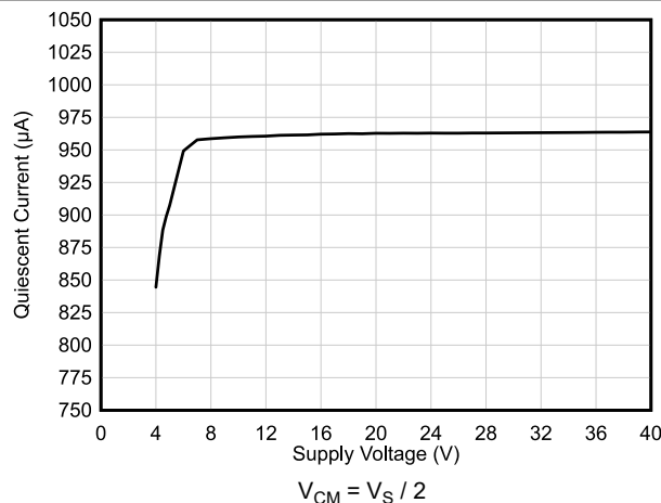
5-21. Quiescent Current vs Supply Voltage
