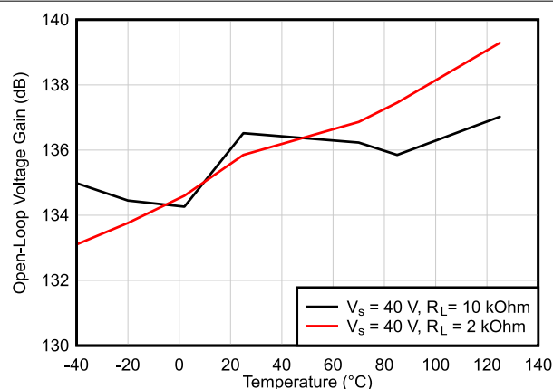
5-23. Open-Loop Voltage Gain vs Temperature (dB)
