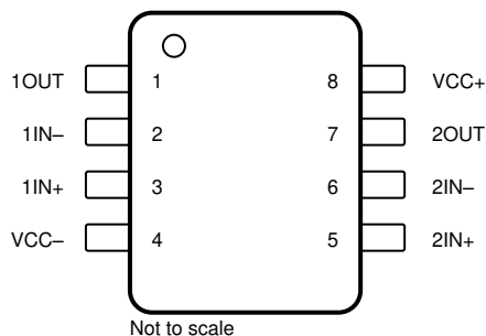
図 4-5. TL082x D, DDF, DGK, JG, P, PS, and PW Package, 8-Pin SOIC, SOT-23 (8), VSSOP, CDIP, PDIP, SO, and TSSOP (Top View)
