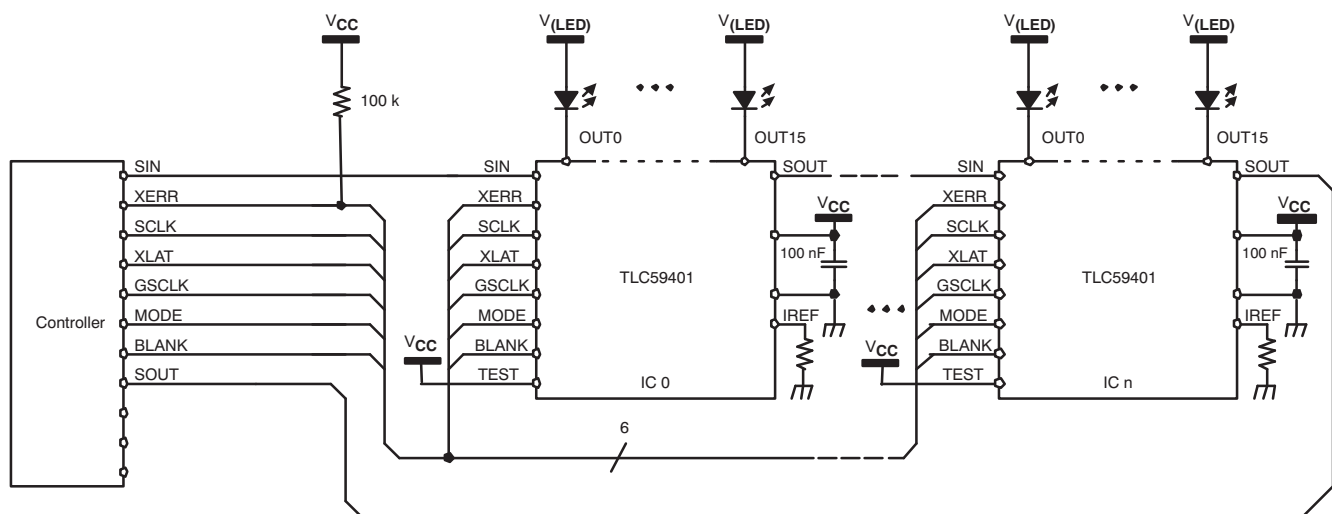
Figure 22. Cascading Devices
