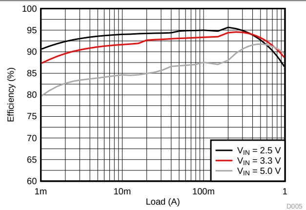
Figure 7. 1.8-V Output Efficiency
