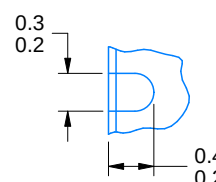
ALTERNATIVE TERMINAL SHAPE TYPICAL
