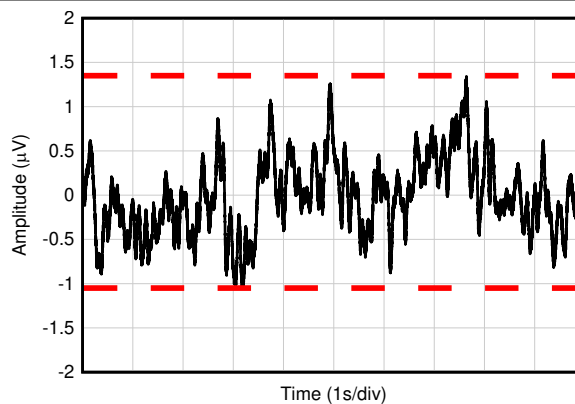
6-20. 0.1-Hz to 10-Hz Noise
