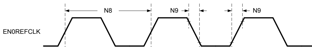
Figure 32-36. EN0RREF_CLK 50-MHz Oscillator Characteristics
