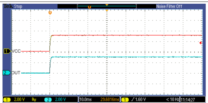
Figure 15. TMP303A Power-On Response, T_A Greater Than 60°C
