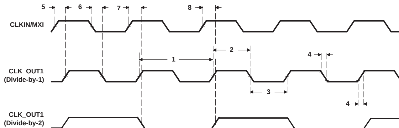
Figure 6-16. CLK_OUT1 Timing
