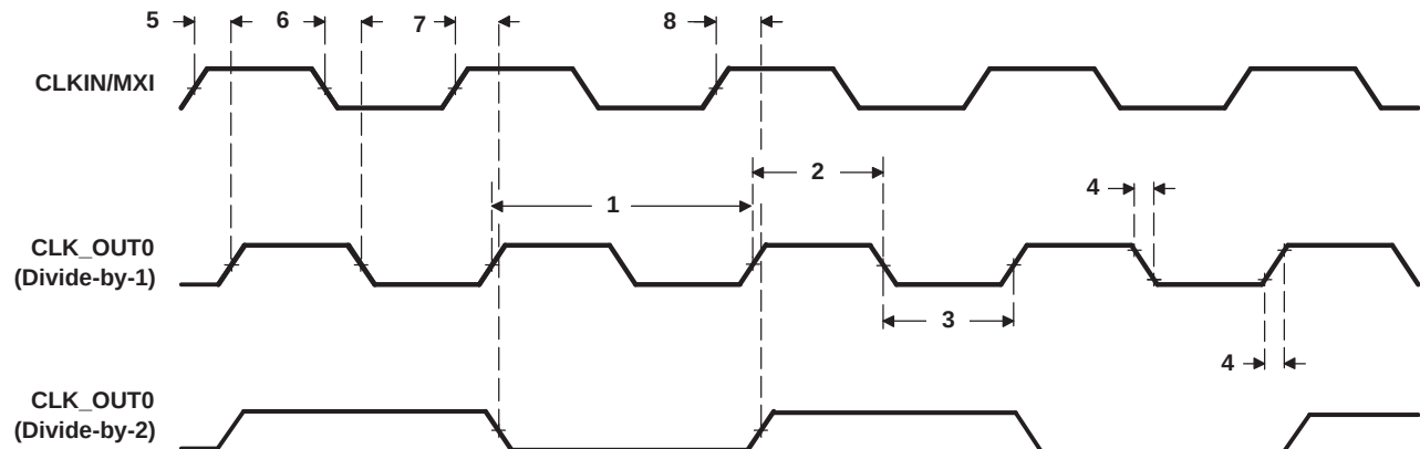
Figure 6-15. CLK_OUT0 Timing
