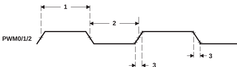
Figure 6-57. PWM Output Timing
