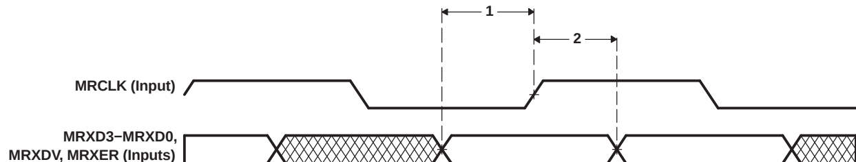
Figure 6-52. EMAC Receive Interface Timing
