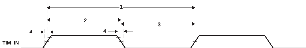
Figure 6-56. Timer Timing
