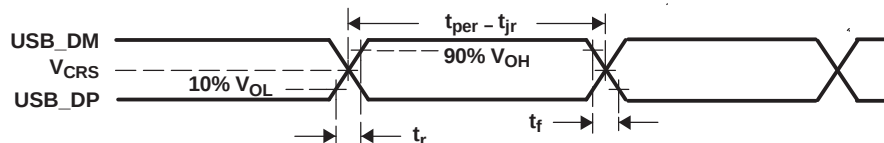
Figure 6-41. USB2.0 Integrated Transceiver Interface Timing
