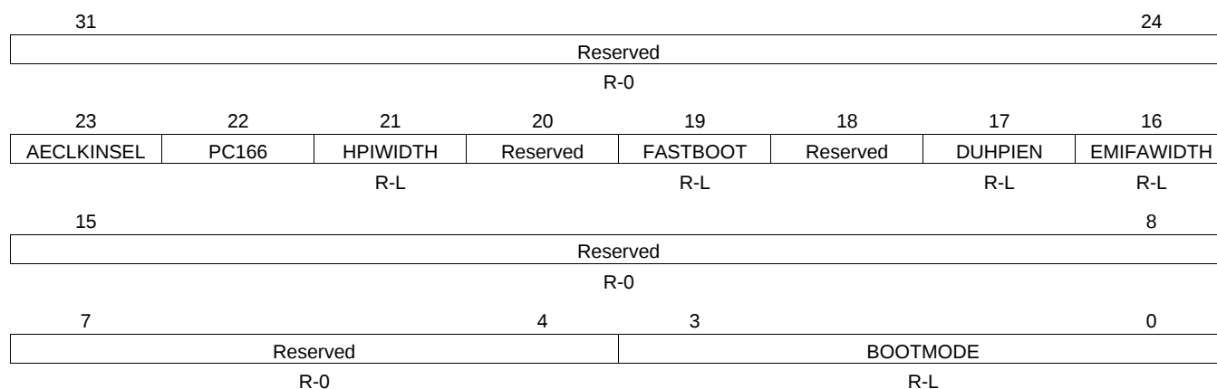
Figure 3-1. BOOTCFG Register
