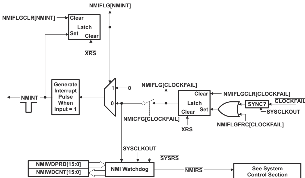
8-10. NMI-watchdog
