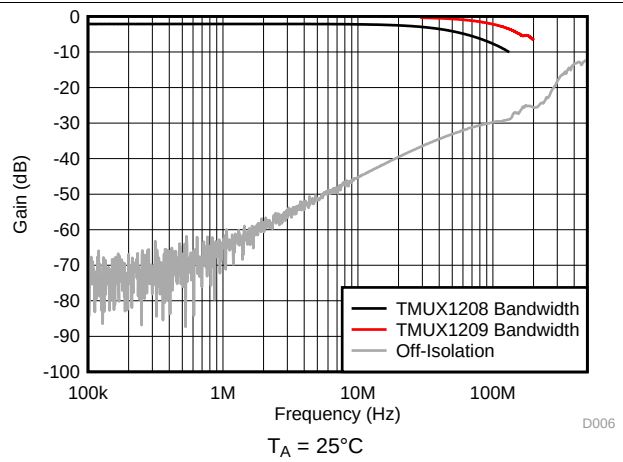
图 6. Frequency Response
