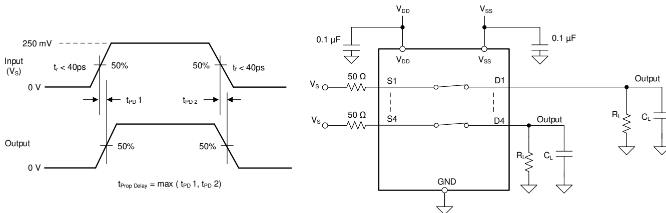
7-6. Propagation Delay Measurement Setup
