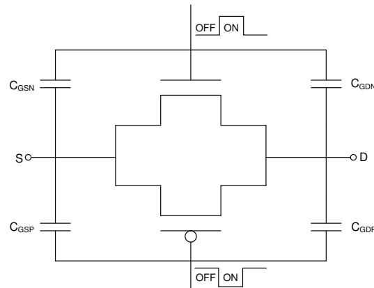
✎ 8-1. Transmission Gate Topology
