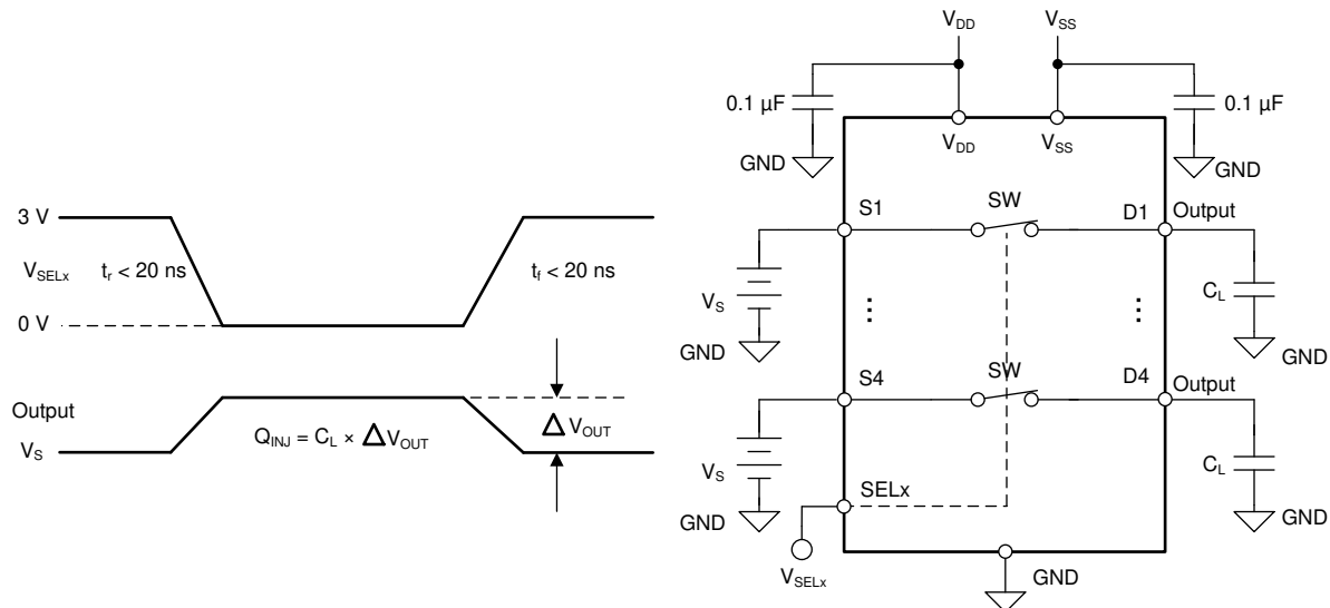
Figure 8-5. Charge-Injection Measurement Setup
