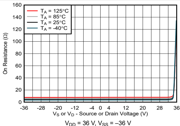
FIG 7-1. On-Resistance vs Source or Drain Voltage
