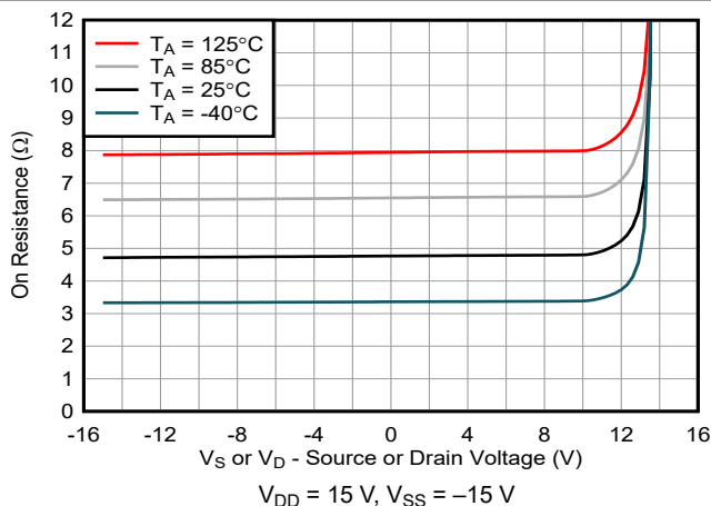
FIG 7-5. On-Resistance vs Source or Drain Voltage
