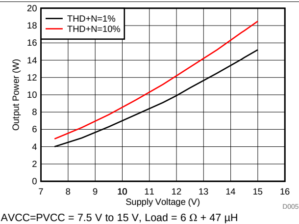
图 5. Output Power vs Supply Voltage (BTL)
