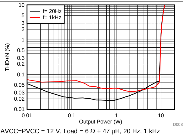
图 3. THD+N vs Output Power (BTL)
