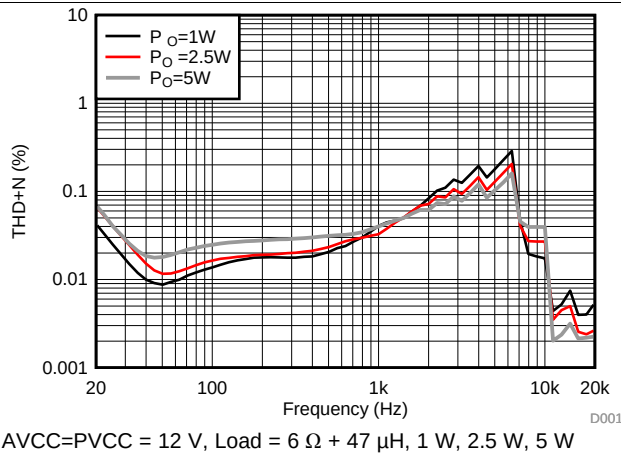
图 1. THD+N vs Frequency (BTL)
