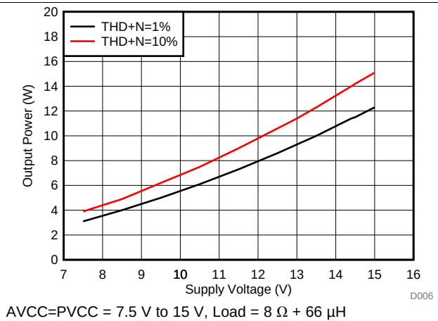
图 6. Output Power vs Supply Voltage (BTL)
