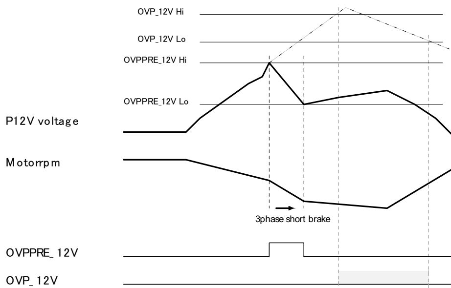
Figure 9. OVPPRE_12V
