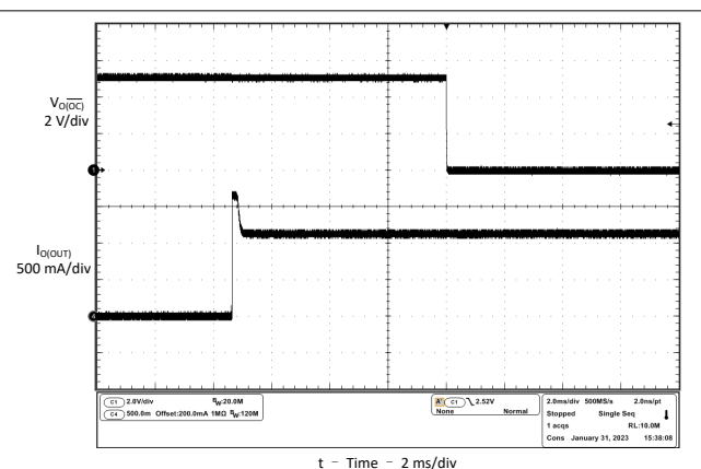
図 6-44. 3-Ω Load Connected to Enabled Device
