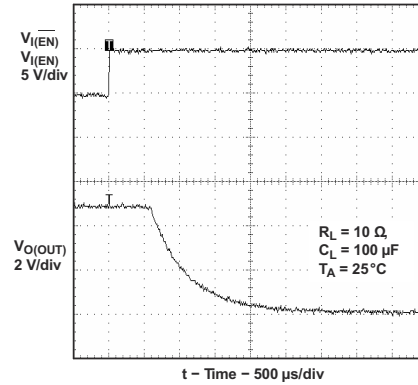
図 6-20. Turnoff Delay and Fall Time With 100-μF Load
