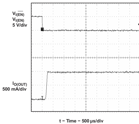
図 6-21. Short-Circuit Current, Device Enabled Into Short
