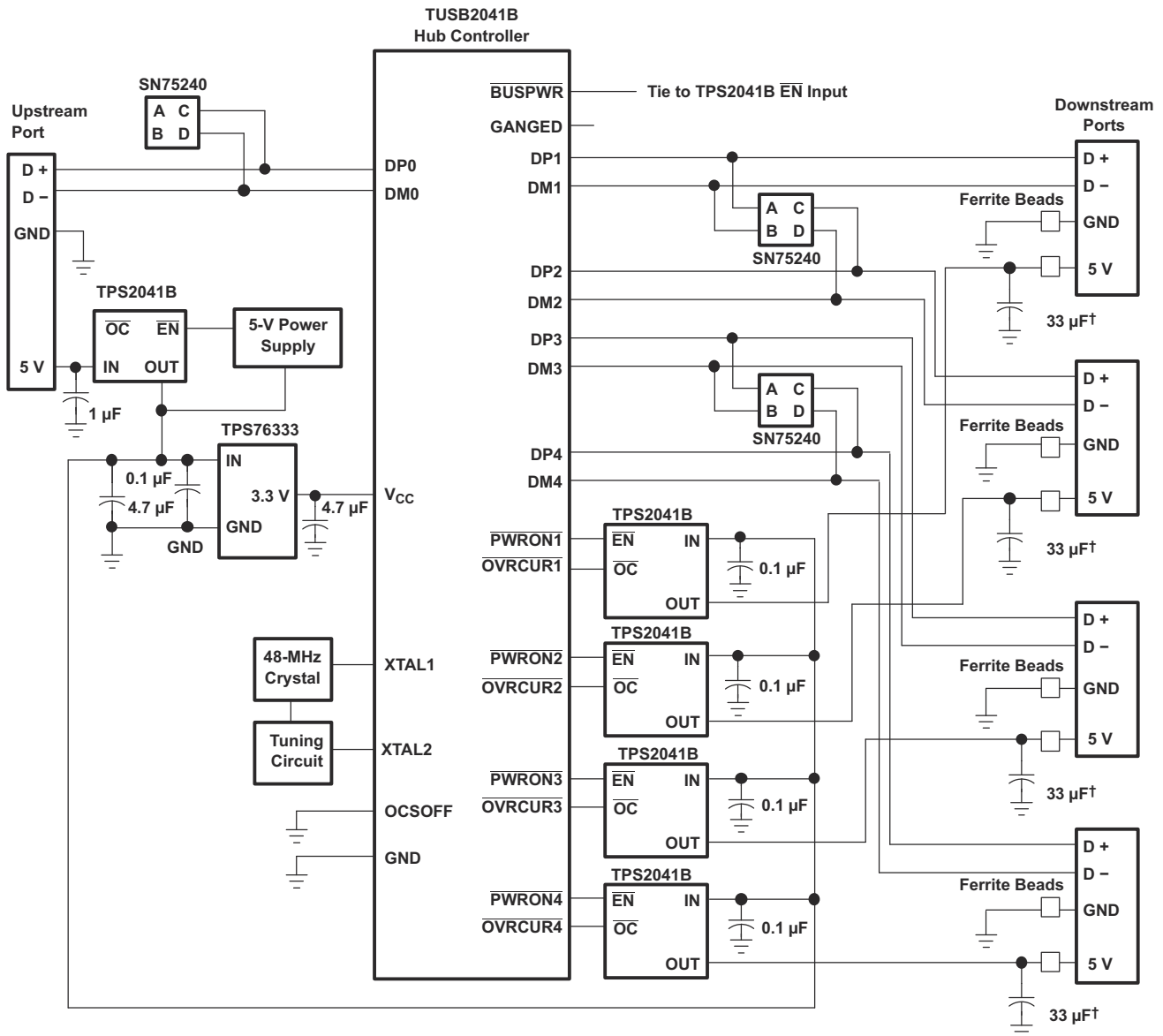
9-13. Hybrid Self and Bus-Powered Hub Implementation, TPS2041B and TPS2051B
