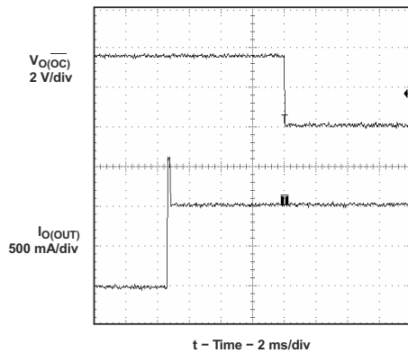
図 6-23. 3-Ω Load Connected to Enabled Device
