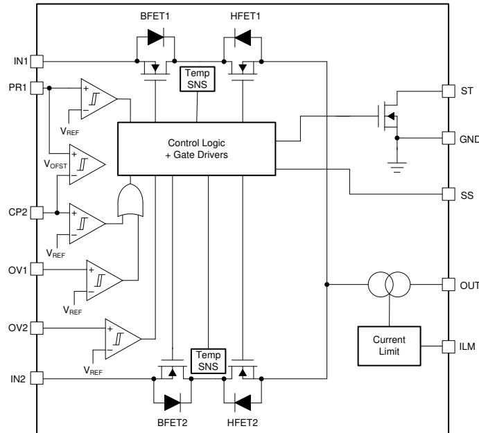
Figure 9-2. TPS2121 Functional Block Diagram
