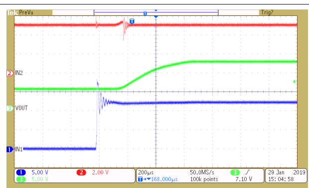
FIG 10-22. TPS2121 Hotplug Event with TVS1800
