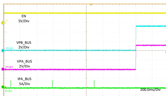
11-24. Short Circuit Recovery
