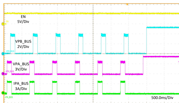
11-26. 1- \Omega Load Recovery
