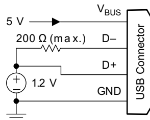
Figure 10-24. 1.2-V Mode
