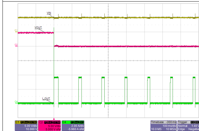
TPS259251/61, V_{IN} = 5\text{ V}
