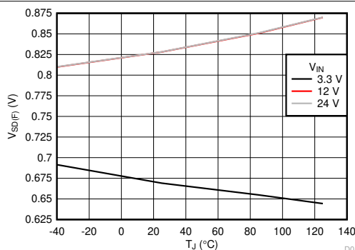
7-7. EN/UVLO Falling Threshold for Lowest Current Consumption
