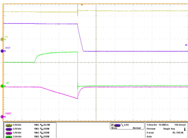
A. R_{ILIM} = 182 \, \Omega C_{ITIMER} = 4.7 \, \text{nF}
