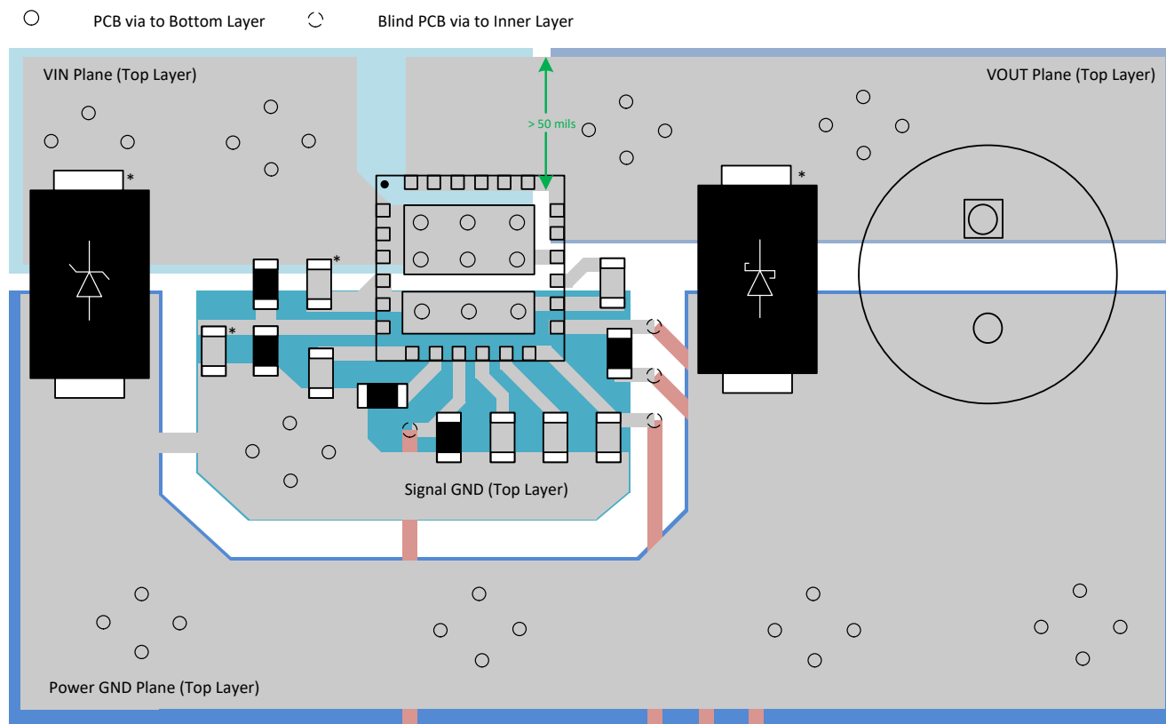
11-1. TPS25980 Example PCB Layout
