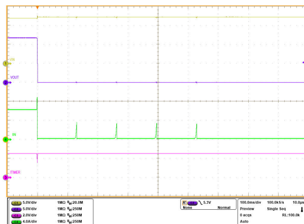
A. R_{ILIM} = \text{TBD } \Omega C_{ITIMER} = 4.7 \text{ nF} C_{RETRY\_DLY} = 2.2 \text{ nF} , C_{NRETRY} = 2.2 \text{ nF}
