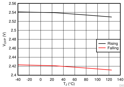
7-1. Supply UVP Threshold vs Temperature
