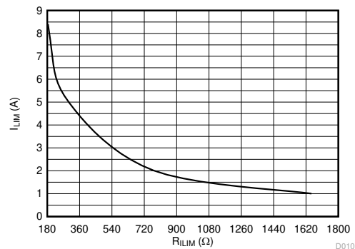
7-10. Output Current Limit ( I_{LIM} ) vs R_{ILIM}
