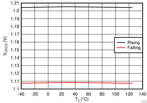
7-5. EN/UVLO Threshold vs Temperature
