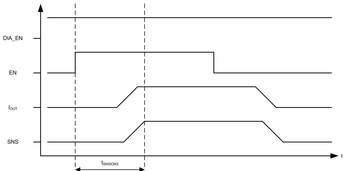
FIG 9-10. Current Sensing in Low-Duty Cycle Applications
