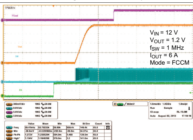
Figure 22. FCCM Start-Up
