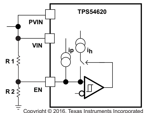
Figure 19. Adjustable VIN and PVIN Undervoltage Lockout
