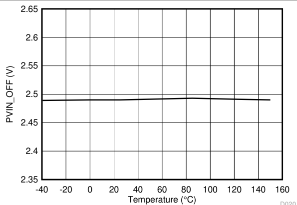
6-14. Turnoff Voltage vs Junction Temperature
