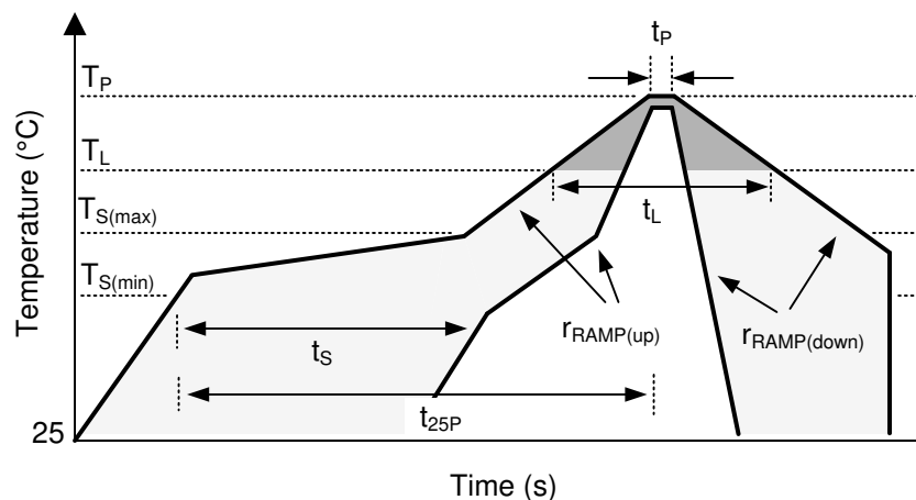
图 10-2. Recommended Reflow-Oven Thermal Profile
