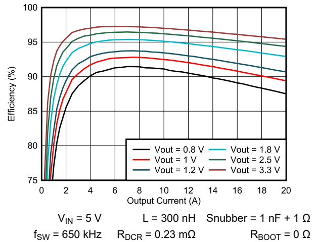
Figure 6-2. TPS546B24A Efficiency vs Output Current
