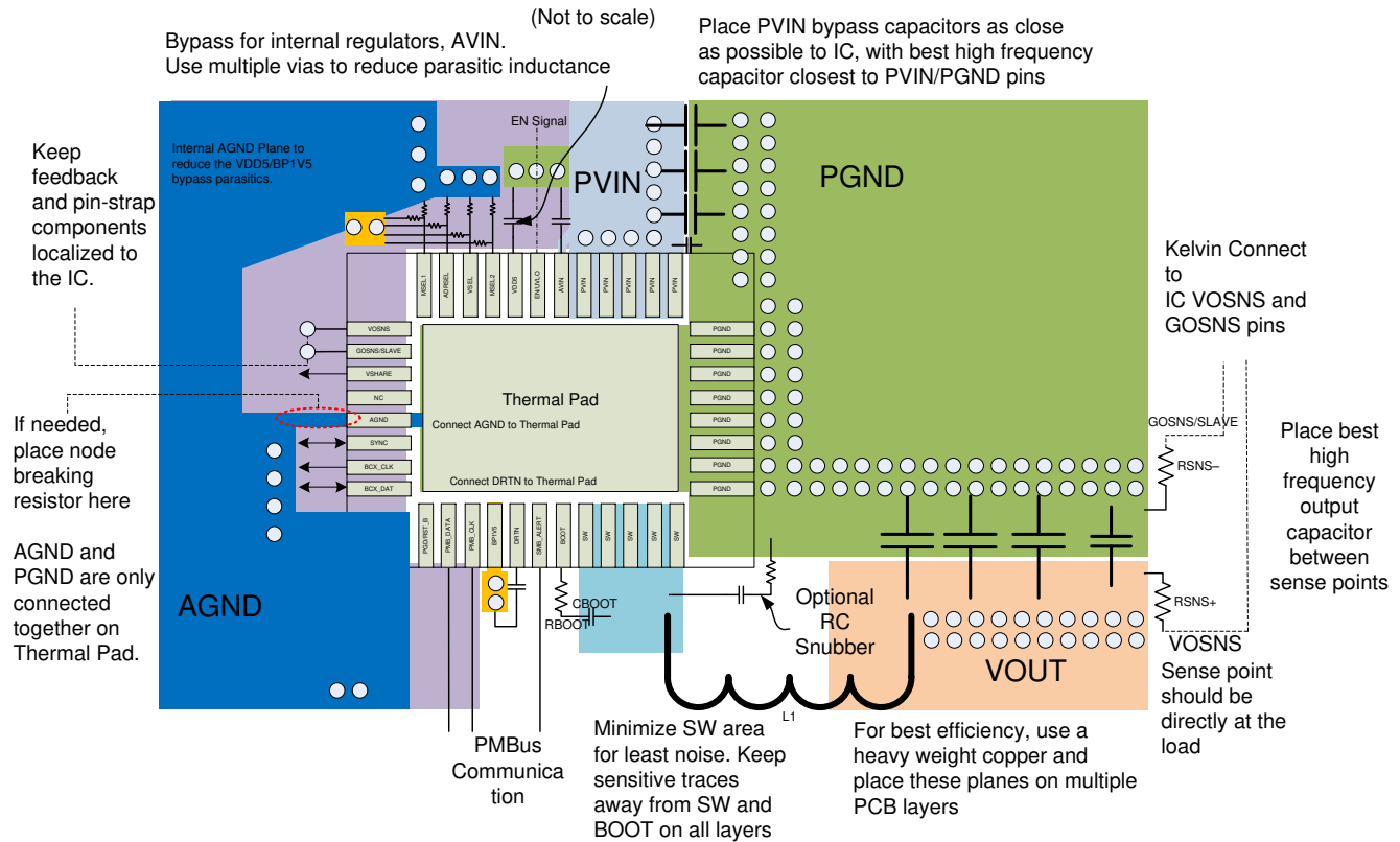
图 10-1. PCB Layout Recommendation
