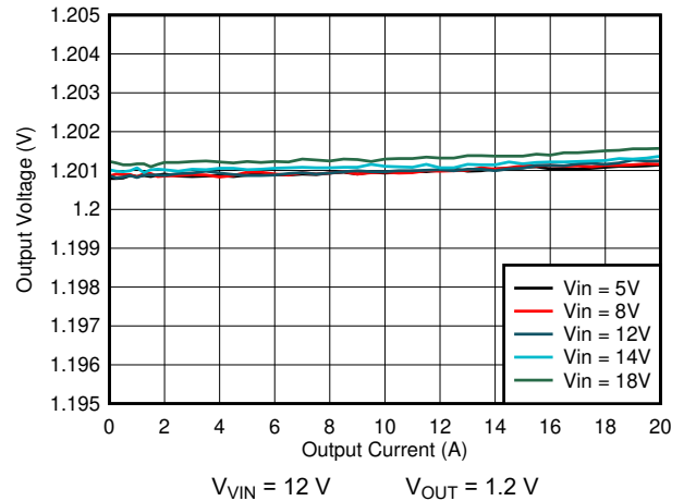
8-3. Load Regulation
