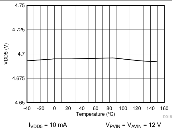
6-11. VDD5 Voltage vs Junction Temperature
