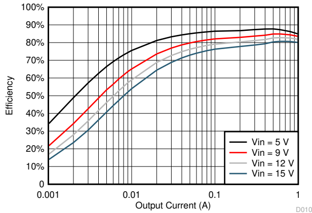
Figure 6-9. TPS561201 V_{OUT} = 1.05 \text{ V} , Efficiency, L = 2.2 \mu\text{H}
