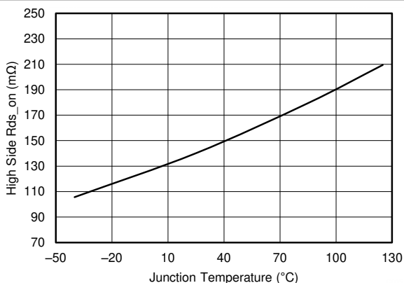
6-5. High-Side R_{ds-on} vs Junction Temperature
