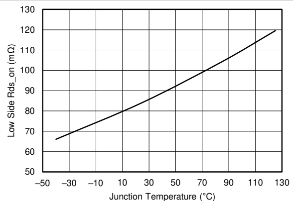
6-6. Low-Side R_{ds-on} vs Junction Temperature
