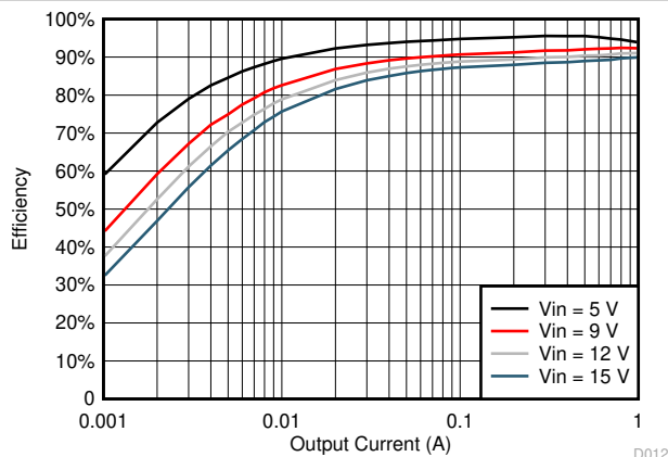
Figure 6-11. TPS561201 V_{OUT} = 3.3 \text{ V} , Efficiency, L = 3.3 \mu\text{H}
