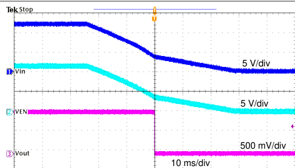
8-16. TPS561201 Shutdown Relative to V_I
