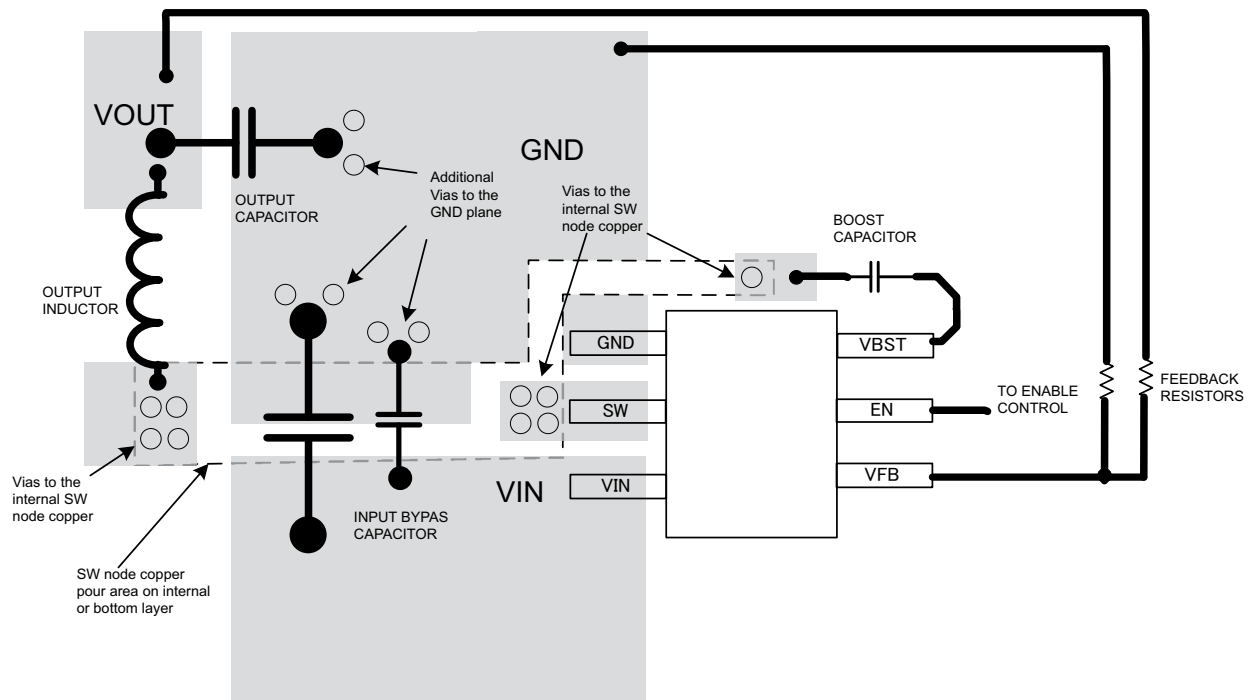
10-1. TPS561201 and TPS561208 Layout
