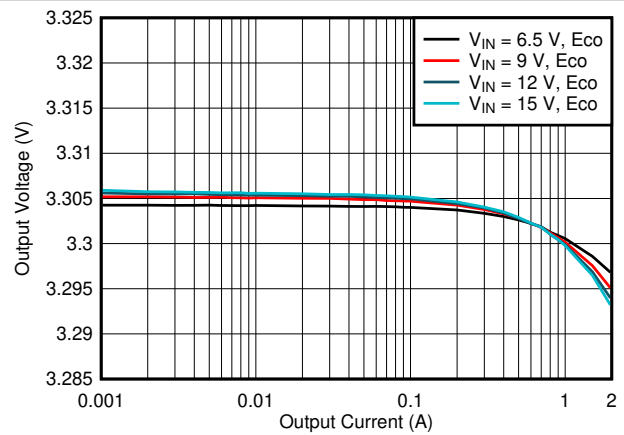
8-3. Load Regulation
