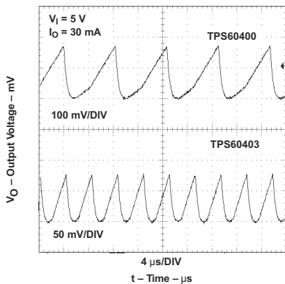
9-2. Output Voltage vs Time for TPS60400 and TPS60403
