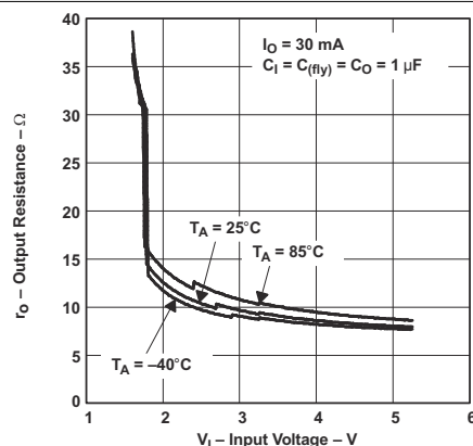
☒ 7-10. Output Resistance vs Input Voltage
