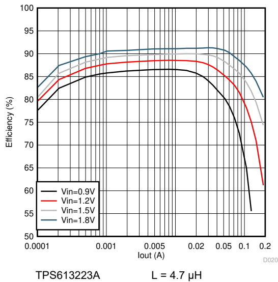
図 6-9. Load Efficiency with Different Inputs
