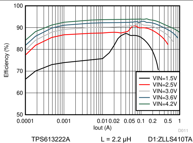
図 8-18. Efficiency with Different Input Voltage
