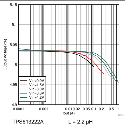
6-6. Load Regulation
