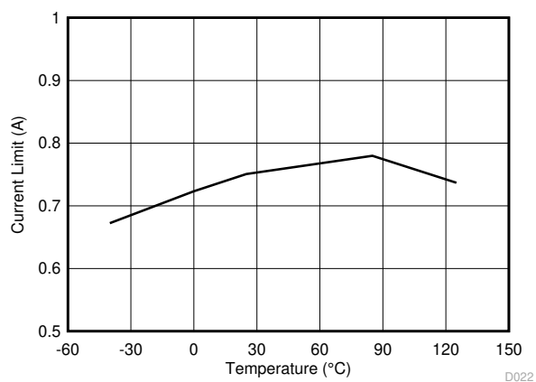
図 6-14. Current Limit with Different Temperature
