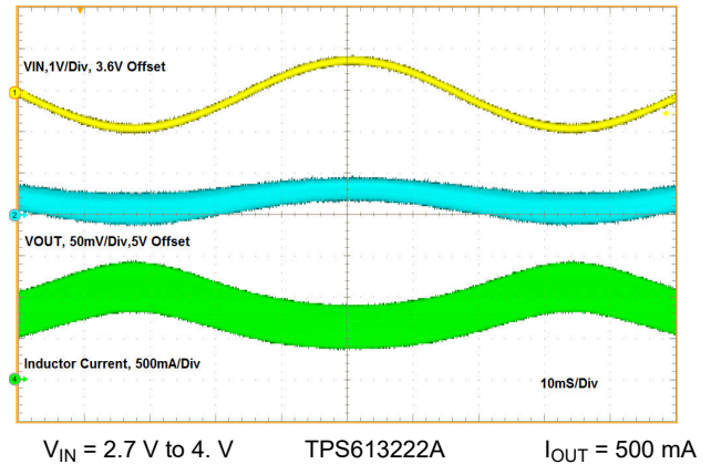
図 8-15. Line Regulation
