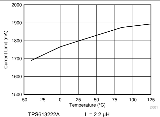
図 6-12. Current Limit with Different Temperature
