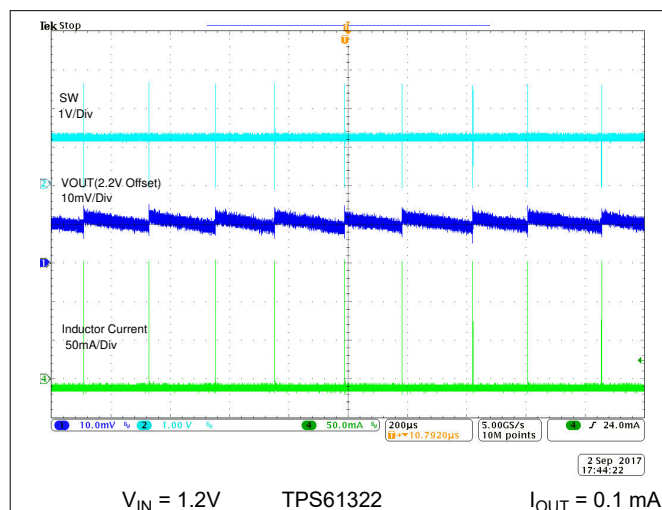
図 8-2. Switching Waveform at Light Load
