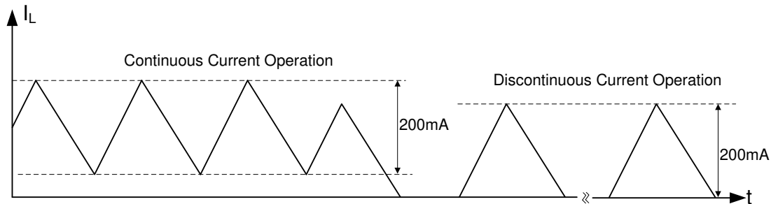
図 7-1. Hysteretic Current Operation
