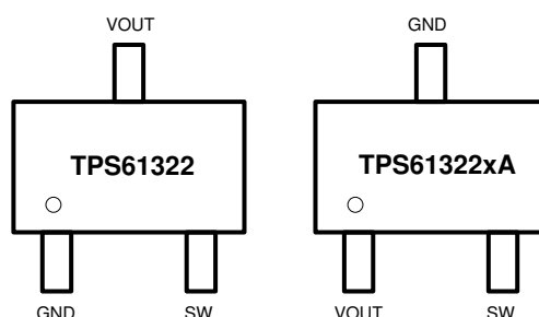
図 5-1. DBZ Package 3-Pin SOT Top View
