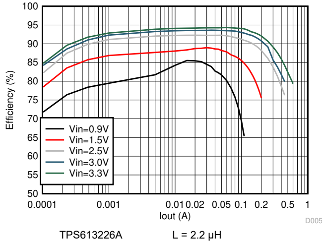
図 6-7. Load Efficiency with Different Inputs
