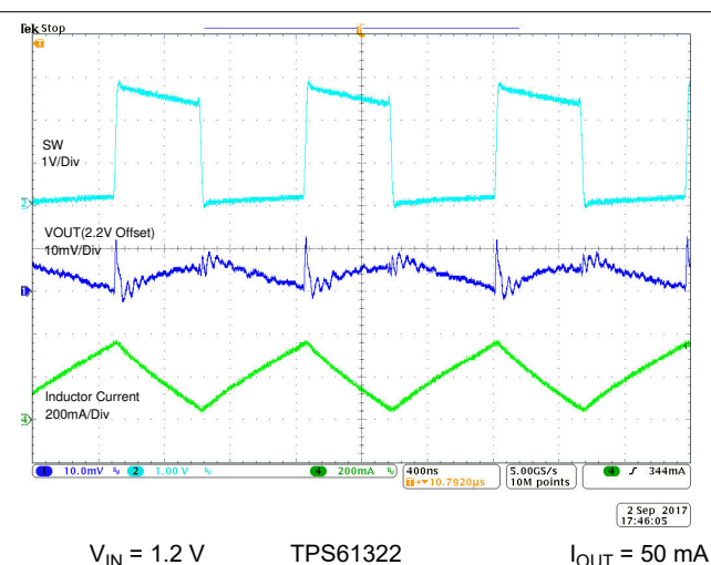
図 8-3. Switching Waveform at Heavy Load
