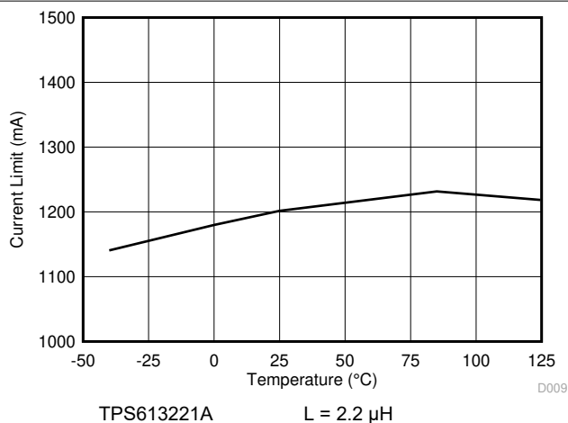
図 6-11. Current Limit with Different Temperature
