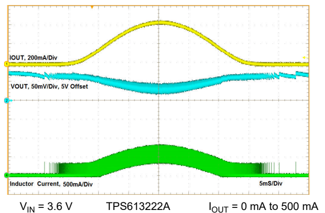
図 8-17. Load Regulation
