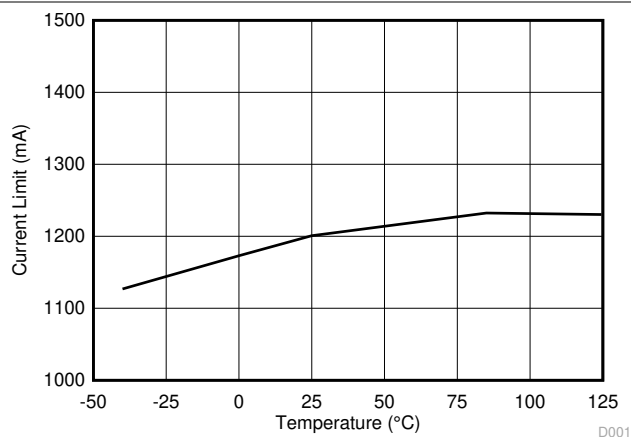
図 6-13. Current Limit with Different Temperature
