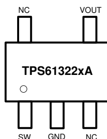
図 5-2. DBV Package 5-Pin SOT Top View
