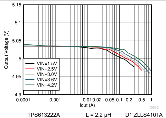
図 8-19. Load Regulation
