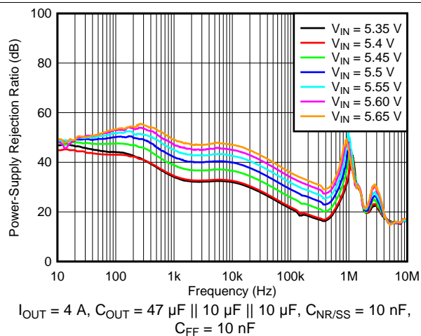
Figure 9. PSRR vs Frequency and V_{IN} for V_{OUT} = 5.0\text{ V}
