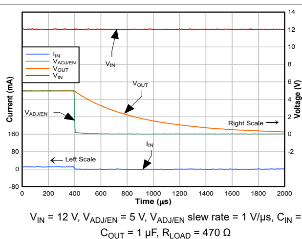
8-3. Power-Down
