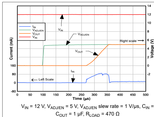
8-2. Power-Up
