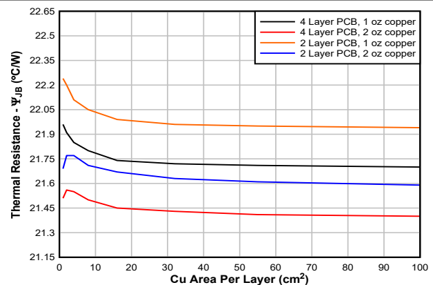
Figure 8-9. \psi_{JB} vs Copper Area (DYB Package)
