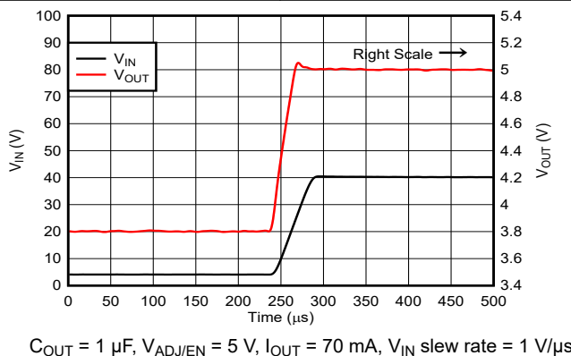
8-4. Dropout Exit Recovery
