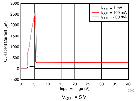
FIG 6-2. Quiescent Current vs Input Voltage
