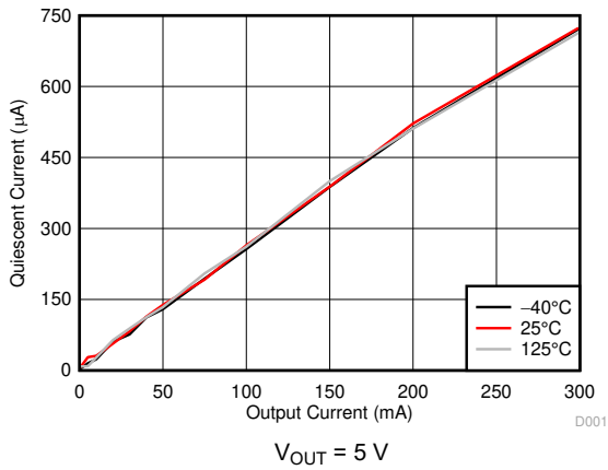
FIG 6-1. Quiescent Current vs Output Current
