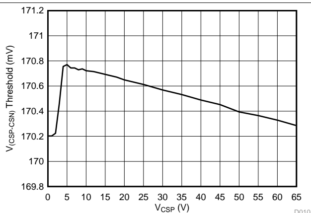
Figure 11. V_{(CSP-CSN)} Threshold vs V_{CSP} Voltage
