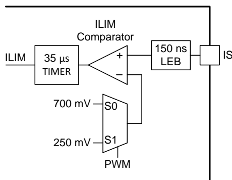
Figure 25. Switch Current Limit Circuit
