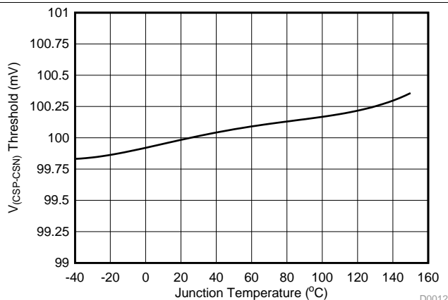
Figure 13. V_{(CSP-CSN)} Threshold vs Junction Temperature
