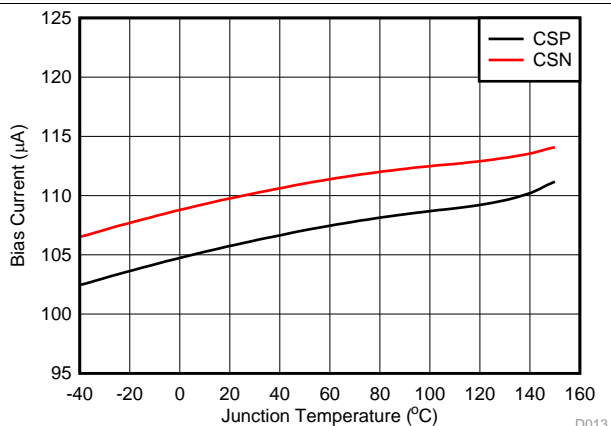
Figure 14. CSP/CSN Input Bias Current vs Junction Temperature
