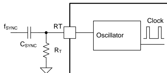
Figure 21. Oscillator Synchronization Through AC Coupling
