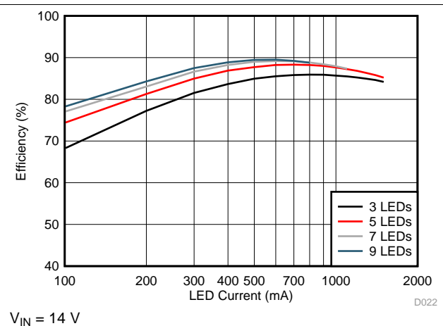
Figure 56. Efficiency
