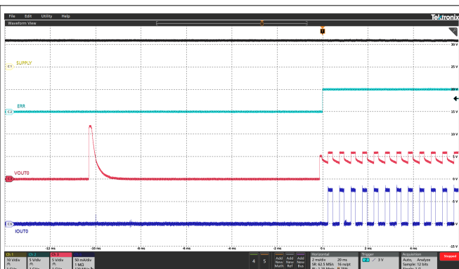
7-26. LED Open-Circuit Recovery In FS Mode
