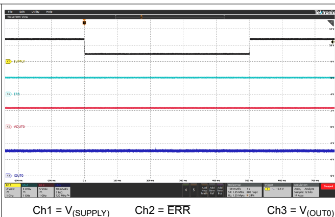
7-14. Transient Undervoltage
