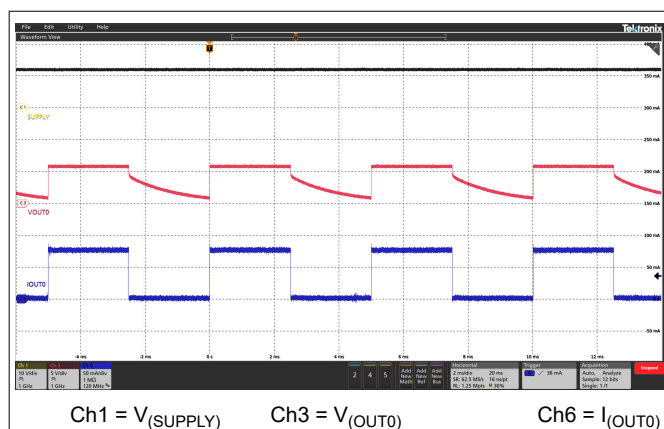
7-11. PWM Dimming at 200 Hz
