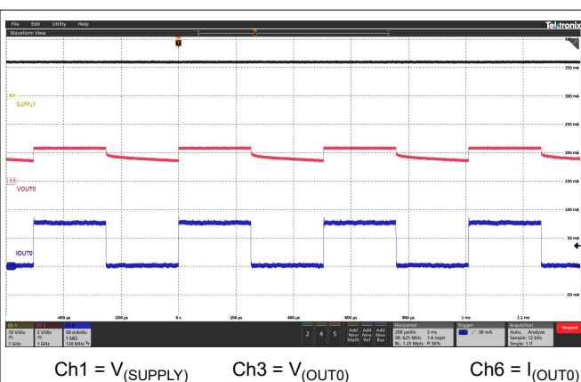
7-12. PWM Dimming at 2000 Hz
