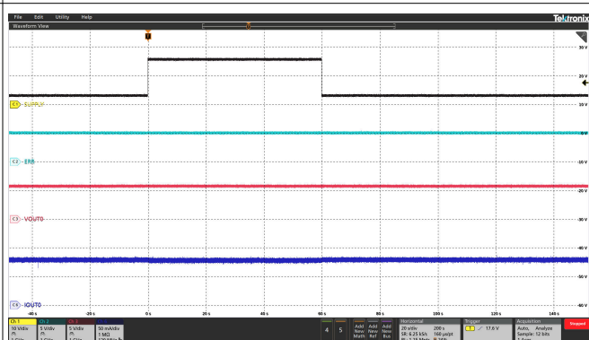
7-14. Transient Undervoltage
