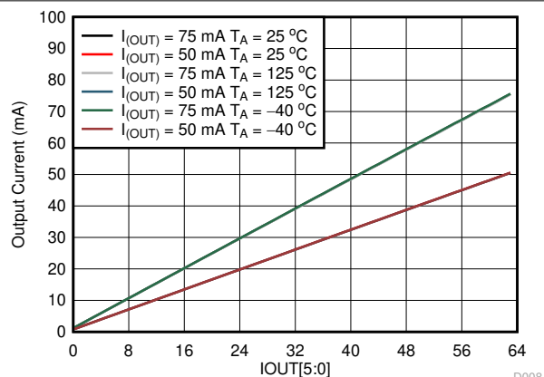
7-8. Output DC Current vs IOUT[5:0]
