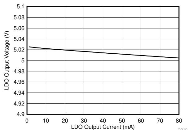
7-10. LDO Output Load Regulation
