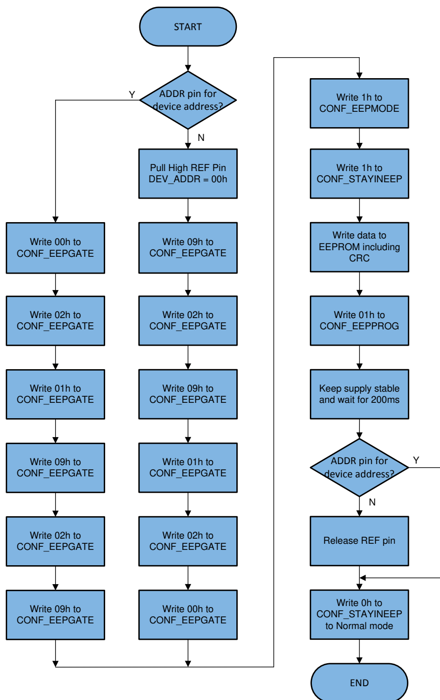
8-18. Programming Sequence
