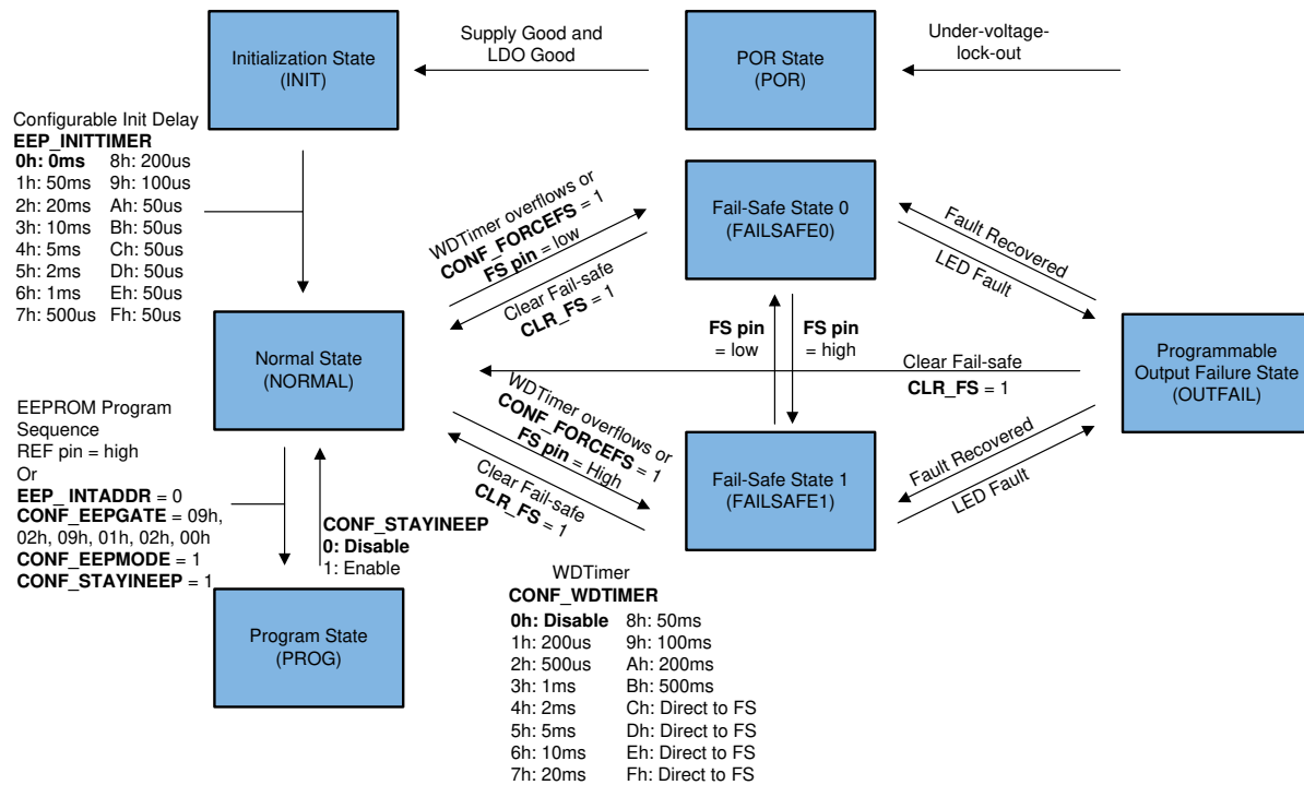
图 8-8. Device Functional Mode State Machine
