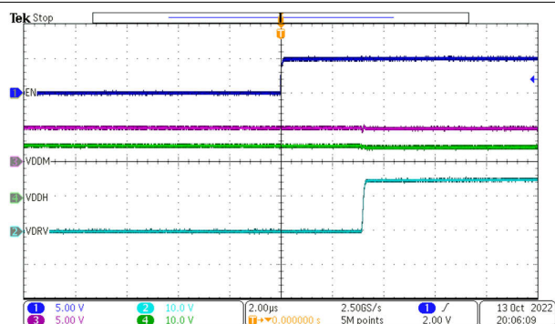
図 9-7. Three-Wire Mode, f_{EN} = 10\text{ kHz} , TPSI3052
