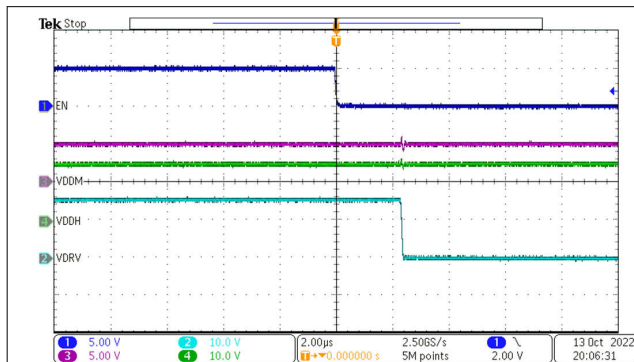
Three-wire mode VDDP = 5.0 V R_{PXFR} = 14.7 \text{ k}\Omega C_{DIV1} = 330 \text{ nF} C_{DIV2} = 1 \mu\text{F} I_{AUX} = 4 \text{ mA} C_{VDRV} = 6.8 \text{ nF} T_A = 25^\circ\text{C} FIG 9-10. t_{HL\_VDRV} , Three-Wire Mode, TPSI3052
