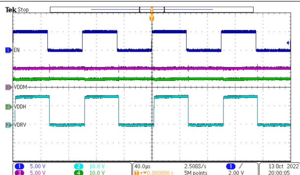
図 9-5. t_{LH\_VDRV} , Three-Wire Mode, TPSI3052
