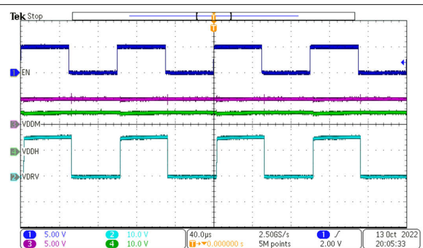
Three-wire mode VDDP = 5.0 V R_{PXFR} = 14.7 \text{ k}\Omega C_{DIV1} = 330 \text{ nF} C_{DIV2} = 1 \mu\text{F} I_{AUX} = 4 \text{ mA} C_{VDRV} = 6.8 \text{ nF} T_A = 25^\circ\text{C} FIG 9-11. Three-Wire Mode, f_{EN} = 10 \text{ kHz} , TPSI3052
