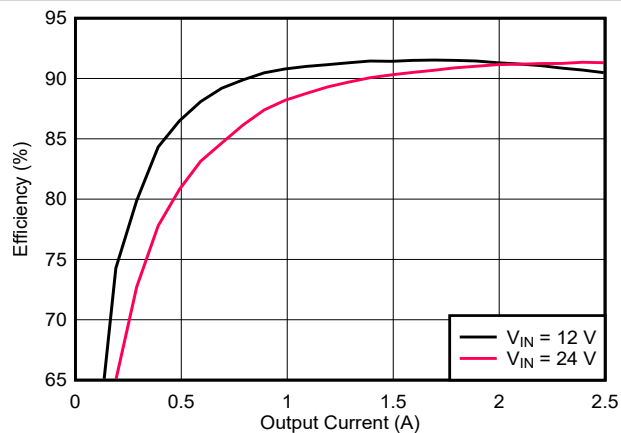
Figure 9-14. Efficiency
