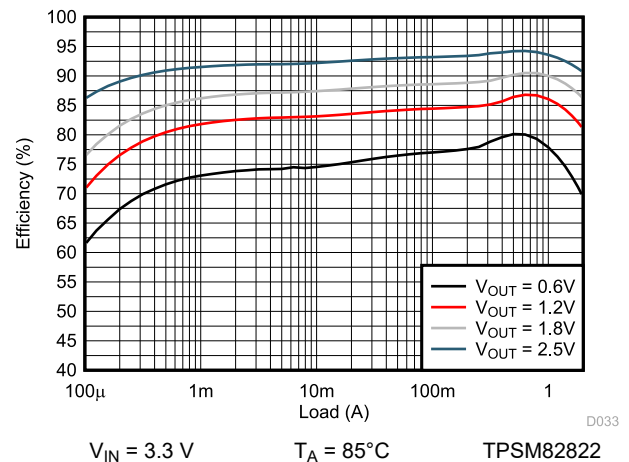
9-58. Efficiency
