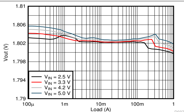
9-18. Load Regulation
