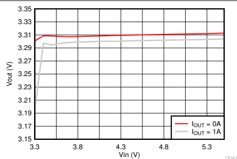
图 9-22. Line Regulation
