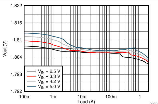
9-66. Load Regulation
