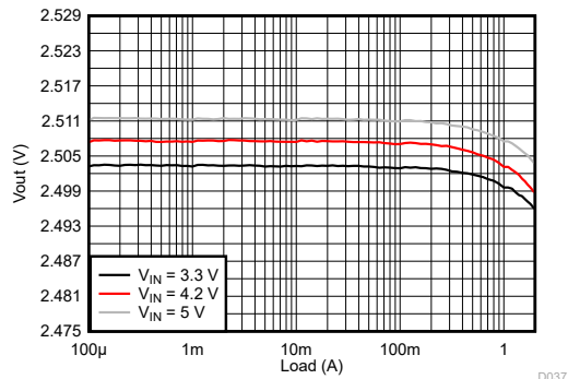
9-100. Load Regulation
