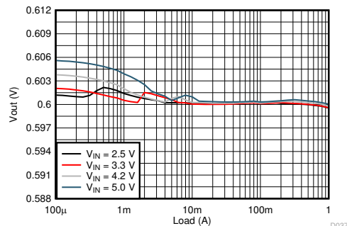
9-16. Load Regulation
