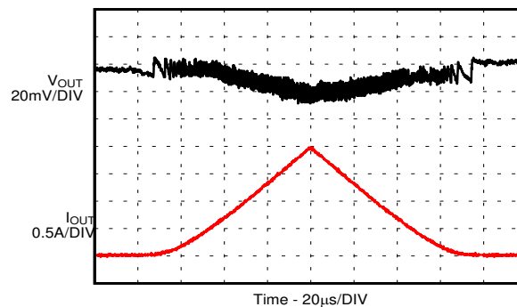
9-78. Load Sweep
