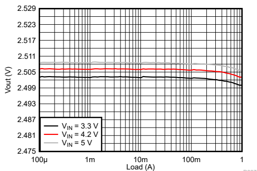
9-43. Load Regulation
