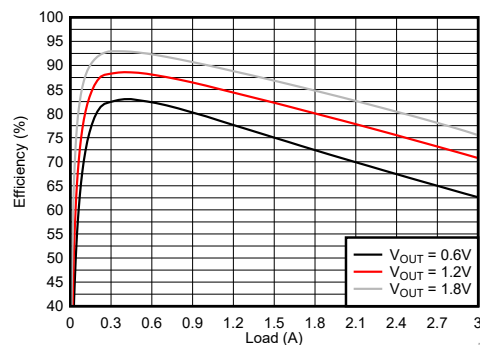
图 9-144. Efficiency
