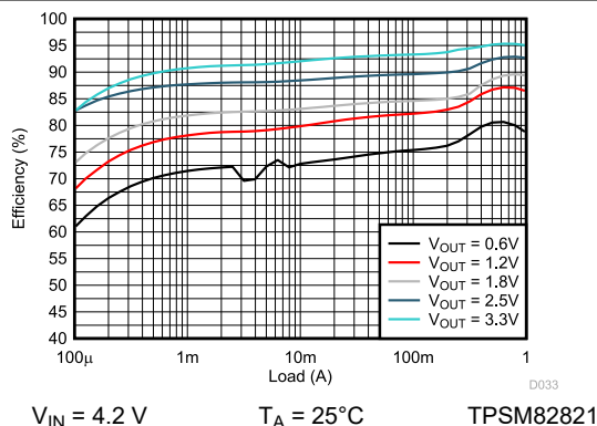
图 9-5. Efficiency
