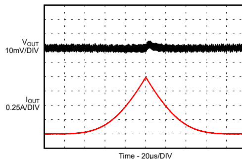
9-48. Load Sweep
