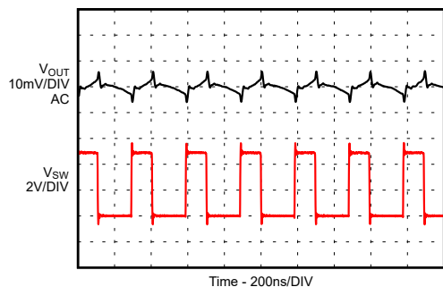
9-47. Output Ripple in PWM Mode
