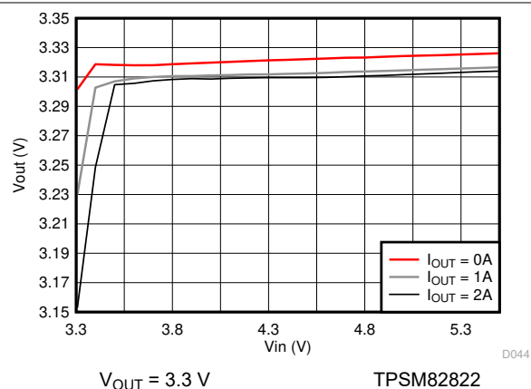
9-75. Line Regulation
