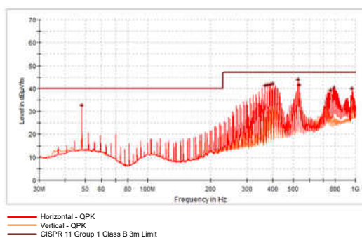
9-136. TPSM82823 Radiated Emissions
