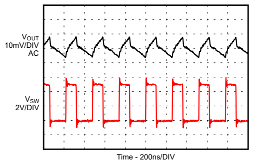
9-128. Output Ripple in PWM Mode
