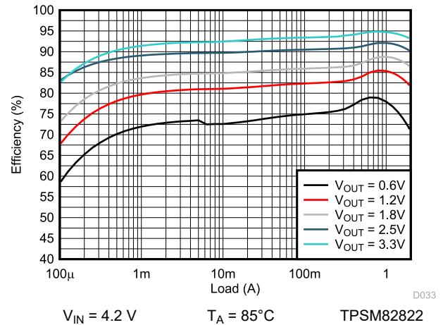
9-56. Efficiency
