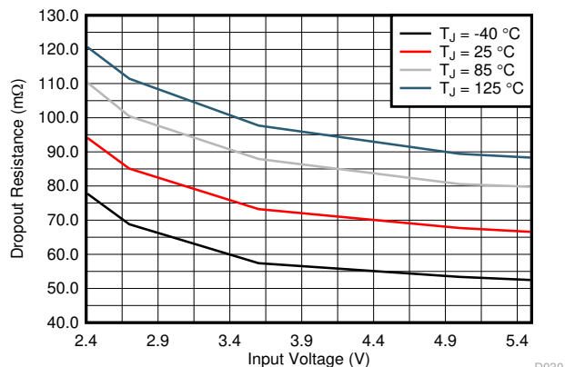
FIG 7-2. TPSM82822/TPSM82822A Dropout Resistance
