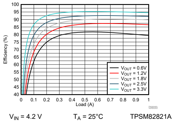
Figure 9-31. Efficiency
