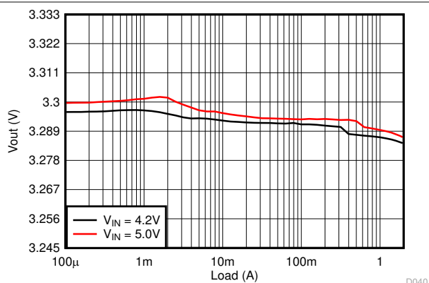
9-68. Load Regulation
