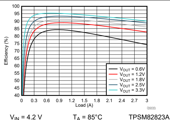
图 9-140. Efficiency
