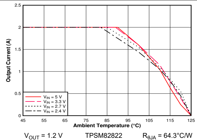
9-62. Safe Operating Area
