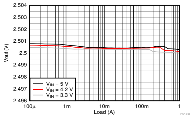
9-19. Load Regulation
