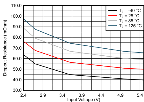
FIG 7-3. TPSM82823/TPSM82823A Dropout Resistance
