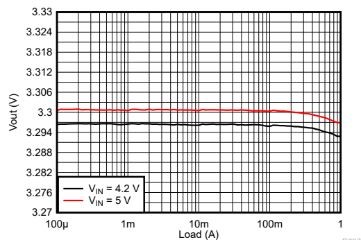
9-44. Load Regulation
