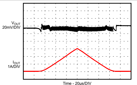
9-130. Load Sweep
