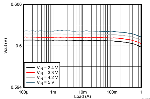
9-42. Load Regulation
