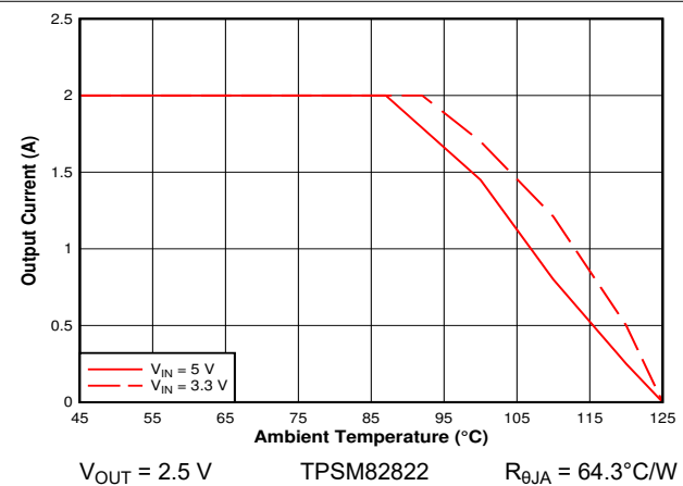
9-64. Safe Operating Area
