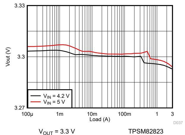
9-127. Load Regulation
