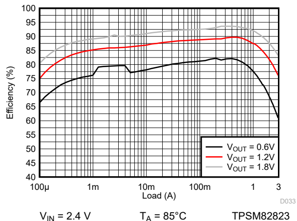
图 9-117. Efficiency
