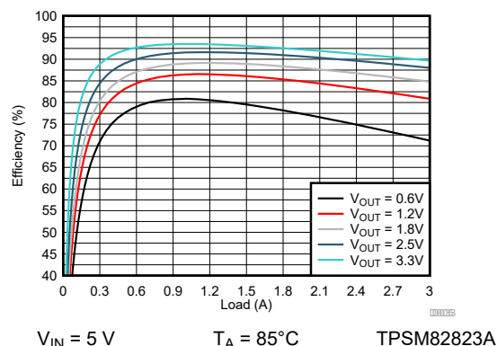
图 9-138. Efficiency
