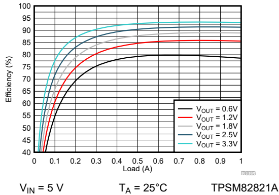
Figure 9-29. Efficiency
