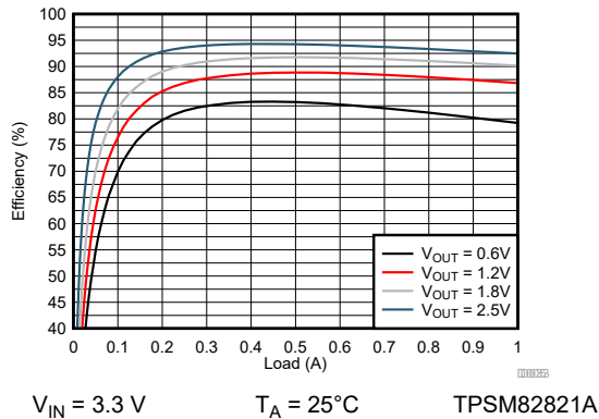
Figure 9-33. Efficiency
