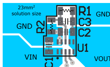
✎ 11-2. TPSM8282x/TPSM8282xA PCB Layout for the Adjustable Devices (BOM from Table 9-1 with 1 x 22-μF for C2)
