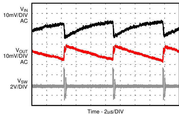
9-77. Input and Output Ripple in PSM Mode
