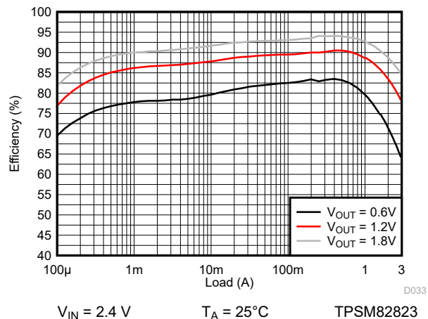
图 9-116. Efficiency
