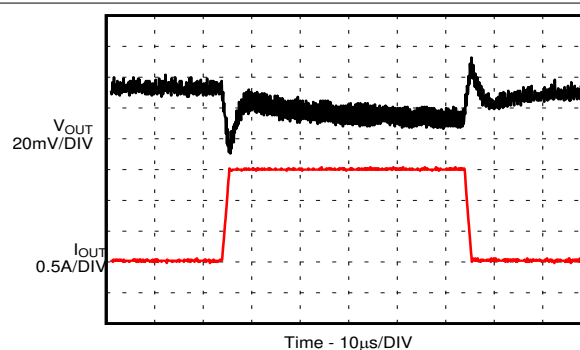
9-80. Load Transient
