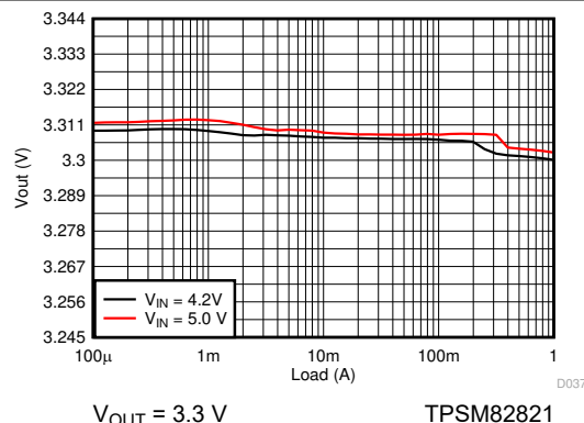
9-20. Load Regulation
