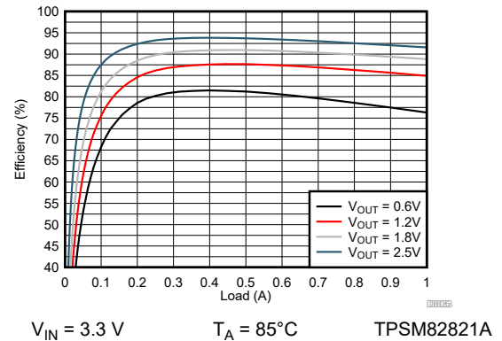
Figure 9-34. Efficiency
