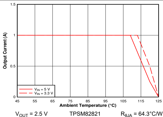
Figure 9-14. Safe Operating Area
