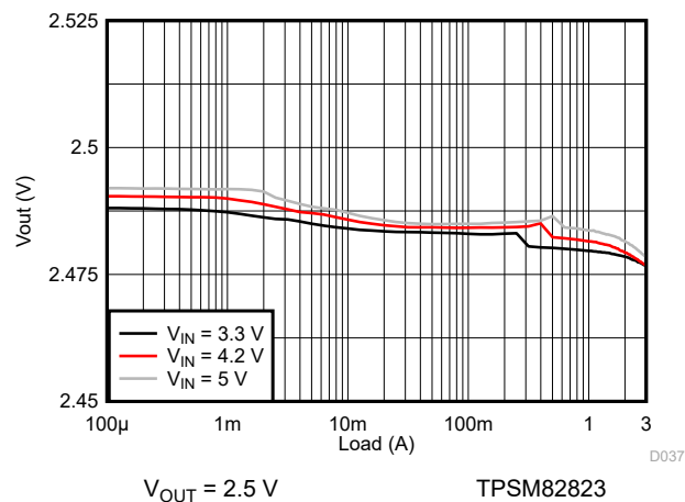
9-126. Load Regulation
