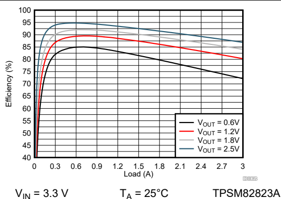
图 9-141. Efficiency
