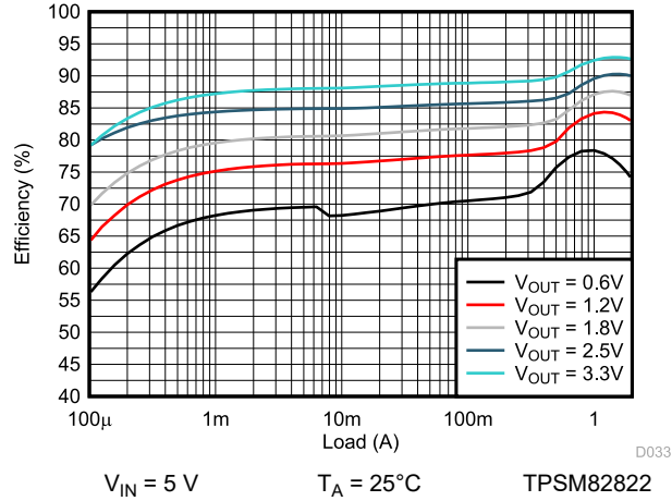
9-53. Efficiency
