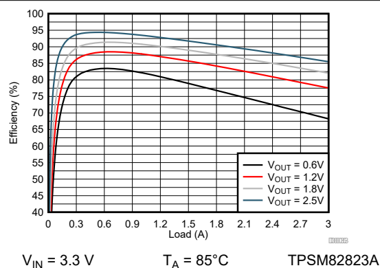
图 9-142. Efficiency
