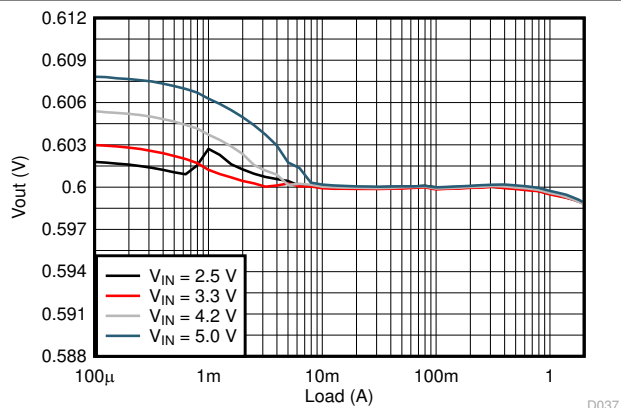
9-66. Load Regulation
