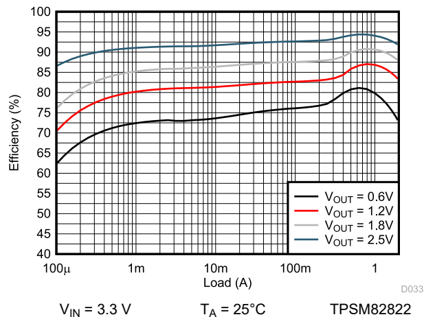
9-57. Efficiency
