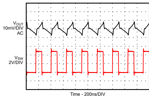
9-155. Output Ripple in PWM Mode
