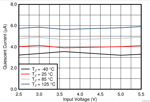
FIG 7-4. Quiescent Current
