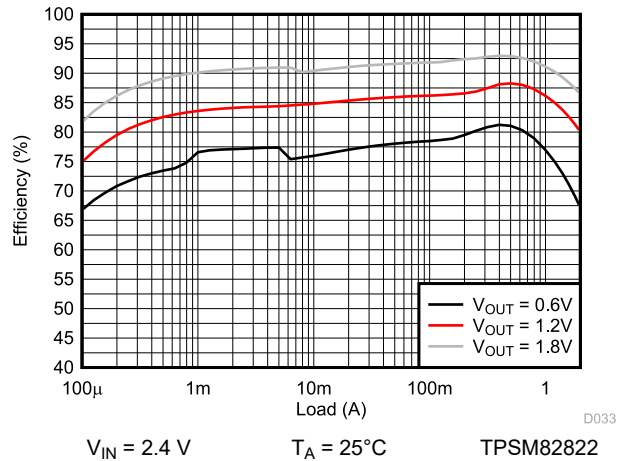
9-59. Efficiency
