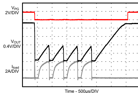
9-135. Short Circuit, HICcup Protection Entry / Exit
