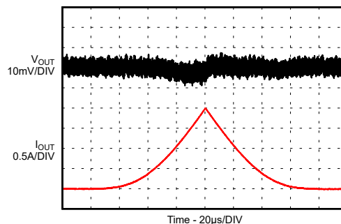
9-105. Load Sweep
