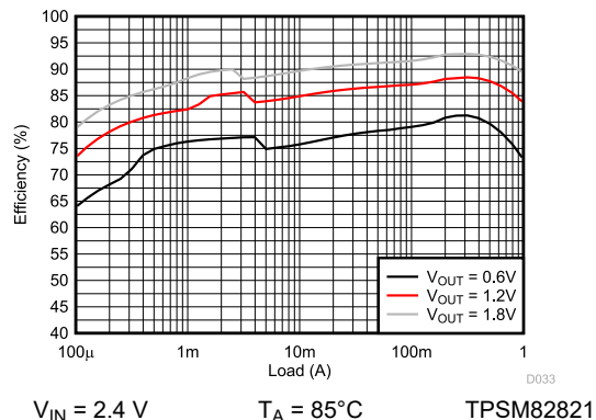
Figure 9-10. Efficiency
