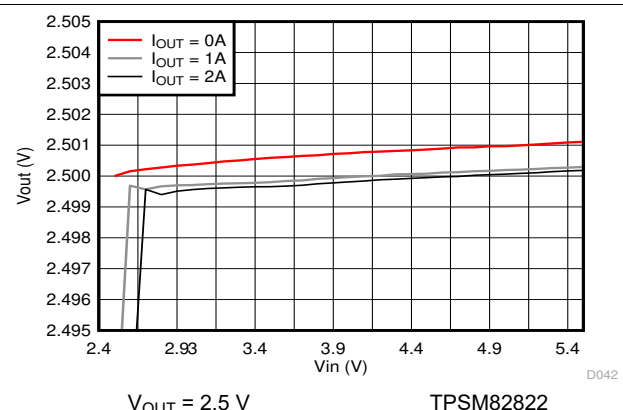
9-74. Line Regulation
