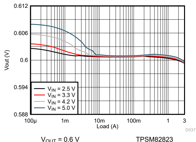
9-123. Load Regulation
