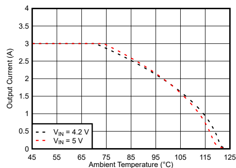
图 9-146. Safe Operating Area
