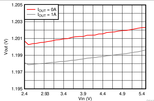
图 9-22. Line Regulation
