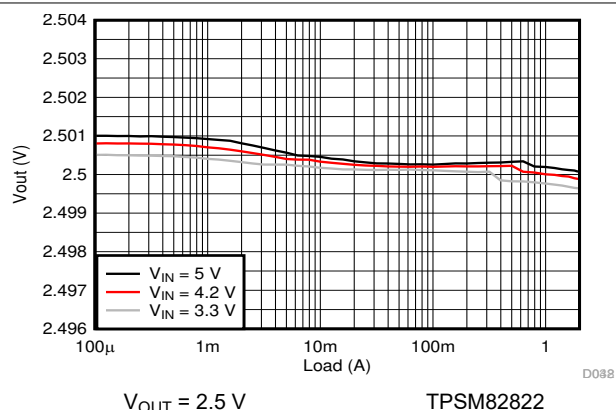
9-69. Load Regulation
