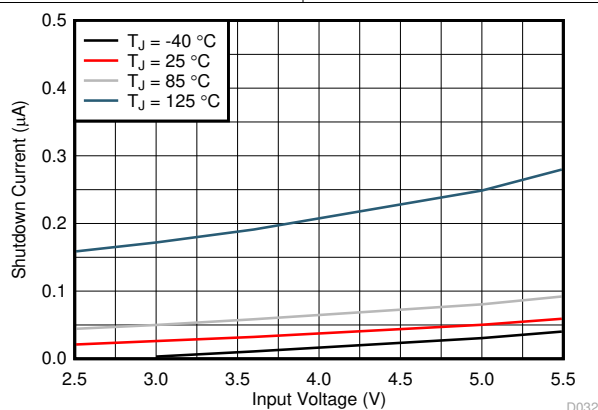
FIG 7-5. Shutdown Current
