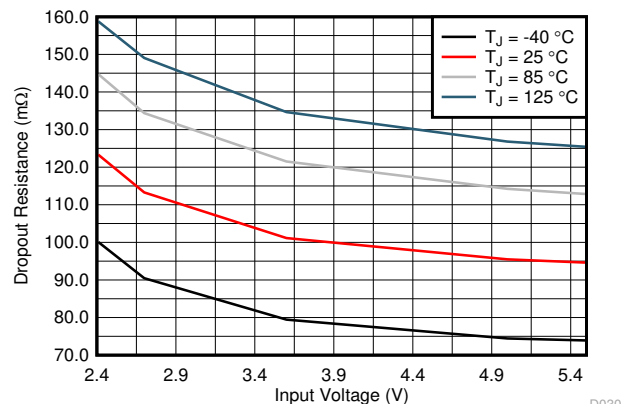
FIG 7-1. TPSM82821/TPSM82821A Dropout Resistance
