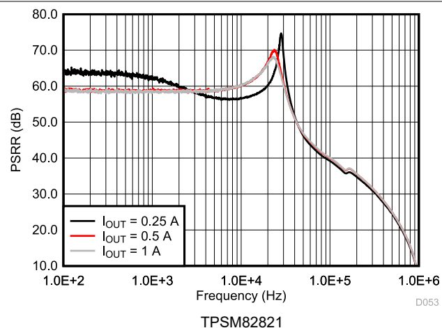
9-28. Power Supply Rejection Ratio (PSRR)
