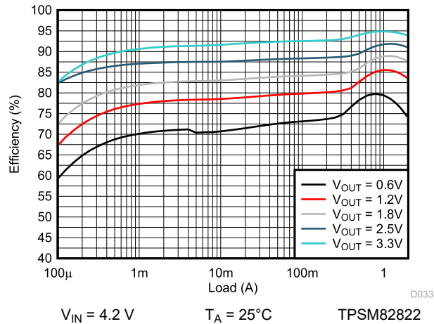
9-55. Efficiency
