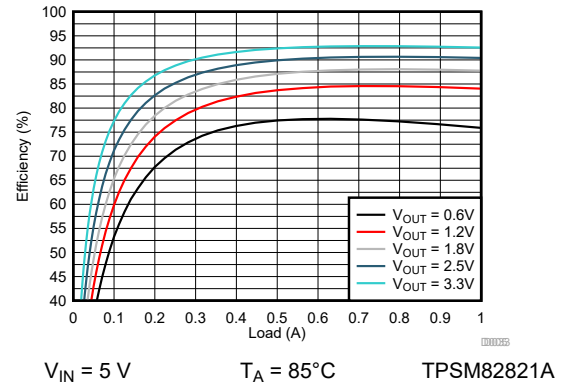
Figure 9-30. Efficiency
