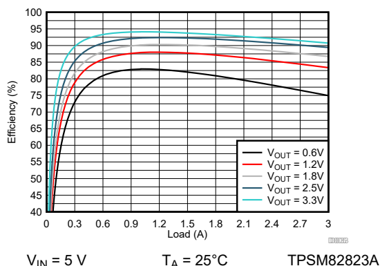
图 9-137. Efficiency
