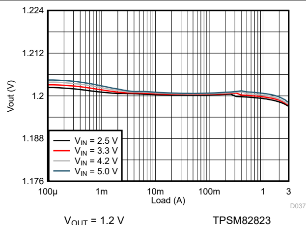
9-124. Load Regulation
