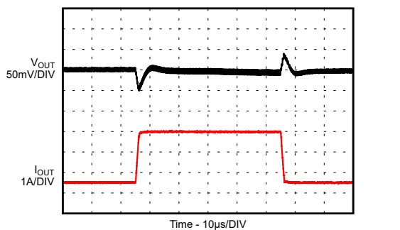
9-130. Load Sweep
