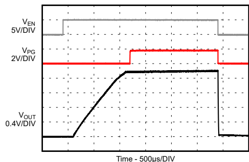
9-134. Start-up / Shutdown with Resistive Load
