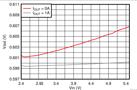
图 9-21. Line Regulation
