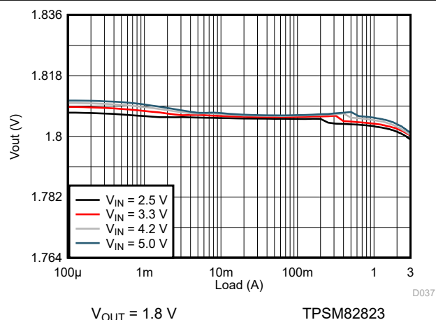
9-125. Load Regulation
