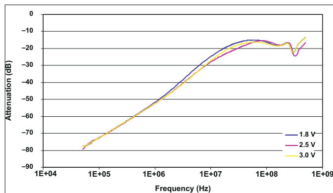
FIG 6-7. OFF Isolation
