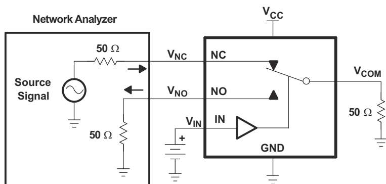
7-9. Crosstalk ( X_{TALK} )
