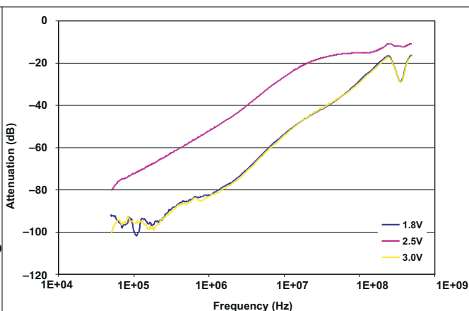
FIG 6-8. Crosstalk
