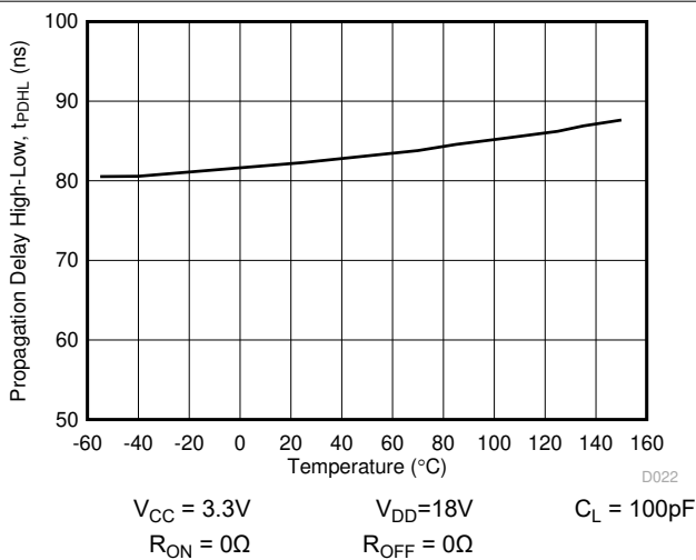
図 5-15. Propagation Delay t_{PDLH} vs. Temperature
