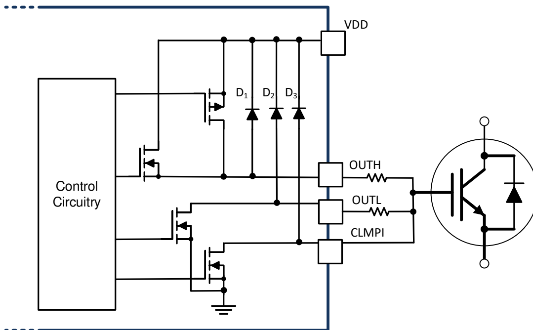
7-3. Short Circuit Clamping
