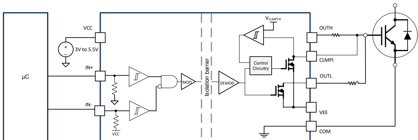
7-4. Active Miller Clamp
