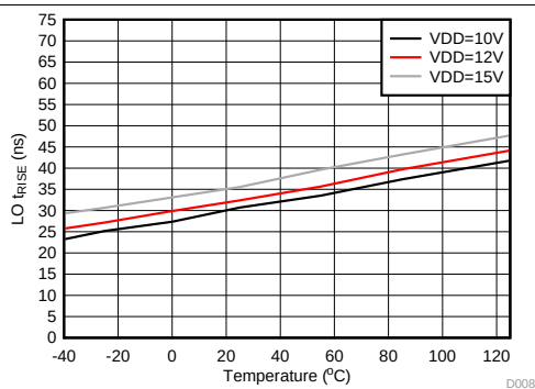
FIG 9. LO Rise Time with 1000-pF Load vs Temperature
