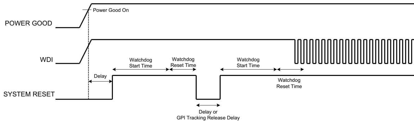
図 26. System Reset With Watchdog
