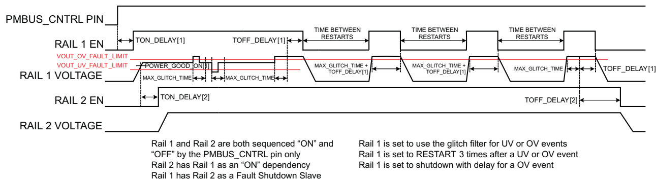
FIG 16. Sequencing and Fault-Response Timing
