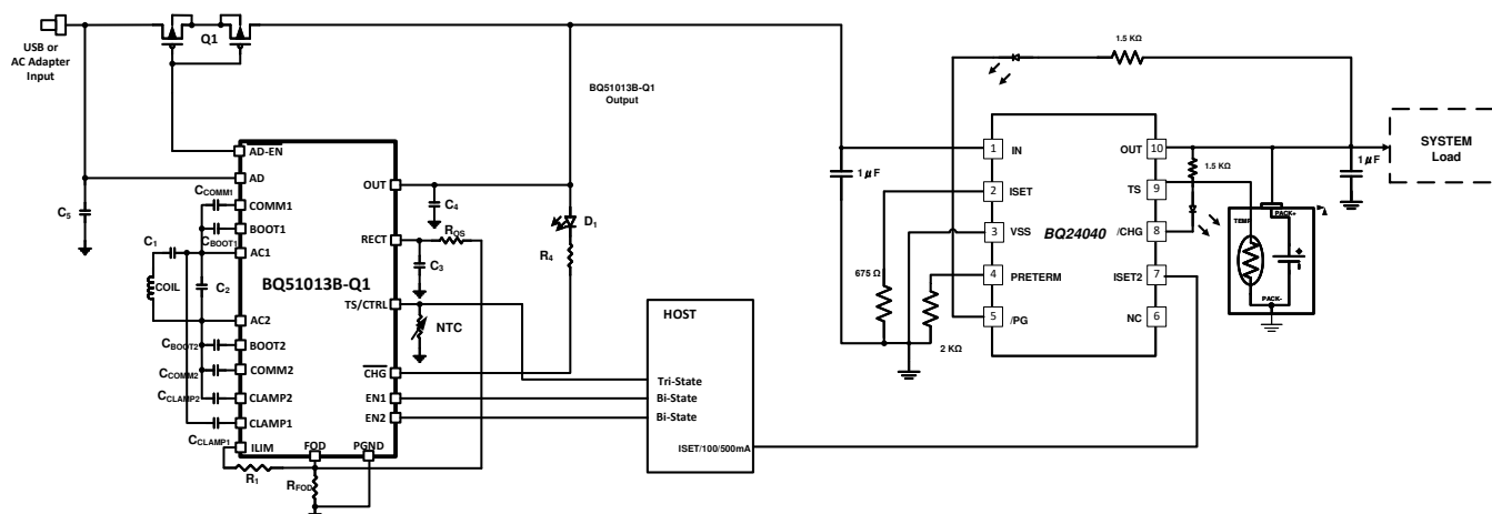
10-11. BQ51013B-Q1 Used as a Wireless Power Supply With Adapter Multiplexing for a Linear Charger
