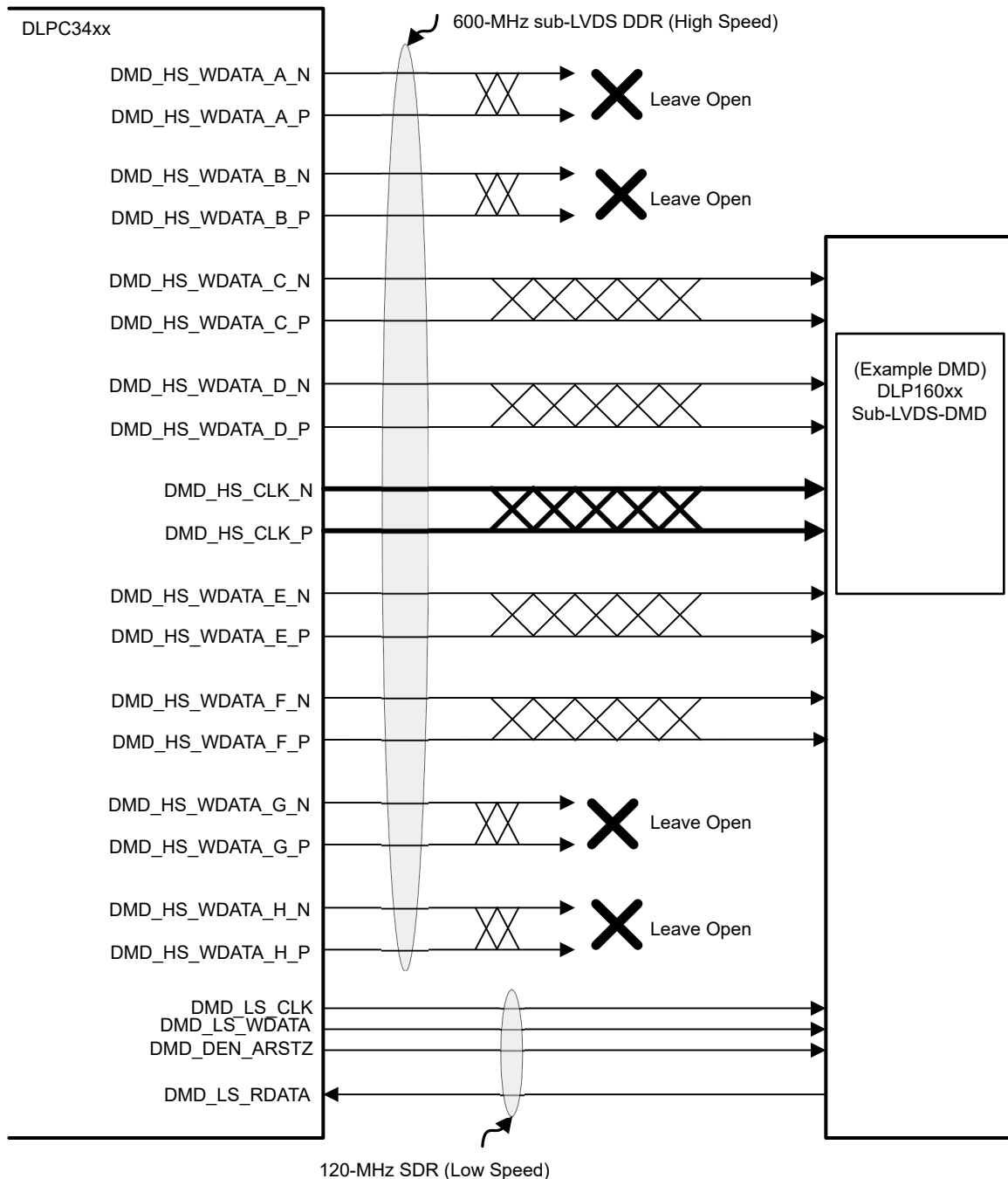
FIG 7-9. DLP160CP (0.16 nHD) DMD Interface Example
