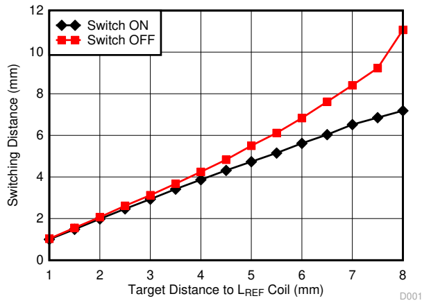
5-1. Switching Distance vs. LREF Target Distance
