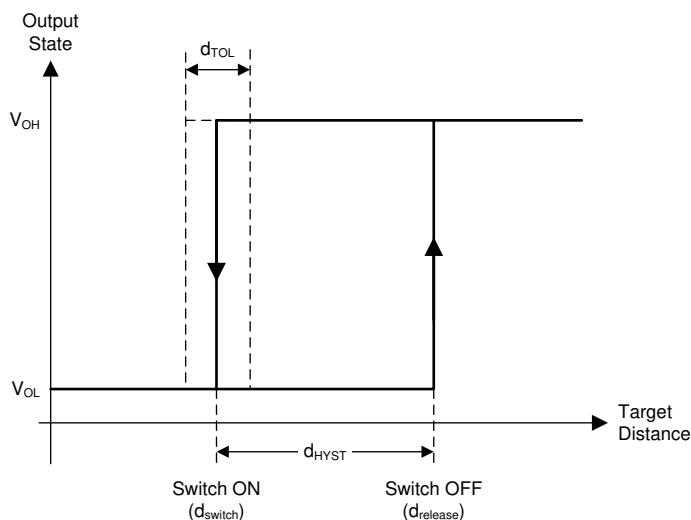
図 6-7. Switching Distance Hysteresis and Threshold Tolerance
