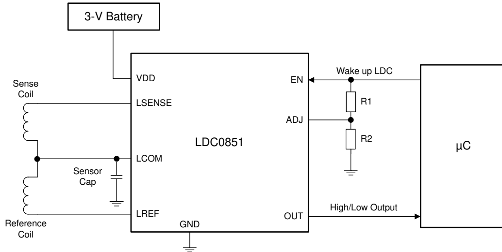
図 7-6. Application Schematic Showing Low Power Operation
