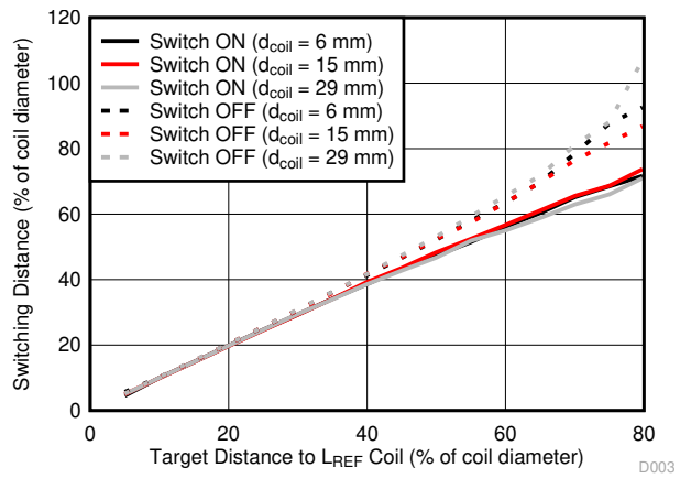
5-1. Switching Distance vs. LREF Target Distance
