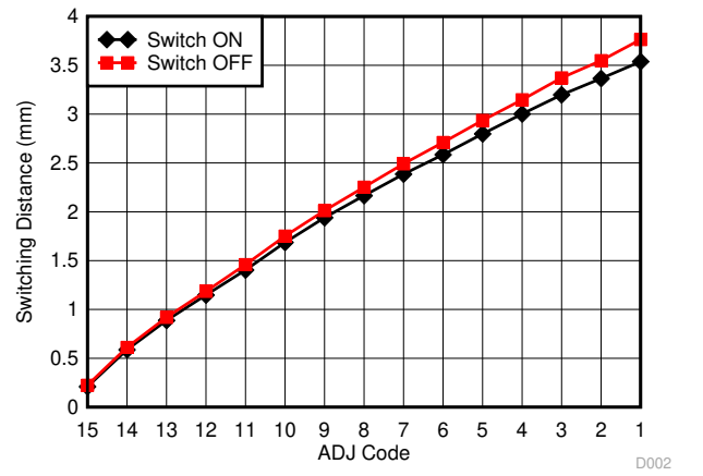
5-2. Switching Distance vs. ADJ code
