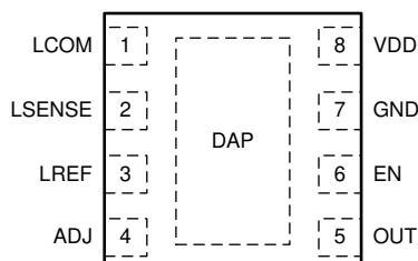
図 4-1. DSG Package 8-Pin WSON with DAP Top View
