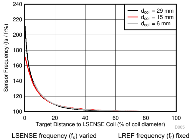
図 5-5. Frequency vs. Distance
