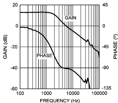
図 7-3. Modulator Gain and Phase
