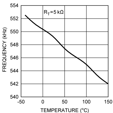
5-15. Frequency vs Temperature
