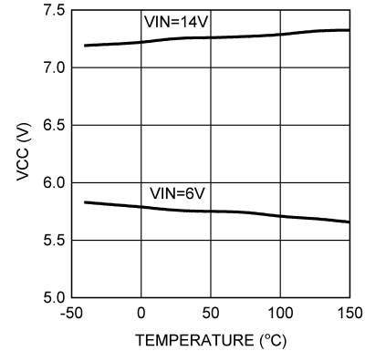
FIG 5-20. VCC vs Temperature
