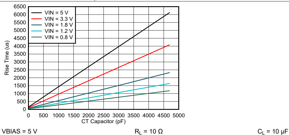
Figure 7-9. Rise Time vs CT Capacitance
