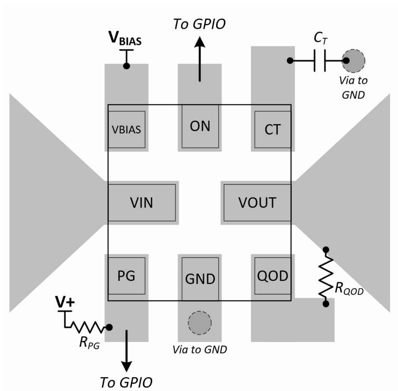
✎ 12-1. TPS22992x Layout Example
