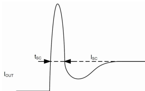
FIG 9-2. Output Short Circuit Response
