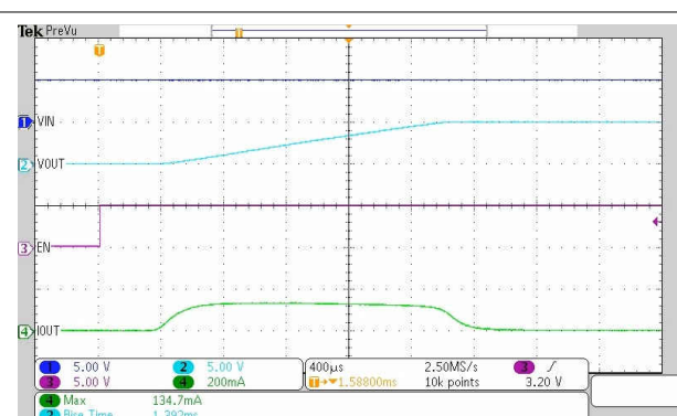
Figure 10-3. Inrush Current for C_L = 47 \text{ } \mu\text{F} with C_T = 1000 \text{ pF}
