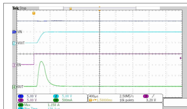
Figure 10-2. Inrush Current for C_L = 47 \text{ } \mu\text{F} with C_T = 0 \text{ pF}
