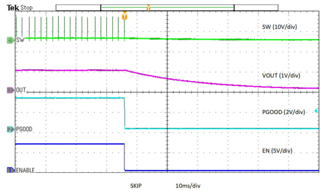
8-17. Enable Power Down, Skip
