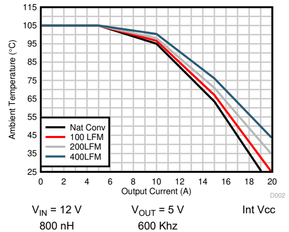
6-4. Safe Operating Area, V OUT = 5 V
