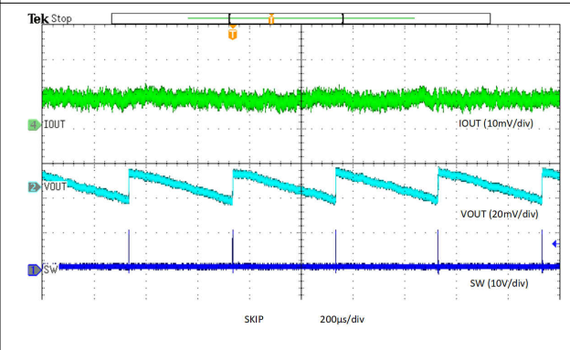
6-18. V OUT Ripple, Skip Mode, 10-mA Load
