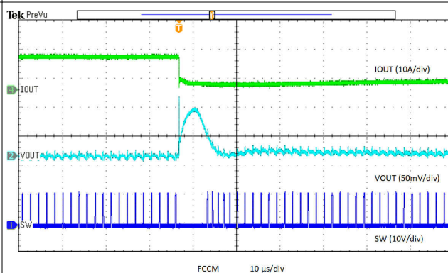
Figure 6-12. Unload Transient
