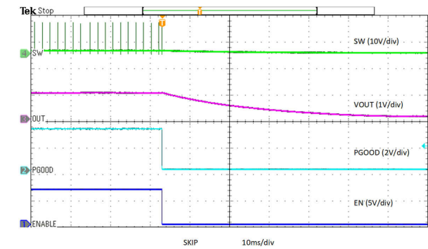
8-19. Enable Power Down with Pre-bias, Skip
