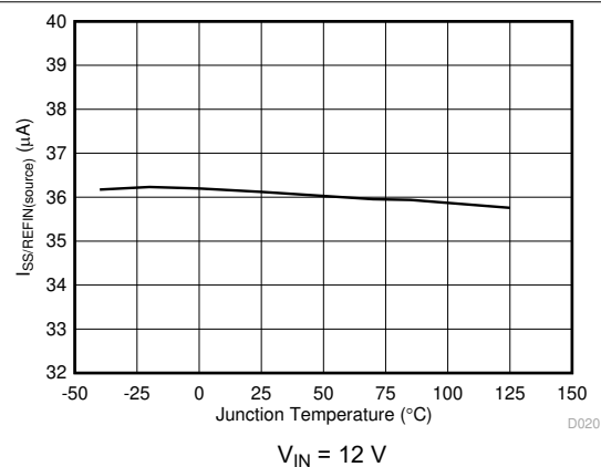
Figure 6-10. I_{SS}(\text{source}) vs Junction Temperature
