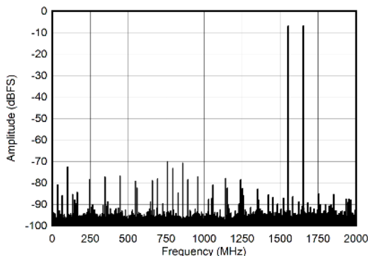
7-25. Dual Channel Mode: Two Tone FFT at 2397 MHz
