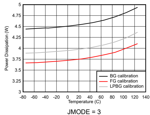
FIG 7-137. Dual Channel Mode: Power Dissipation vs Temperature
