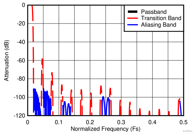
图 8-17. Decimate-by-32 Composite Response
