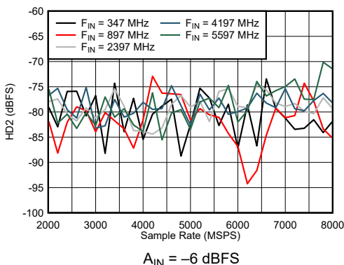
FIG 7-35. DES Mode: HD2 vs Sample Rate and Input Frequency
