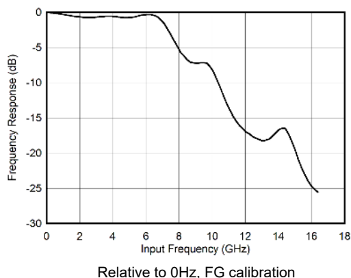
7-1. DES Mode: Input Amplitude vs Input Frequency
