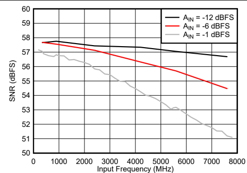
7-82. DES Mode: F_{\text{IN}} \pm F_S/4 vs Input Frequency
