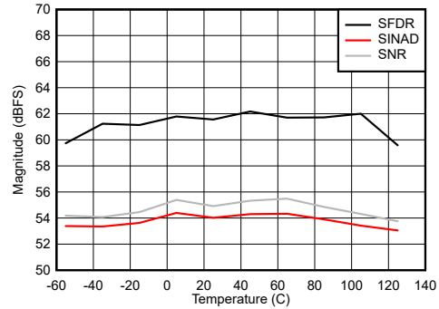
7-92. DES Mode: SNR, SINAD and SFDR vs Temperature
