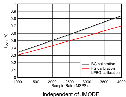
FIG 7-127. Dual Channel Mode: I_{VA11} vs Sample Rate
