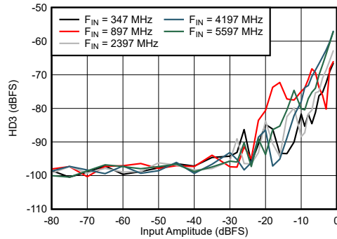
7-73. Dual Channel Mode: HD3 vs Input Amplitude and Frequency
