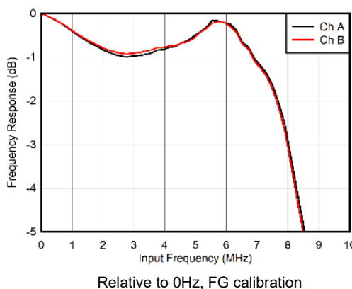
7-4. Input Response vs Input Frequency (zoomed)
