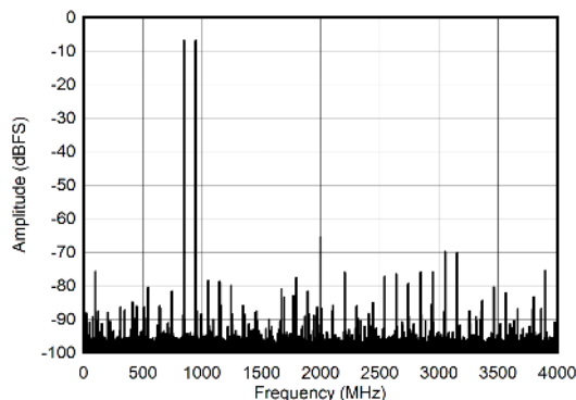
7-14. DES Mode: Two Tone FFT at 897 MHz
