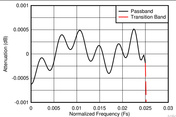
8-16. Decimate-by-16 Composite Zoomed Pass-Band Response
