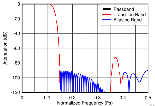
8-11. Decimate-by-4 Composite Response
