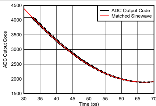
7-144. Sinewave Overdrive Recovery
