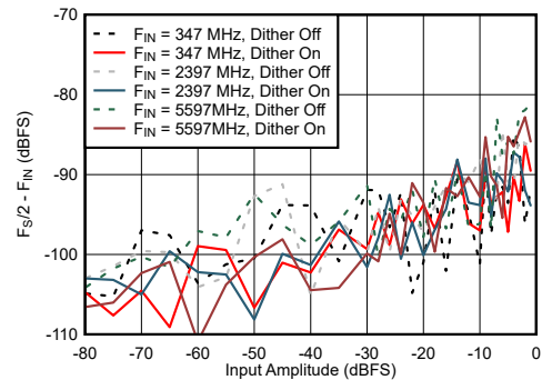
7-76. Dual Channel Mode: F_{S/2} - F_{\text{IN}} vs Input Amplitude and Dither
