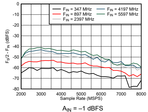
FIG 7-40. DES Mode: F_S/2 - F_{\text{IN}} vs Sample Rate and Input Frequency
