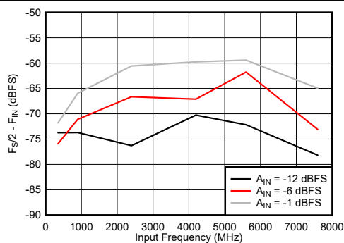
7-81. DES Mode: F_S/2 - F_{\text{IN}} vs Input Frequency
