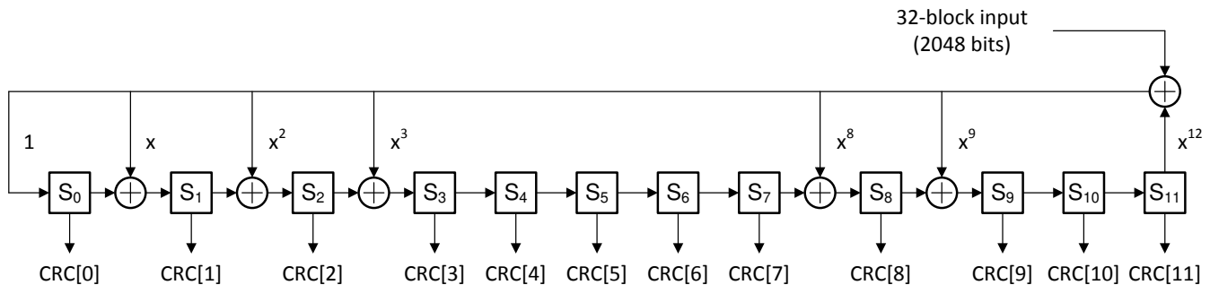
図 8-21. CRC-12 Parity Bit Generator
