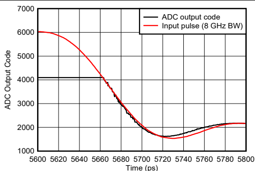
7-142. Pulse Overdrive Recovery Zoomed
