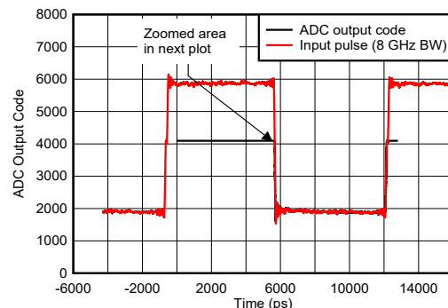
FIG 7-141. Pulse Overdrive Recovery
