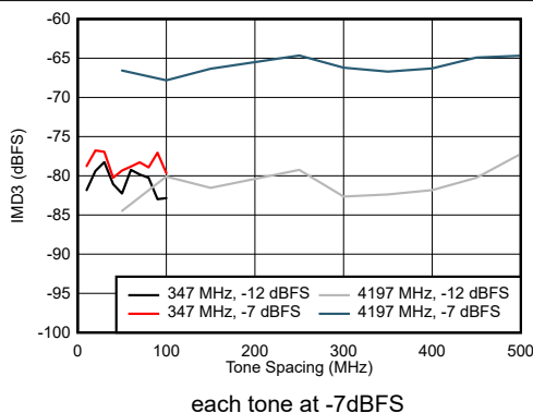
FIG 7-109. Dual Channel Mode: IMD3 vs Tone Spacing
