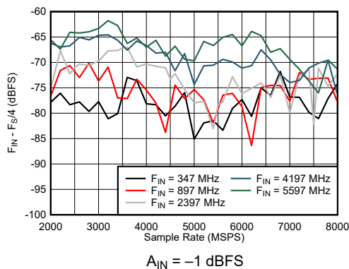
FIG 7-41. DES Mode: F_{\text{IN}} \pm F_S/4 vs Sample Rate and Input Frequency
