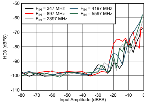
7-61. DES Mode: HD3 vs Input Amplitude and Frequency
