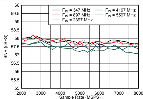
7-30. DES Mode: SNR vs Sample Rate and Input Frequency
