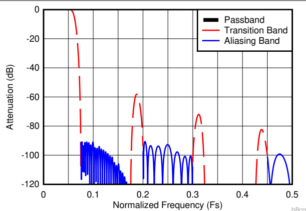
8-13. Decimate-by-8 Composite Response
