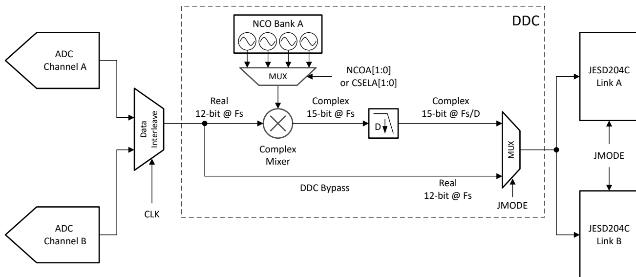
8-9. Digital Down Conversion Block in Single Channel Mode
