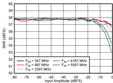
FIG 7-55. DES Mode: SNR vs Input Amplitude and Frequency
