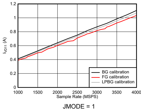
7-118. DES Mode: I_{VD11} vs Sample Rate
