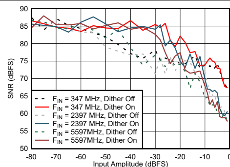
FIG 7-58. DES Mode: SFDR vs Input Amplitude and Dither
