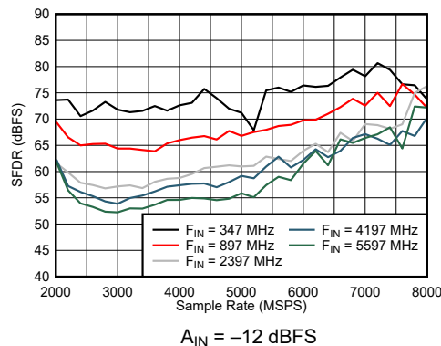
FIG 7-33. DES Mode: SFDR vs Sample Rate and Input Frequency
