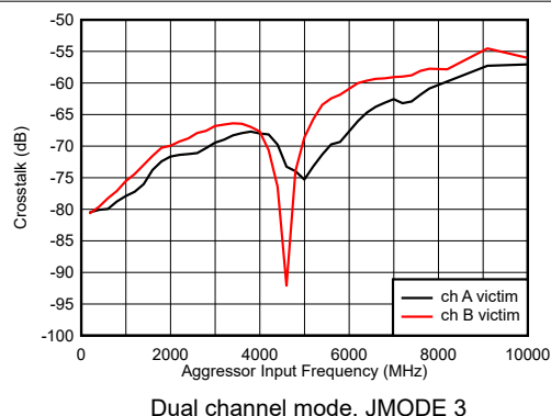
7-5. Crosstalk vs Input Frequency
