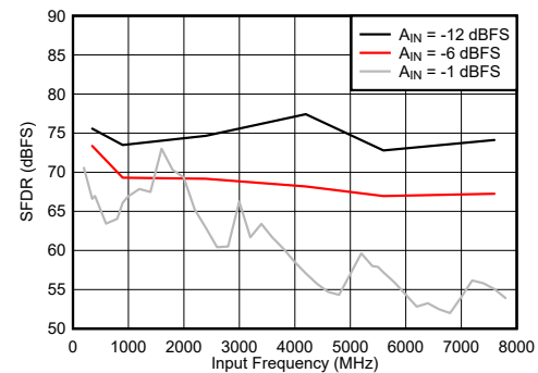
7-84. Dual Channel Mode: SFDR vs Input Frequency
