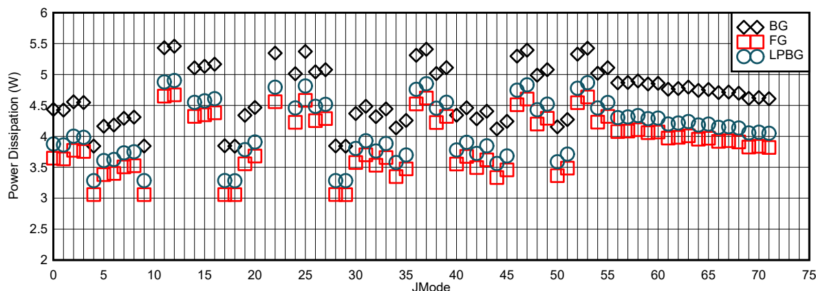
7-114. Power Dissipation vs JMODE at F_{\text{CLK}} = 4\text{ GHz}
