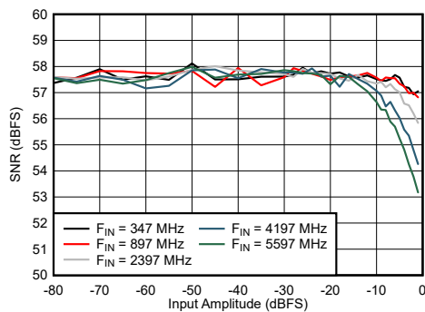
7-67. Dual Channel Mode: SNR vs Input Amplitude and Frequency
