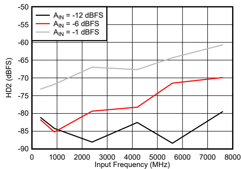
7-79. DES Mode: HD2 vs Input Frequency
