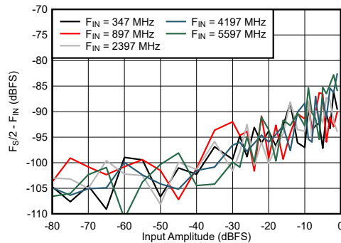
7-75. Dual Channel Mode: F_{S/2} - F_{\text{IN}} vs Input Amplitude and Frequency
