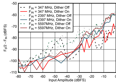
7-64. DES Mode: F_S/2 - F_{\text{IN}} vs Input Amplitude and Dither
