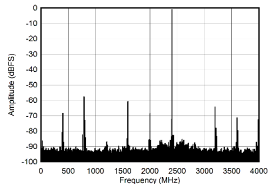
Figure 7-12. DES Mode: Single Tone FFT at 5597 MHz
