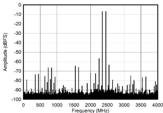
7-17. DES Mode: Two Tone FFT at 5597 MHz
