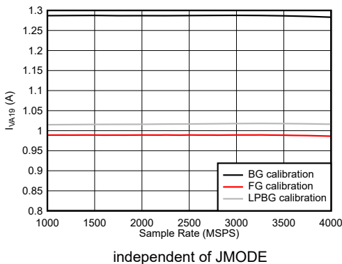
FIG 7-126. Dual Channel Mode: I_{VA19} vs Sample Rate
