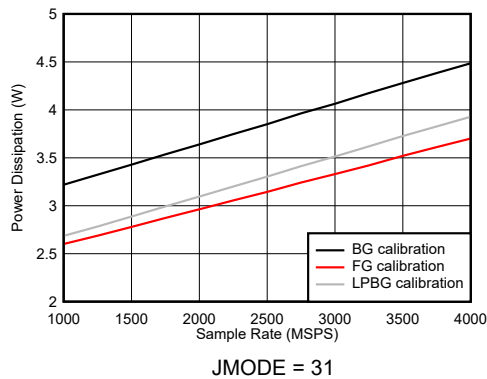
FIG 7-134. Dual Channel Mode: Power Dissipation vs Sample Rate
