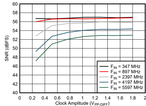
7-90. Dual Channel Mode: SNR vs Clock Amplitude
