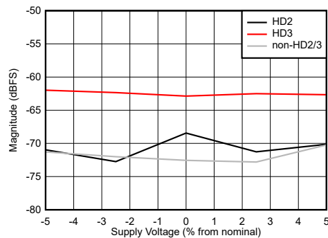
FIG 7-103. Dual Channel Mode: HD2, HD3 and Worst non-HD Spur vs Supply Voltage
