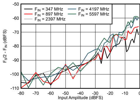
7-63. DES Mode: F_S/2 - F_{\text{IN}} vs Input Amplitude and Frequency
