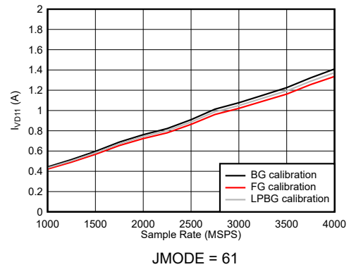
7-121. DES Mode: I_{VD11} vs Sample Rate
