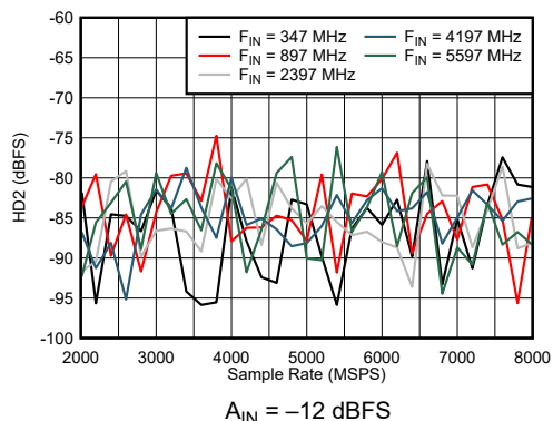
FIG 7-36. DES Mode: HD2 vs Sample Rate and Input Frequency
