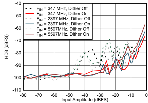
7-74. Dual Channel Mode: HD3 vs Input Amplitude and Dither
