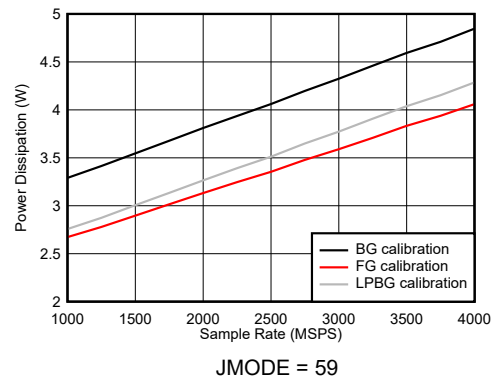
FIG 7-135. Dual Channel Mode: Power Dissipation vs Sample Rate
