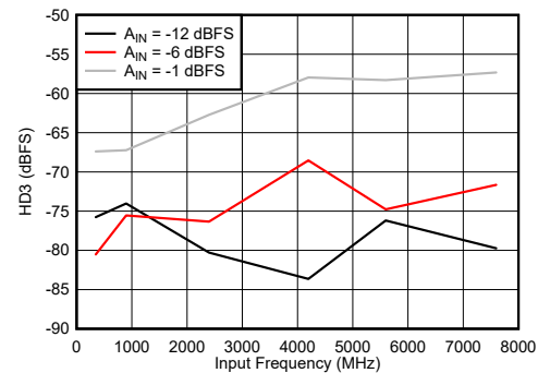
7-80. DES Mode: HD3 vs Input Frequency
