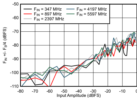
7-65. DES Mode: F_{\text{IN}} \pm F_S/4 vs Input Amplitude and Frequency
