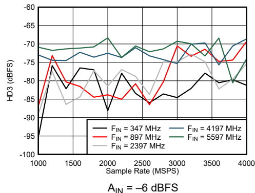
7-52. Dual Channel Mode: HD3 vs Sample Rate and Input Frequency
