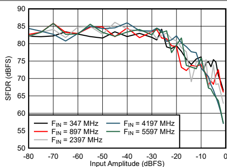
7-69. Dual Channel Mode: SFDR vs Input Amplitude and Frequency
