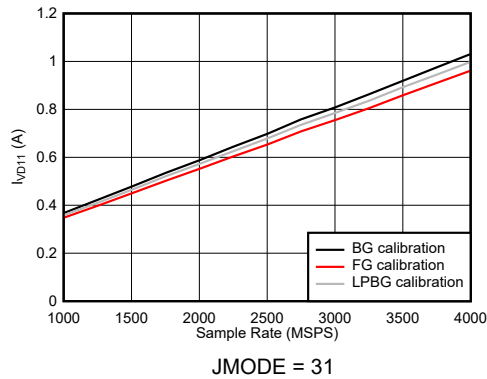
FIG 7-130. Dual Channel Mode: I_{VD11} vs Sample Rate
