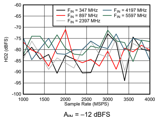
7-50. Dual Channel Mode: HD2 vs Sample Rate and Input Frequency
