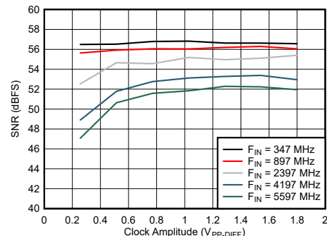
7-88. DES Mode: SNR vs Clock Amplitude
