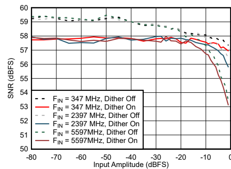
FIG 7-56. DES Mode: SNR vs Input Amplitude and Dither
