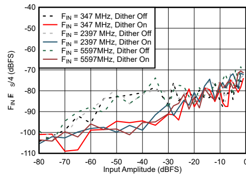
7-66. DES Mode: F_{\text{IN}} \pm F_S/4 vs Input Amplitude and Dither
