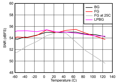
7-94. Dual Channel Mode: SNR, SINAD and SFDR vs Temperature
