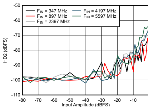
FIG 7-59. DES Mode: HD2 vs Input Amplitude and Frequency
