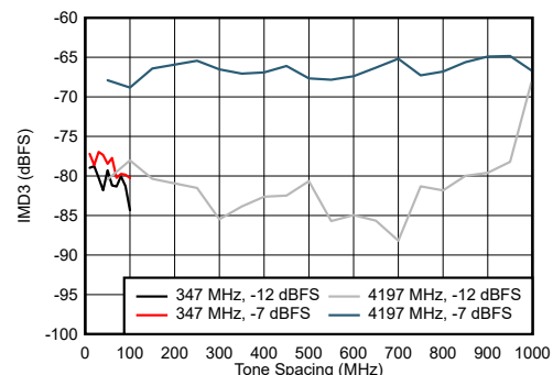
FIG 7-108. DES Mode: IMD3 vs Tone Spacing
