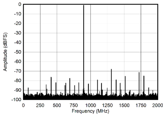
FIG 7-19. Dual Channel Mode: Single Tone FFT at 897 MHz
