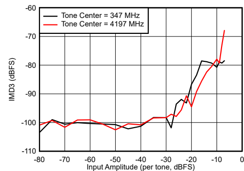
FIG 7-106. DES Mode: IMD3 vs Input Amplitude
