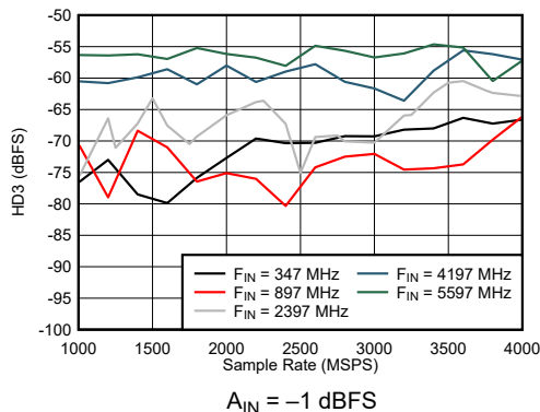
7-51. Dual Channel Mode: HD3 vs Sample Rate and Input Frequency
