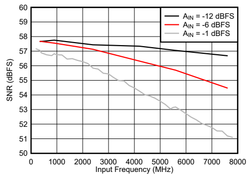
7-83. Dual Channel Mode: SNR vs Input Frequency
