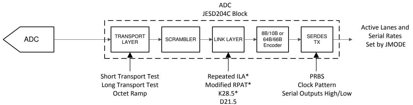
图 8-25. Test Mode Insertion Points
