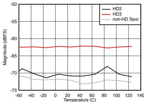
7-93. DES Mode: HD2, HD3 and Worst non-HD Spur vs Temperature
