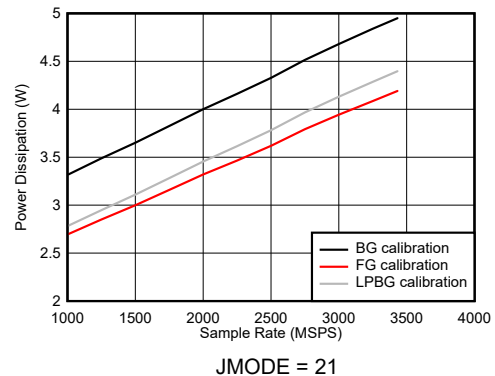
7-123. DES Mode: Power Dissipation vs Sample Rate
