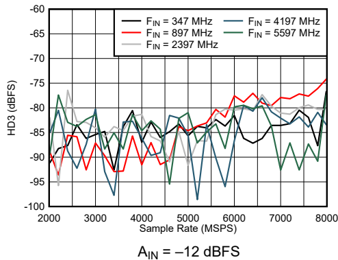
FIG 7-39. DES Mode: HD3 vs Sample Rate and Input Frequency
