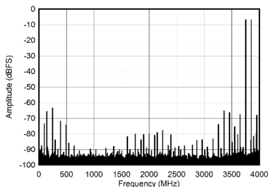
7-16. DES Mode: Two Tone FFT at 4197 MHz
