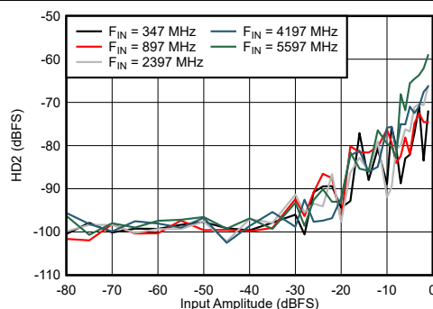
7-71. Dual Channel Mode: HD2 vs Input Amplitude and Frequency
