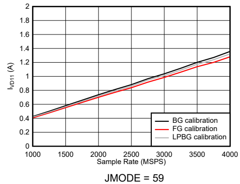
FIG 7-131. Dual Channel Mode: I_{VD11} vs Sample Rate
