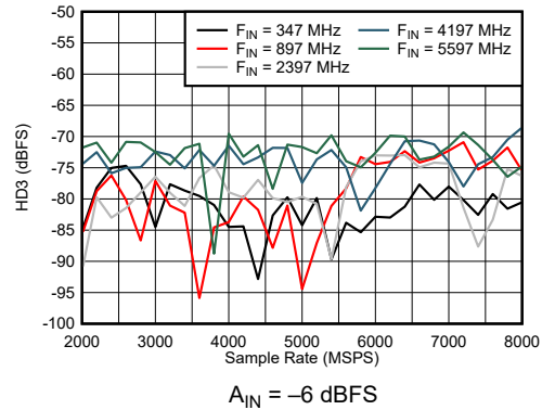
FIG 7-38. DES Mode: HD3 vs Sample Rate and Input Frequency
