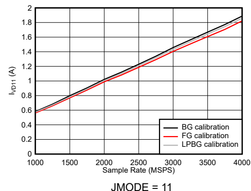
FIG 7-129. Dual Channel Mode: I_{VD11} vs Sample Rate
