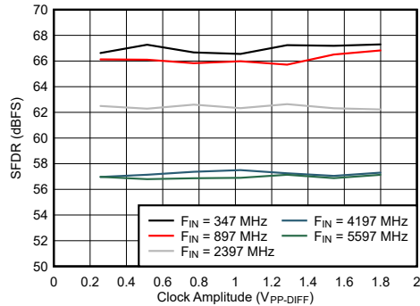
7-91. Dual Channel Mode: SFDR vs Clock Amplitude
