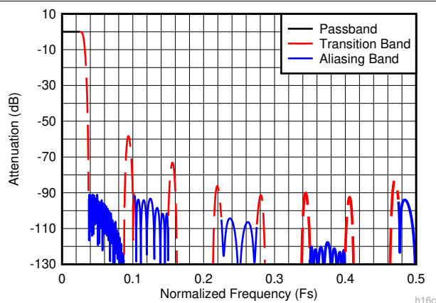
8-15. Decimate-by-16 Composite Response
