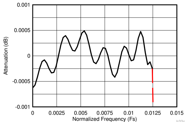
图 8-18. Decimate-by-32 Composite Zoomed Pass-Band Response
