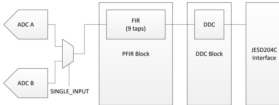
图 8-5. Single Channel Equalization PFIR Block Diagram
