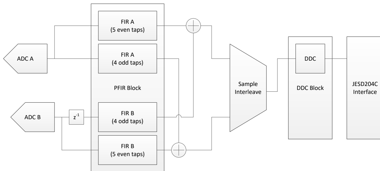
✕ 8-7. Alternate I/Q Correction-Type Filter Block Diagram
