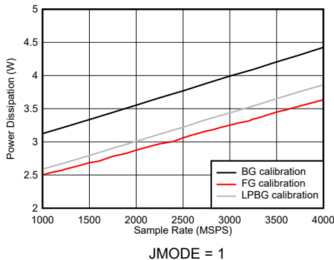
7-122. DES Mode: Power Dissipation vs Sample Rate
