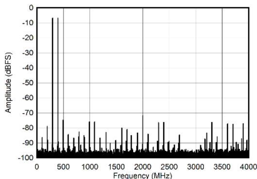
7-13. DES Mode: Two Tone FFT at 347 MHz
