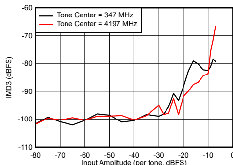
FIG 7-107. Dual Channel Mode: IMD3 vs Input Amplitude
