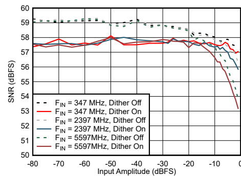
7-68. Dual Channel Mode: SNR vs Input Amplitude and Dither
