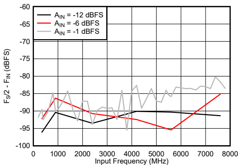
7-87. Dual Channel Mode: F_S/2 - F_{\text{IN}} vs Input Frequency
