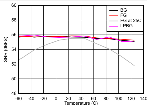
FIG 7-98. Dual Channel Mode: SNR vs Temperature and Calibration Mode
