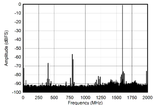
FIG 7-22. Dual Channel Mode: Single Tone FFT at 5597 MHz
