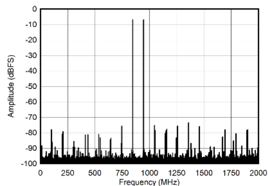
FIG 7-24. Dual Channel Mode: Two Tone FFT at 897 MHz
