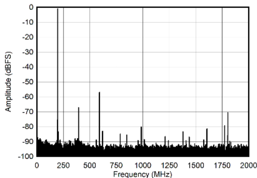
FIG 7-21. Dual Channel Mode: Single Tone FFT at 4197 MHz
