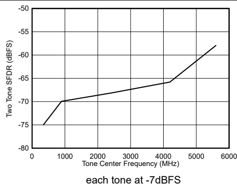
FIG 7-110. DES Mode: Two Tone SFDR vs Input Frequency
