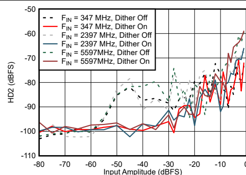
7-72. Dual Channel Mode: HD2 vs Input Amplitude and Dither
