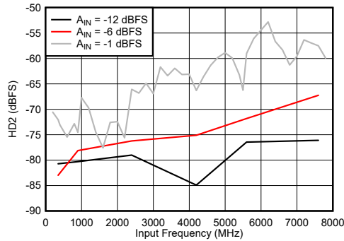
7-85. Dual Channel Mode: HD2 vs Input Frequency
