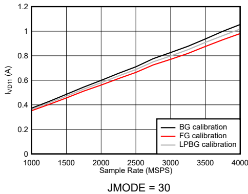
7-120. DES Mode: I_{VD11} vs Sample Rate
