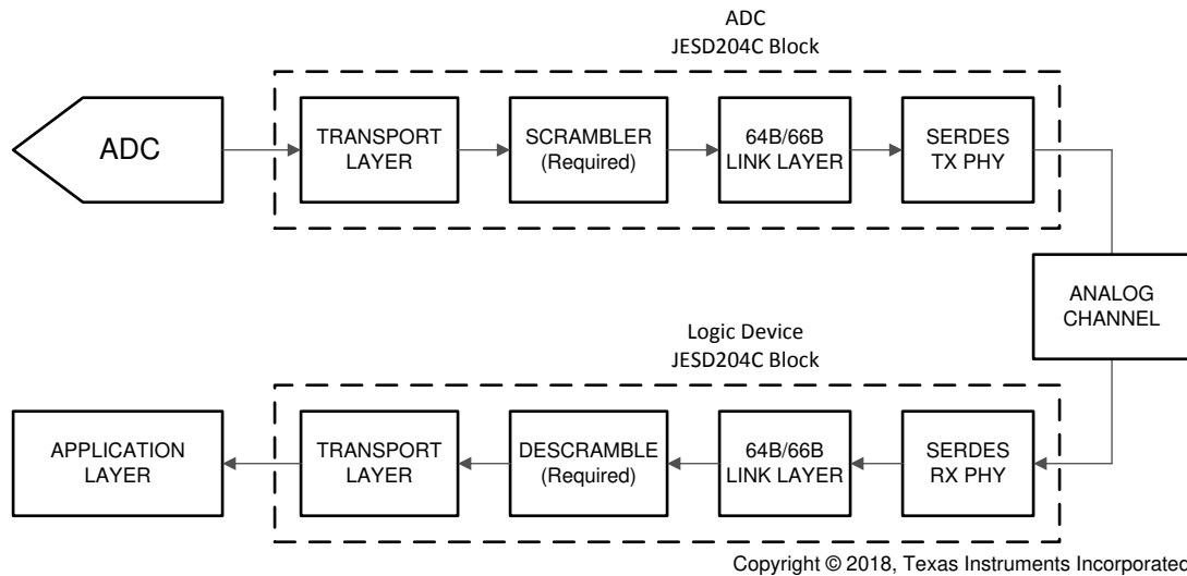
图 8-20. Simplified 64B/66B Encoded JESD204C Interface Diagram
