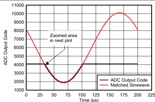
7-143. Sinewave Overdrive Recovery
