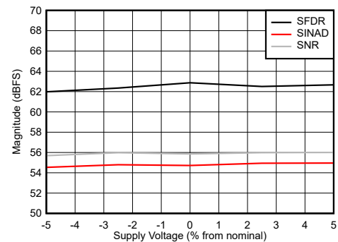
FIG 7-102. Dual Channel Mode: SNR, SINAD and SFDR vs Supply Voltage
