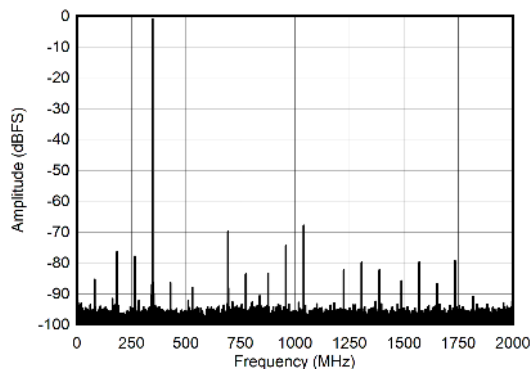
7-18. Dual Channel Mode: Single Tone FFT at 347 MHz
