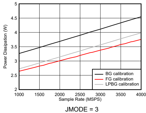
FIG 7-132. Dual Channel Mode: Power Dissipation vs Sample Rate
