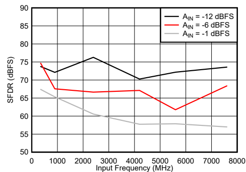
7-78. DES Mode: SFDR vs Input Frequency
