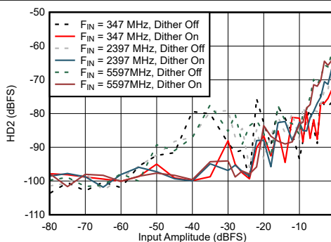
FIG 7-60. DES Mode: HD2 vs Input Amplitude and Dither
