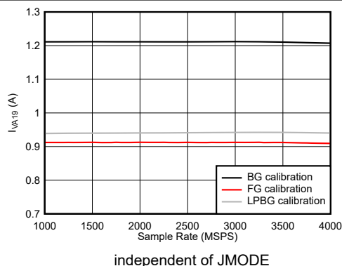
7-116. DES Mode: I_{V_{A19}} vs Sample Rate
