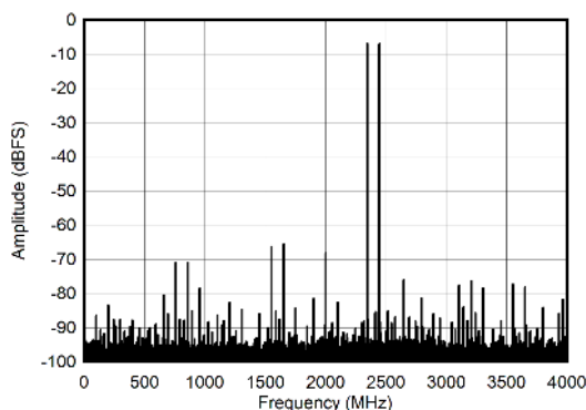
7-15. DES Mode: Two Tone FFT at 2397 MHz
