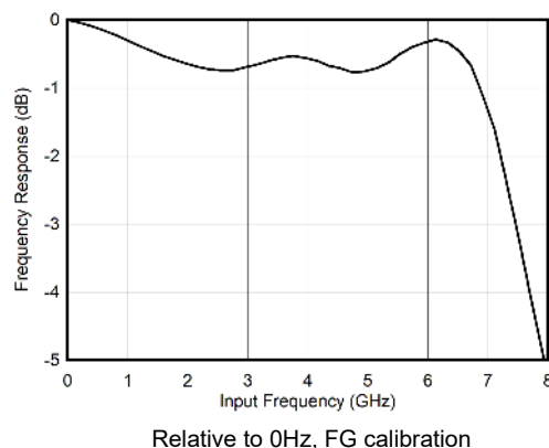
7-2. DES Mode: Input Response vs Input Frequency
