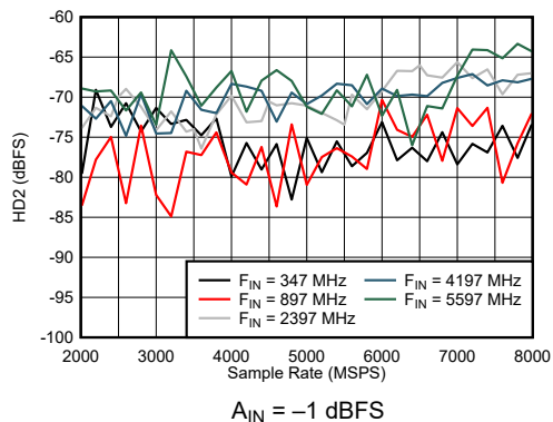
FIG 7-34. DES Mode: HD2 vs Sample Rate and Input Frequency
