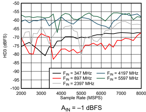
FIG 7-37. DES Mode: HD3 vs Sample Rate and Input Frequency
