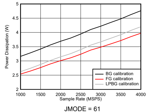
FIG 7-125. DES Mode: Power Dissipation vs Sample Rate
