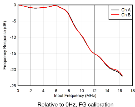
7-3. Dual Channel Mode: Input Amplitude vs Input Frequency
