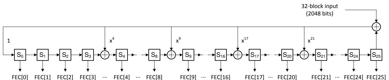
图 8-22. FEC Parity Bit Generator
