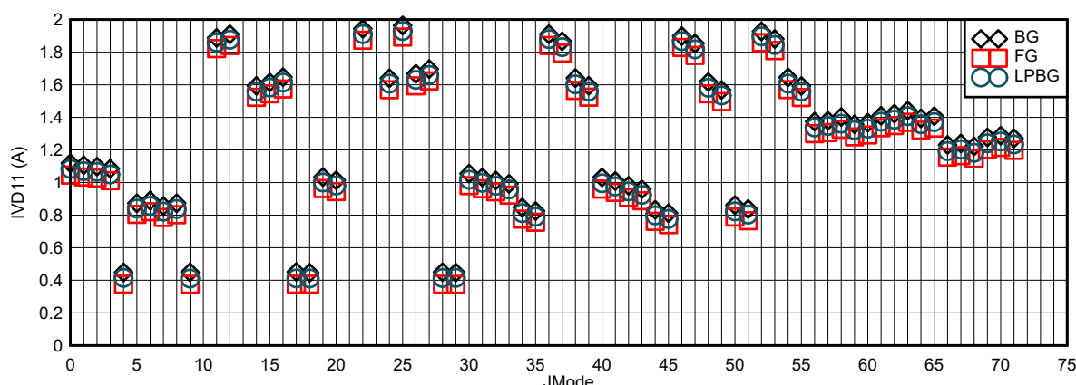
7-115. I_{V_{D11}} vs JMODE at F_{\text{CLK}} = 4\text{ GHz}
