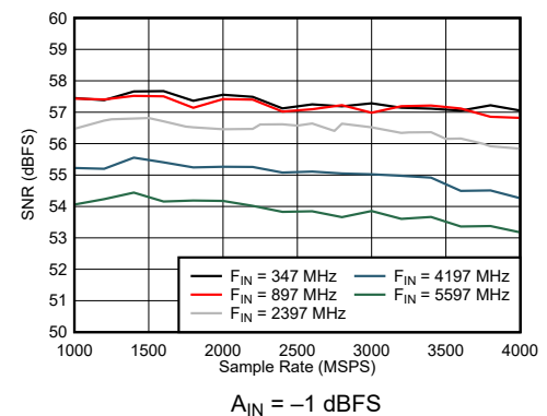
FIG 7-42. Dual Channel Mode: SNR vs Sample Rate and Input Frequency
