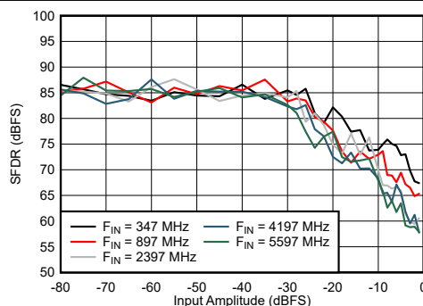
FIG 7-57. DES Mode: SFDR vs Input Amplitude and Frequency
