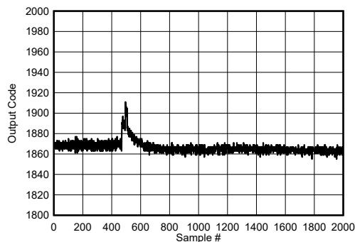
FIG 7-138. Background Calibration Core Transition (DC Offset Signal)
