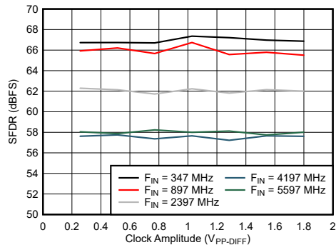
7-89. DES Mode: SFDR vs Clock Amplitude
