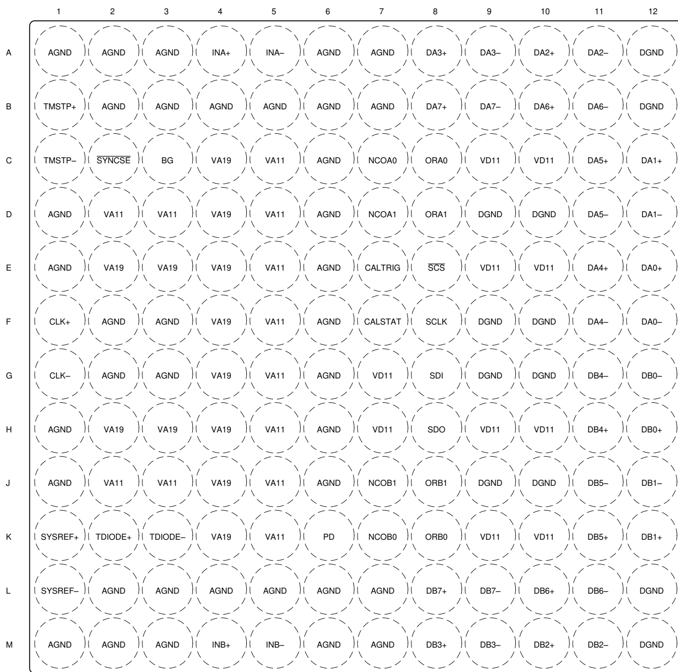
6-1. AAV Package, 144-Ball Flip Chip BGA, Top View
