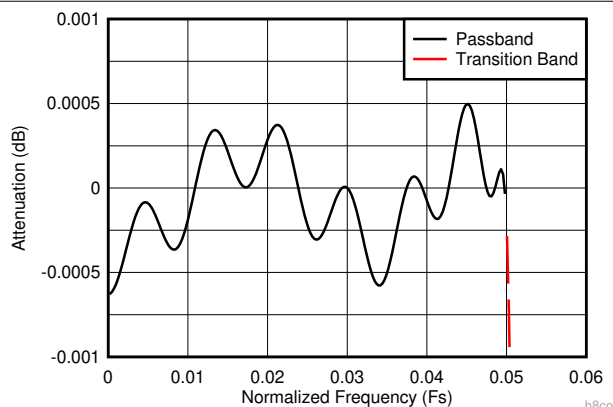
8-14. Decimate-by-8 Composite Zoomed Pass-Band Response
