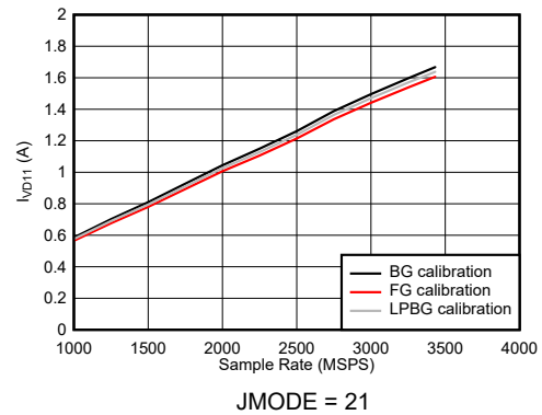
7-119. DES Mode: I_{VD11} vs Sample Rate
