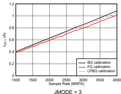
FIG 7-128. Dual Channel Mode: I_{VD11} vs Sample Rate
