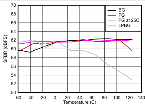
FIG 7-97. DES Mode: SFDR vs Temperature and Calibration Mode
