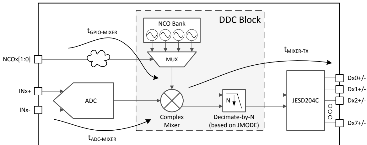
図 8-10. NCO Fast Frequency Hopping Latency Diagram
