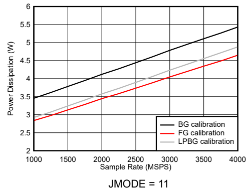
FIG 7-133. Dual Channel Mode: Power Dissipation vs Sample Rate
