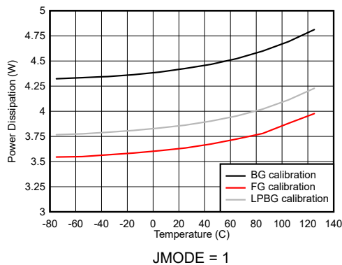
FIG 7-136. DES Mode: Power Dissipation vs Temperature
