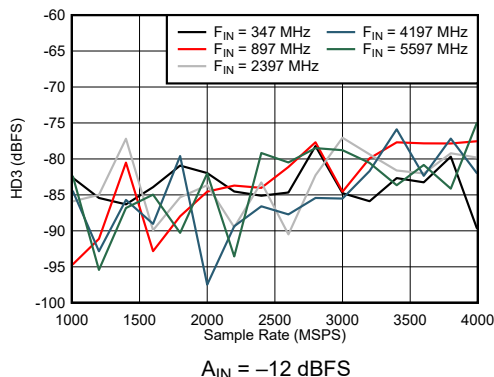
7-53. Dual Channel Mode: HD3 vs Sample Rate and Input Frequency
