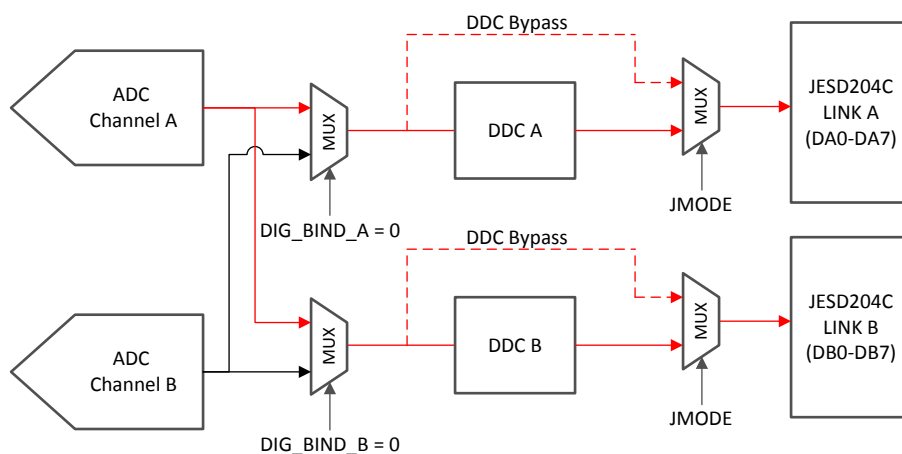
图 8-24. Dual DDC Mode or Redundant Data Mode for Channel A
