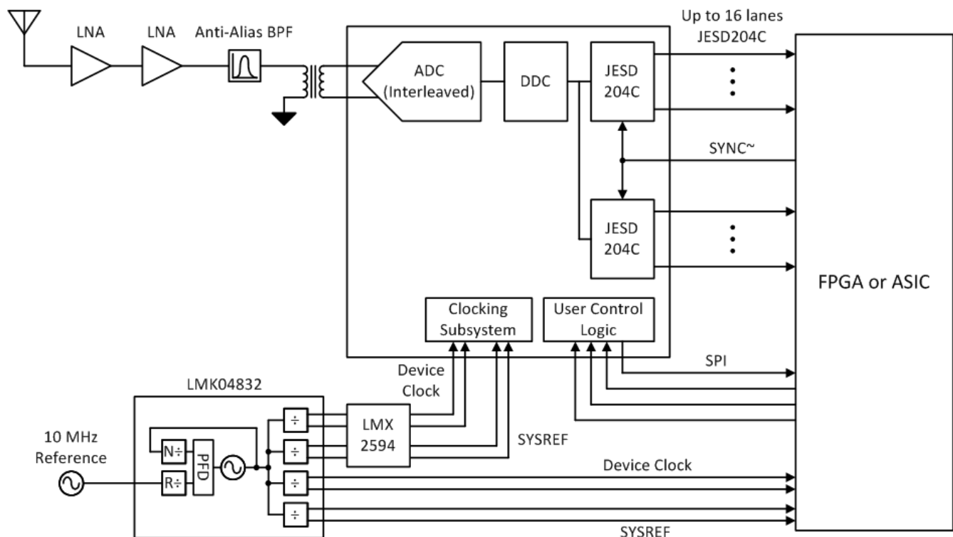
図 9-1. Typical Configuration for Wideband RF Sampling
