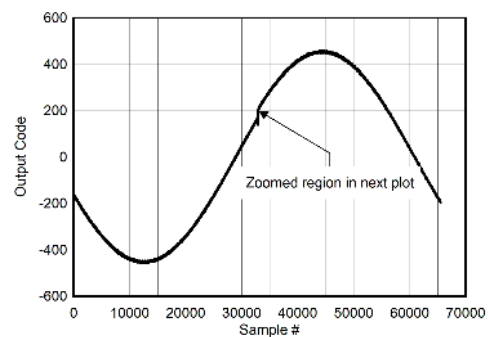
FIG 7-139. Background Calibration Core Transition (AC Signal)
