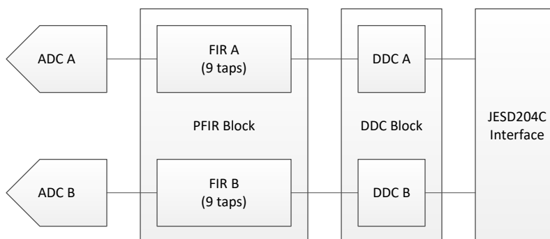
図 8-4. Dual Channel Equalization PFIR Block Diagram
