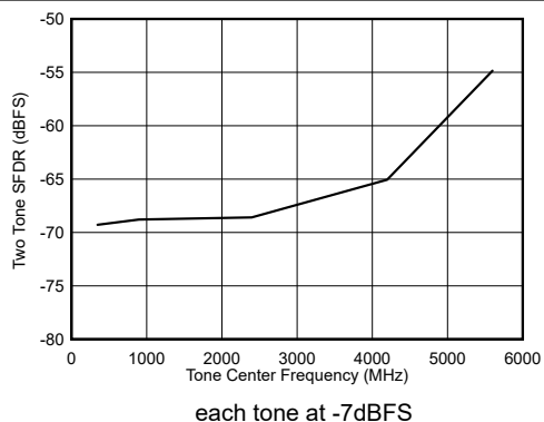
FIG 7-111. Dual Channel Mode: Two Tone SFDR vs Input Frequency
