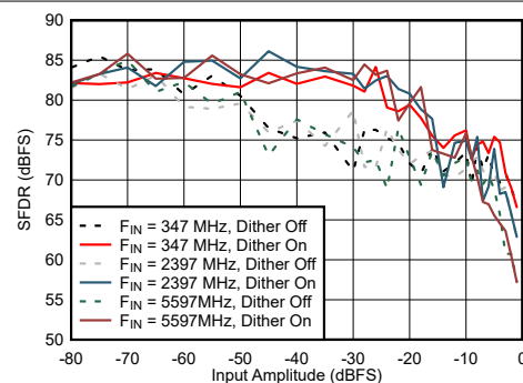
7-70. Dual Channel Mode: SFDR vs Input Amplitude and Dither
