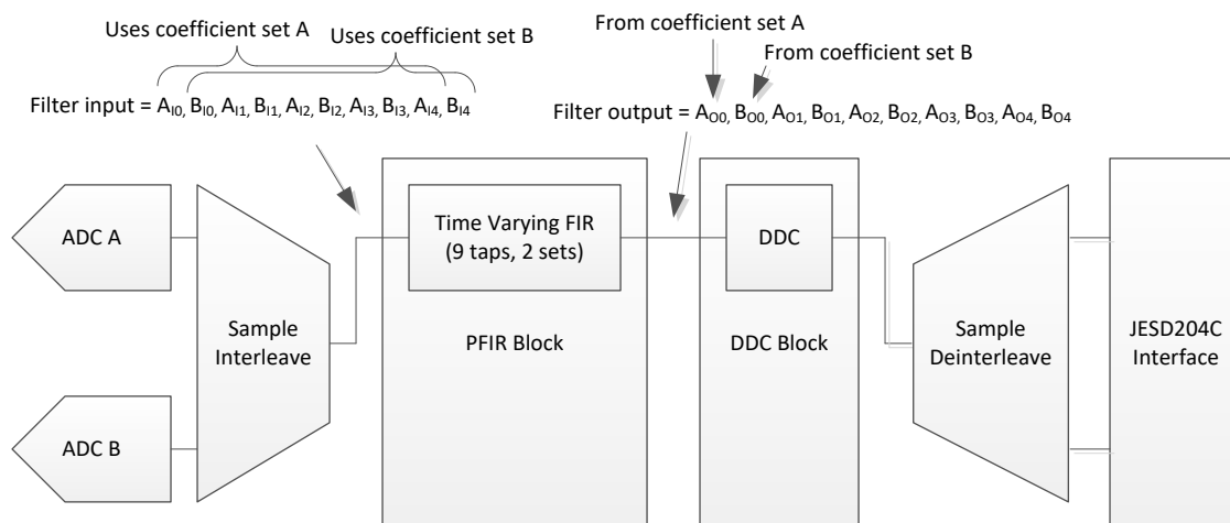
图 8-6. Time Varying Filter PFIR Block Diagram
