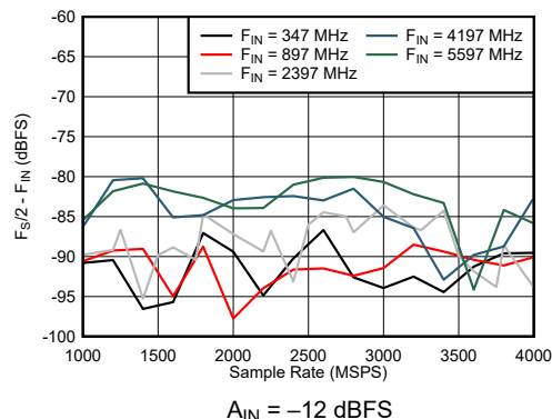
7-54. Dual Channel Mode: F_{\text{S}}/2 - F_{\text{IN}} vs Sample Rate and Input Frequency
