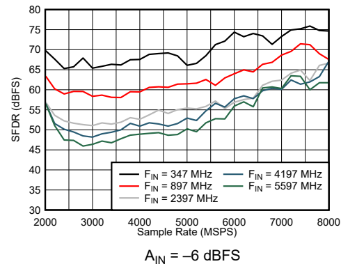
FIG 7-32. DES Mode: SFDR vs Sample Rate and Input Frequency
