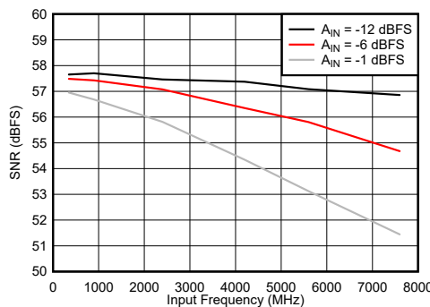
7-77. DES Mode: SNR vs Input Frequency
