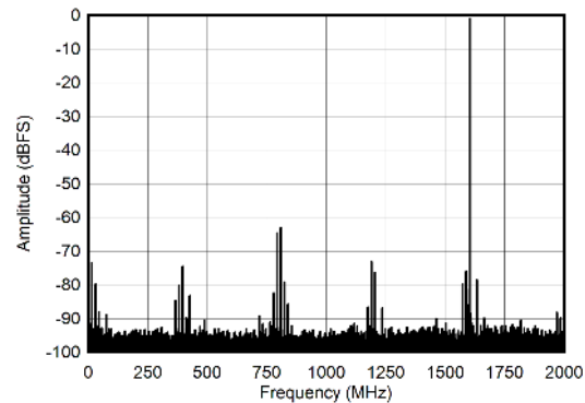
FIG 7-20. Dual Channel Mode: Single Tone FFT at 2397 MHz
