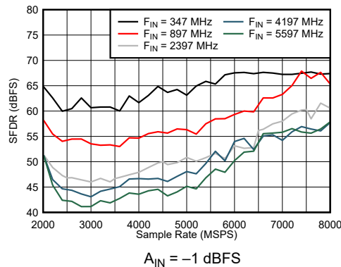
FIG 7-31. DES Mode: SFDR vs Sample Rate and Input Frequency
