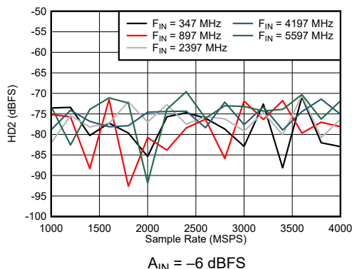
7-49. Dual Channel Mode: HD2 vs Sample Rate and Input Frequency
