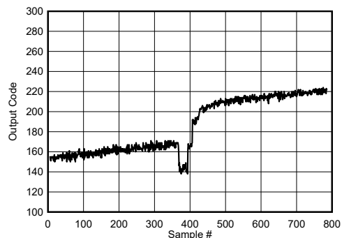
FIG 7-140. Background Calibration Core Transition (AC Signal Zoomed)
