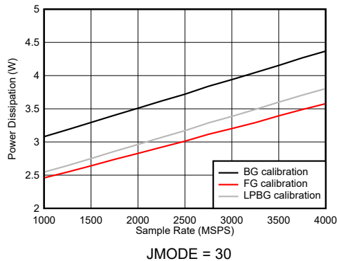
FIG 7-124. DES Mode: Power Dissipation vs Sample Rate
