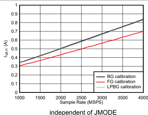
7-117. DES Mode: I_{V_{A11}} vs Sample Rate
