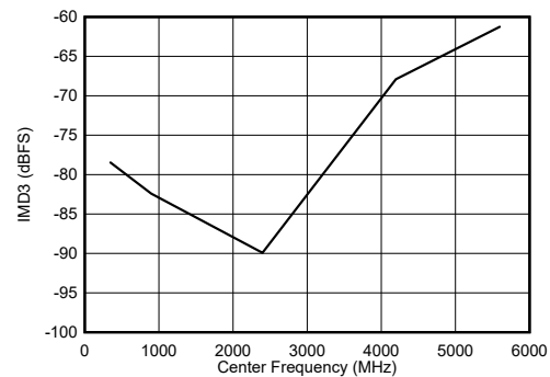
FIG 7-104. DES Mode: IMD3 vs Input Frequency
