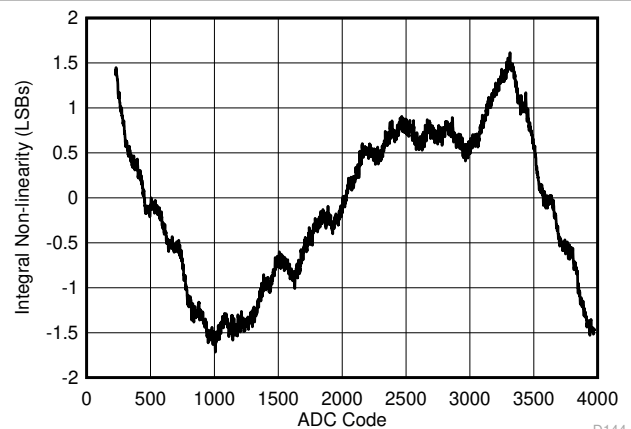
FIG 6-4. INL vs ADC Code
