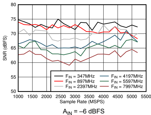
6-49. Dual Channel Mode: SNR vs Sample Rate and Input Frequency
