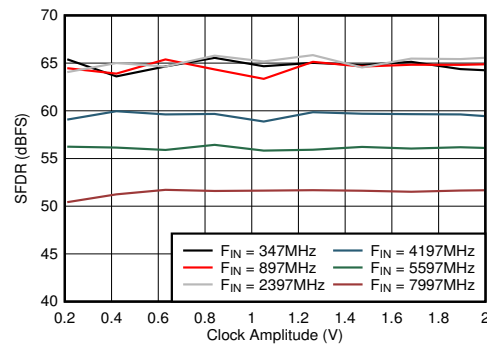
FIG 6-86. Dual Channel Mode: SFDR vs Clock Amplitude
