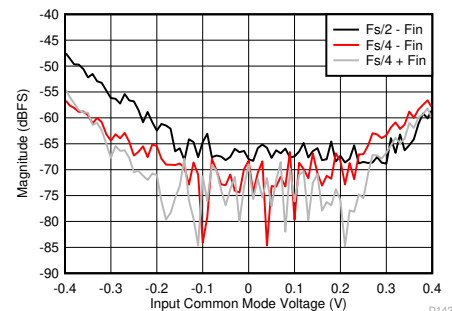
FIG 6-100. F_s/2 - F_{\text{IN}} and F_s/4 \pm F_{\text{IN}} vs Input Common Mode Voltage
