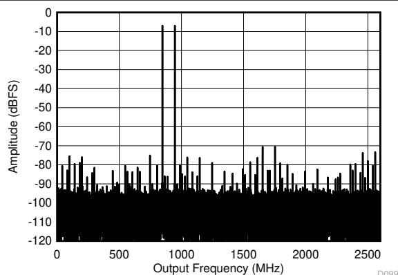
each tone at -7 dBFS, 100 MHz Tone Spacing FIG 6-24. Dual Channel Mode: Two Tone FFT at 897 MHz
