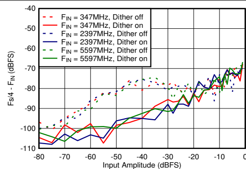
FIG 6-72. DES Mode: F_s/4 - F_{\text{IN}} vs Input Amplitude and Dither
