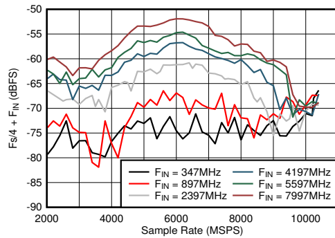
FIG 6-43. DES Mode: F_s/4 + F_{IN} vs Sample Rate and Input Frequency
