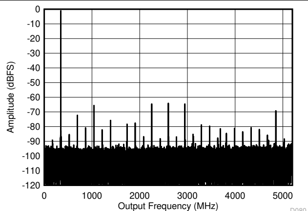
FIG 6-5. DES Mode: Single Tone FFT at 347 MHz
