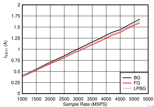
FIG 6-136. Dual Channel Mode: I_{VD11} vs Sample Rate
