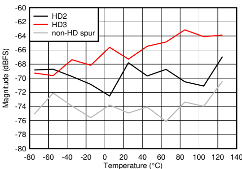
FIG 6-89. DES Mode: HD2, HD3 and Worst non-HD Spur vs Temperature
