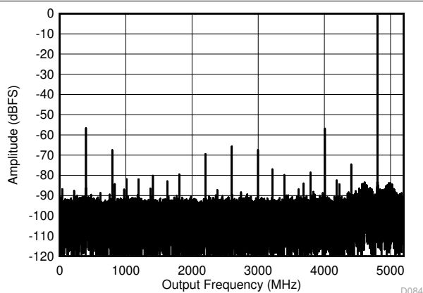
6-9. DES Mode: Single Tone FFT at 5597 MHz
