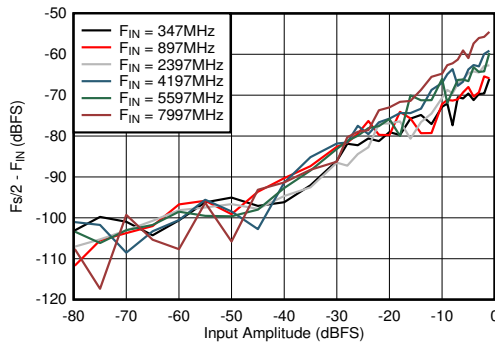
FIG 6-67. DES Mode: F_s/2 - F_{\text{IN}} vs Input Amplitude and Frequency
