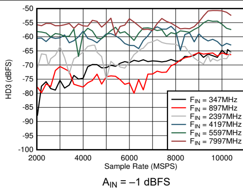
FIG 6-39. DES Mode: HD3 vs Sample Rate and Input Frequency
