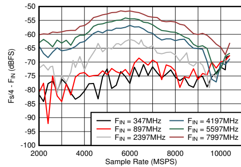
FIG 6-44. DES Mode: F_s/4 - F_{IN} vs Sample Rate and Input Frequency
