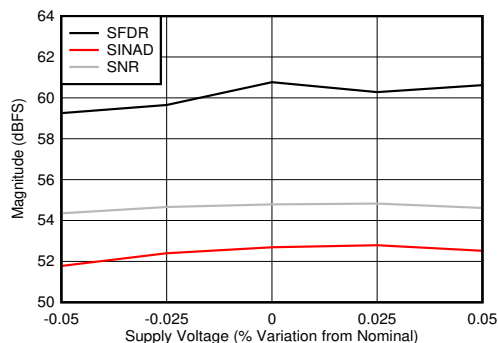
FIG 6-95. DES Mode: SNR, SINAD and SFDR vs Supply Voltage
