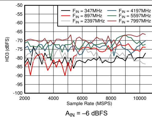
FIG 6-40. DES Mode: HD3 vs Sample Rate and Input Frequency
