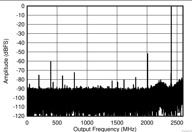
FIG 6-22. Dual Channel Mode: Single Tone FFT at 7997 MHz
