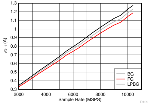
FIG 6-127. DES Mode: I_{VD11} vs Sample Rate
