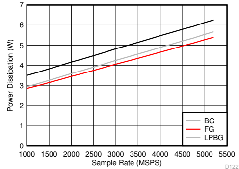
FIG 6-140. Dual Channel Mode: Power Dissipation vs Sample Rate
