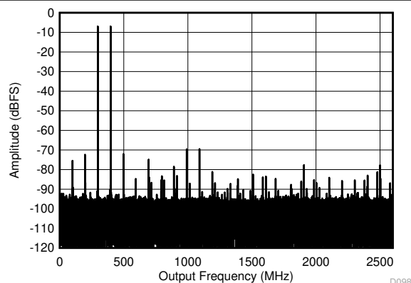
each tone at -7 dBFS, 100 MHz Tone Spacing FIG 6-23. Dual Channel Mode: Two Tone FFT at 347 MHz
