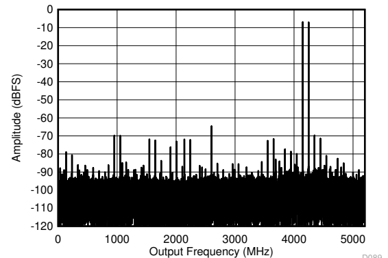
FIG 6-14. DES Mode: Two Tone FFT at 4197 MHz
