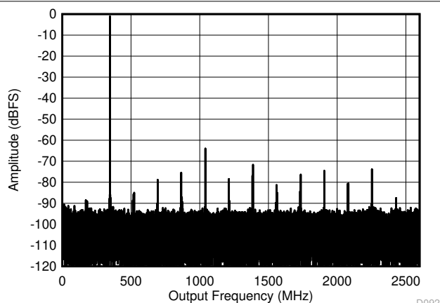
FIG 6-17. Dual Channel Mode: Single Tone FFT at 347 MHz
