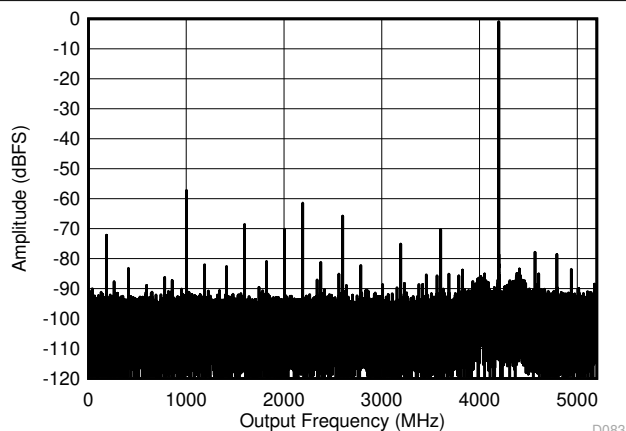
6-8. DES Mode: Single Tone FFT at 4197 MHz
