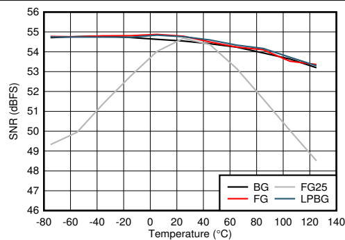
FIG 6-92. Dual Channel Mode: SNR vs Temperature and Calibration Mode
