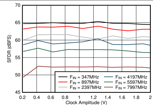
FIG 6-84. DES Mode: SFDR vs Clock Amplitude
