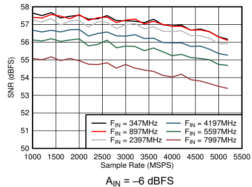
FIG 6-46. Dual Channel Mode: SNR vs Sample Rate and Input Frequency
