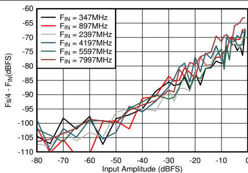
FIG 6-71. DES Mode: F_s/4 - F_{\text{IN}} vs Input Amplitude and Frequency
