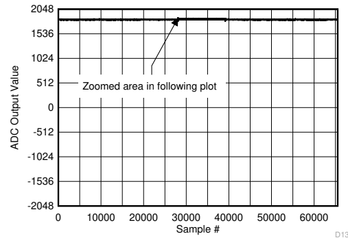
6-146. Background Calibration Core Transition (DC Signal)
