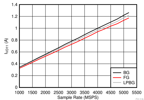
FIG 6-135. Dual Channel Mode: I_{VD11} vs Sample Rate
