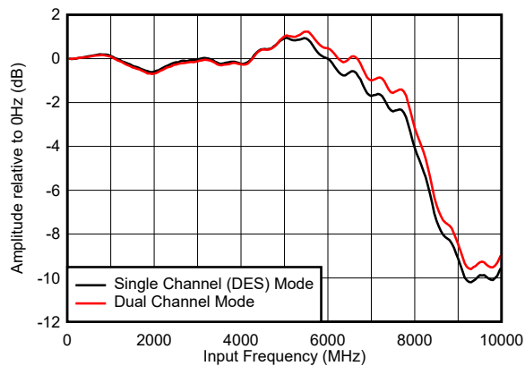
FIG 6-1. Input Amplitude vs Input Frequency
