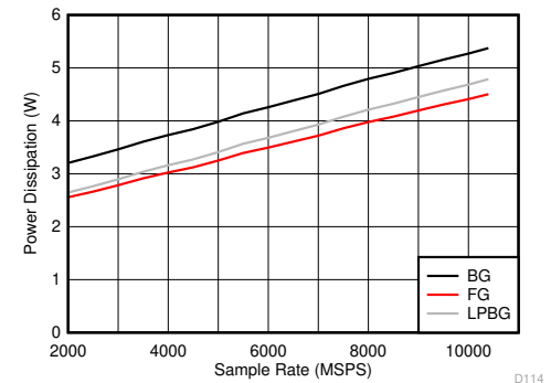
FIG 6-130. DES Mode: Power Dissipation vs Sample Rate
