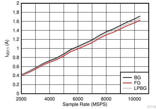
FIG 6-128. DES Mode: I_{VD11} vs Sample Rate
