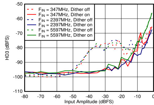
FIG 6-80. Dual Channel Mode: HD3 vs Input Amplitude and Dither
