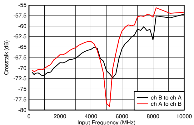
FIG 6-2. Crosstalk vs Input Frequency
