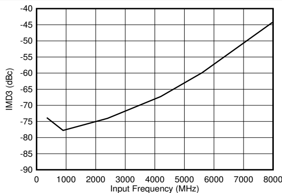
FIG 6-101. DES Mode: IMD3 vs Input Frequency
