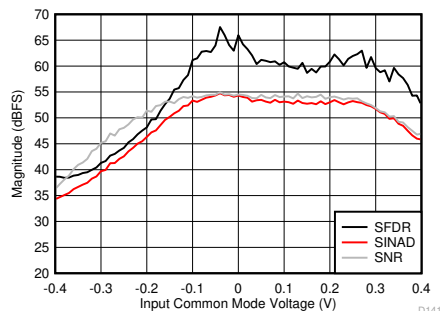
FIG 6-99. SNR, SFDR and SINAD vs Input Common Mode Voltage
