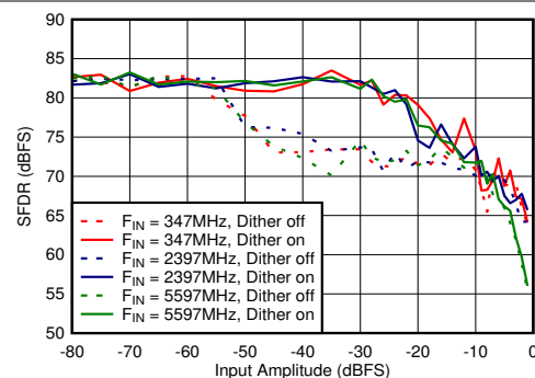
FIG 6-76. Dual Channel Mode: SFDR vs Input Amplitude and Dither
