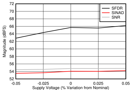
FIG 6-97. Dual Channel Mode: SNR, SINAD and SFDR vs Supply Voltage
