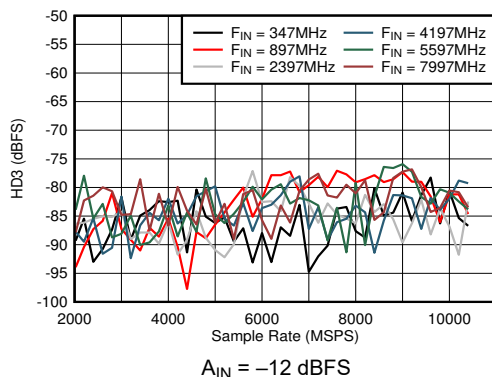
FIG 6-41. DES Mode: HD3 vs Sample Rate and Input Frequency
