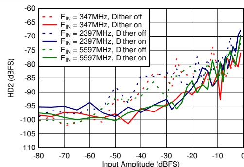
Figure 6-64. DES Mode: HD2 vs Input Amplitude and Dither
