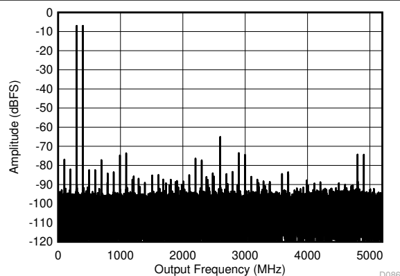
6-11. DES Mode: Two Tone FFT at 347 MHz
