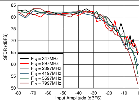
FIG 6-75. Dual Channel Mode: SFDR vs Input Amplitude and Frequency
