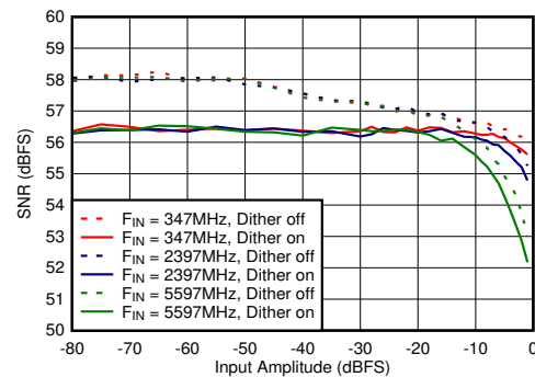
FIG 6-74. Dual Channel Mode: SNR vs Input Amplitude and Dither
