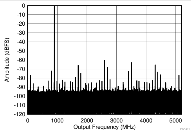
FIG 6-6. DES Mode: Single Tone FFT at 897 MHz
