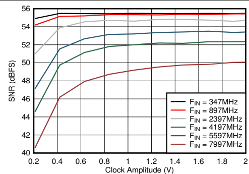
FIG 6-83. DES Mode: SNR vs Clock Amplitude
