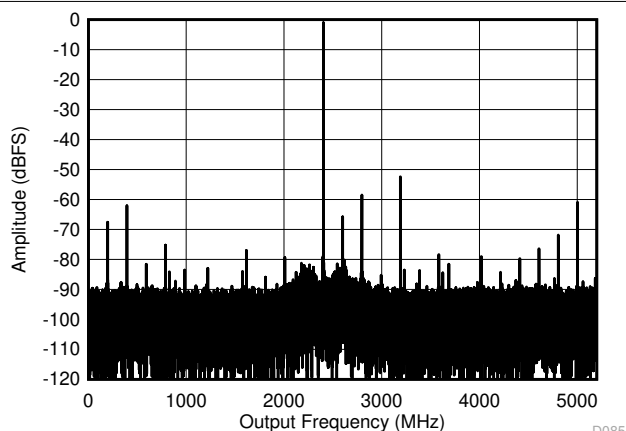
6-10. DES Mode: Single Tone FFT at 7997 MHz
