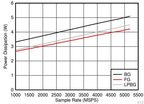
FIG 6-139. Dual Channel Mode: Power Dissipation vs Sample Rate
