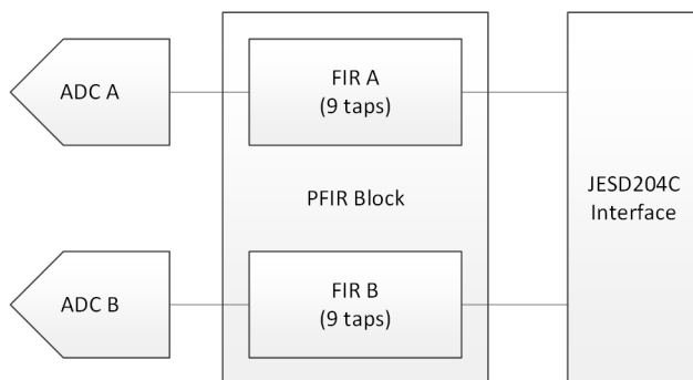
図 7-4. Dual Channel Equalization PFIR Block Diagram
