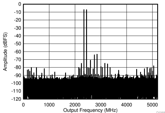
FIG 6-13. DES Mode: Two Tone FFT at 2397 MHz
