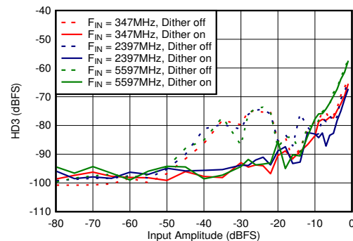
Figure 6-66. DES Mode: HD3 vs Input Amplitude and Dither
