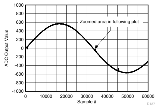
FIG 6-144. Background Calibration Core Transition (AC Signal)
