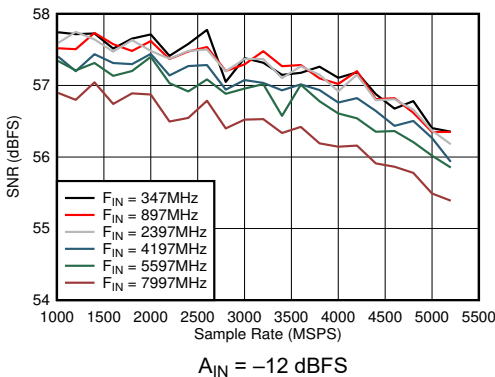
FIG 6-47. Dual Channel Mode: SNR vs Sample Rate and Input Frequency
