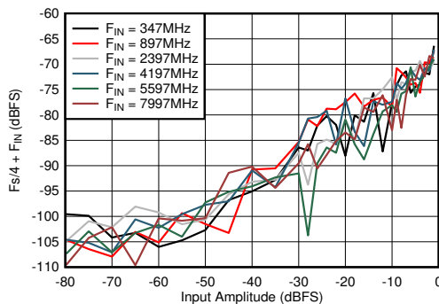
FIG 6-69. DES Mode: F_s/4 + F_{\text{IN}} vs Input Amplitude and Frequency
