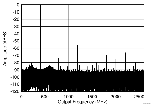
FIG 6-21. Dual Channel Mode: Single Tone FFT at 5597 MHz
