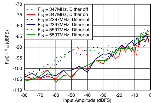
FIG 6-82. Dual Channel Mode: F_s/2 - F_{\text{IN}} vs Input Amplitude and Dither
