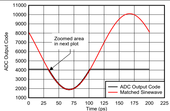
6-150. Sinewave Overdrive Recovery
