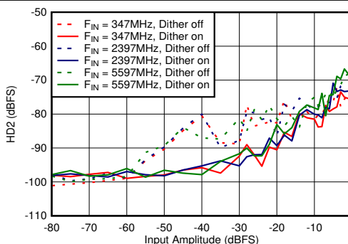
FIG 6-78. Dual Channel Mode: HD2 vs Input Amplitude and Dither
