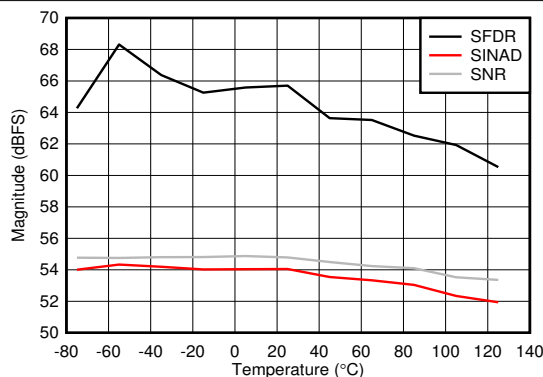
FIG 6-91. Dual Channel Mode: SNR, SINAD and SFDR vs Temperature
