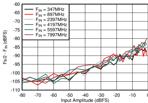
FIG 6-81. Dual Channel Mode: F_s/2 - F_{\text{IN}} vs Input Amplitude and Frequency
