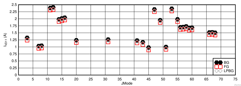
Figure 6-116. Dual Channel Mode: I_{VA11} vs JMODE at 5.2GSPS
