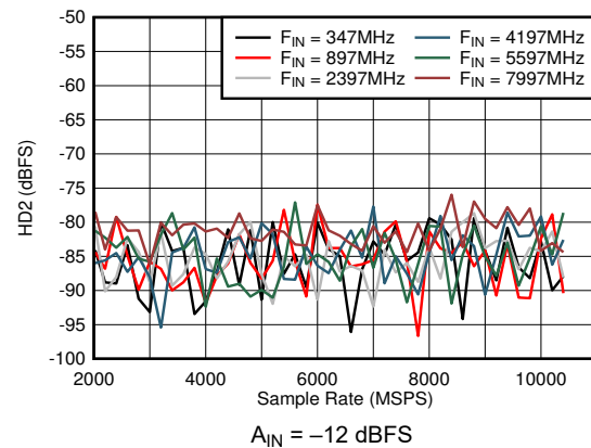
FIG 6-38. DES Mode: HD2 vs Sample Rate and Input Frequency
