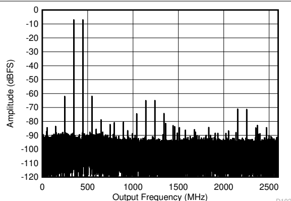
FIG 6-25. Dual Channel Mode: Two Tone FFT at 2397 MHz
