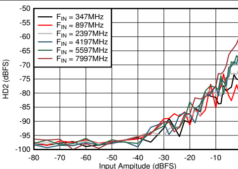
FIG 6-77. Dual Channel Mode: HD2 vs Input Amplitude and Frequency
