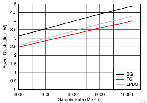
FIG 6-129. DES Mode: Power Dissipation vs Sample Rate
