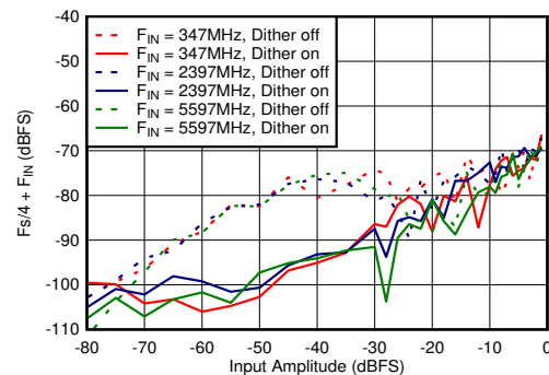
FIG 6-70. DES Mode: F_s/4 + F_{\text{IN}} vs Input Amplitude and Dither
