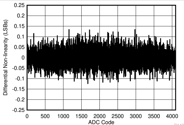
FIG 6-3. DNL vs ADC Code
