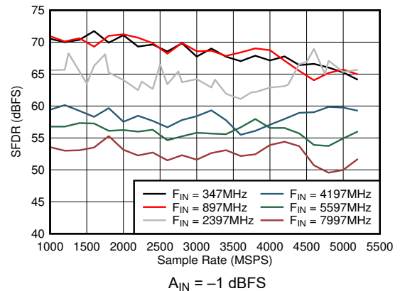
FIG 6-48. Dual Channel Mode: SFDR vs Sample Rate and Input Frequency
