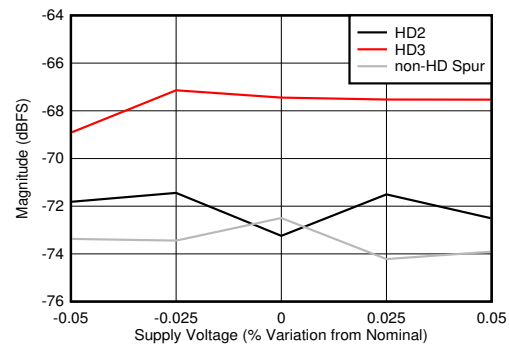
FIG 6-98. Dual Channel Mode: HD2, HD3 and Worst non-HD Spur vs Supply Voltage
