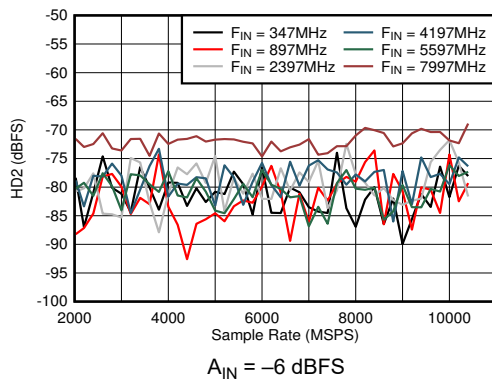
FIG 6-37. DES Mode: HD2 vs Sample Rate and Input Frequency
