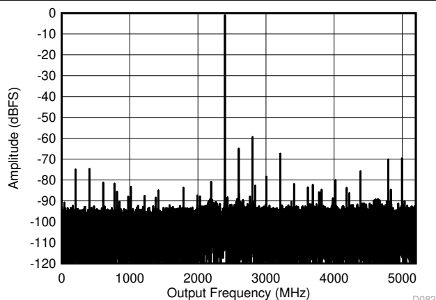
6-7. DES Mode: Single Tone FFT at 2397 MHz
