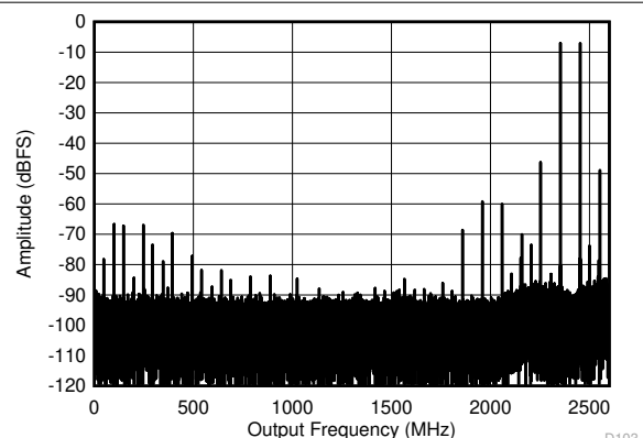
FIG 6-26. Dual Channel Mode: Two Tone FFT at 4197 MHz
