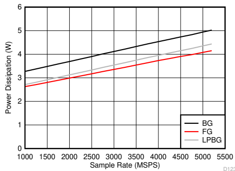
FIG 6-139. Dual Channel Mode: Power Dissipation vs Sample Rate
