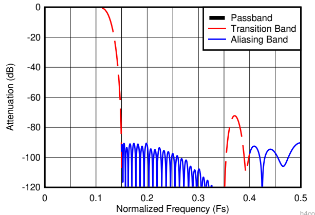
7-11. Decimate-by-4 Composite Response
