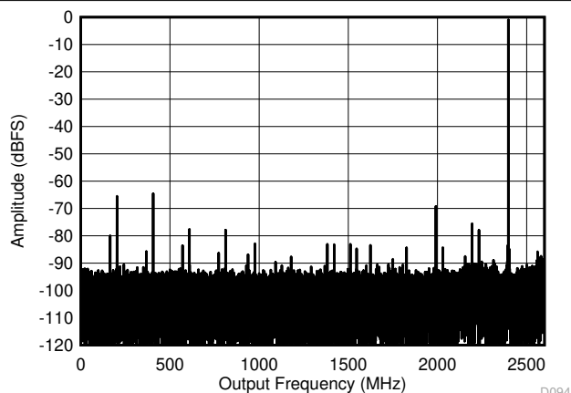
FIG 6-19. Dual Channel Mode: Single Tone FFT at 2397 MHz
