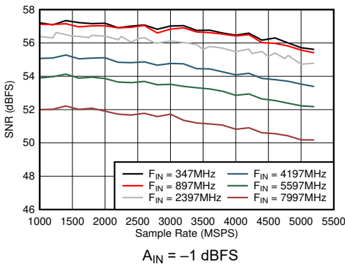
FIG 6-45. Dual Channel Mode: SNR vs Sample Rate and Input Frequency
