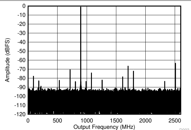
FIG 6-18. Dual Channel Mode: Single Tone FFT at 897 MHz
