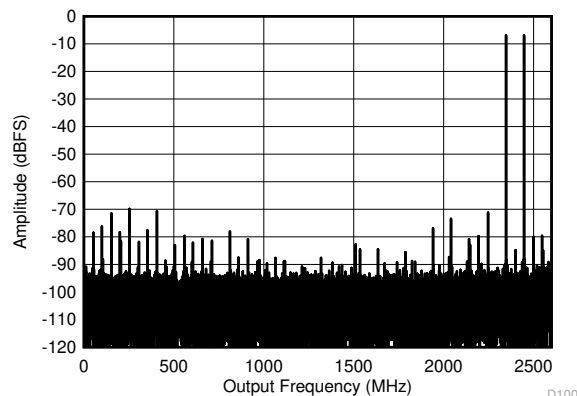
FIG 6-25. Dual Channel Mode: Two Tone FFT at 2397 MHz
