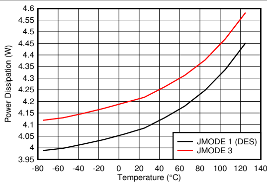
FIG 6-143. Power Dissipation vs Temperature
