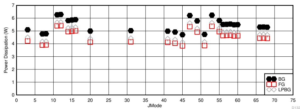
Figure 5-117. Dual Channel Mode: I_{VD11} vs JMODE at 5.2GSPS
