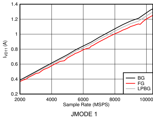
図 5-125. DES Mode: I_{VD11} vs Sample Rate
