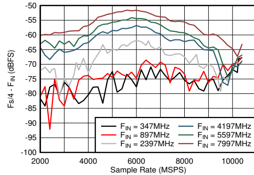
FIG 5-44. DES Mode: F_s/4 - F_{\text{IN}} vs Sample Rate and Input Frequency
