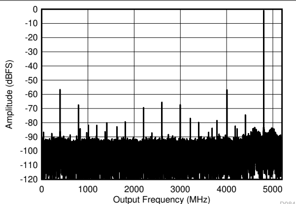
FIG 5-9. DES Mode: Single Tone FFT at 5597 MHz
