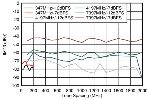
FIG 5-103. DES Mode: IMD3 vs Tone Spacing
