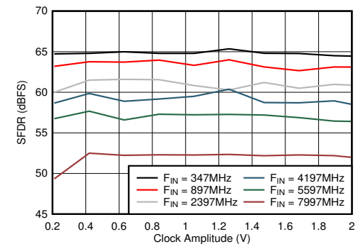
図 5-84. DES Mode: SFDR vs Clock Amplitude
