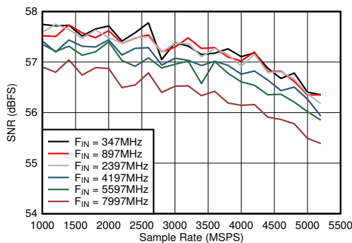
FIG 5-45. Dual Channel Mode: SNR vs Sample Rate and Input Frequency
