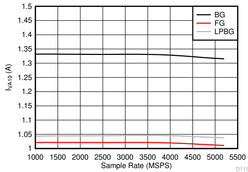
FIG 5-133. Dual Channel Mode: I_{VA19} vs Sample Rate
