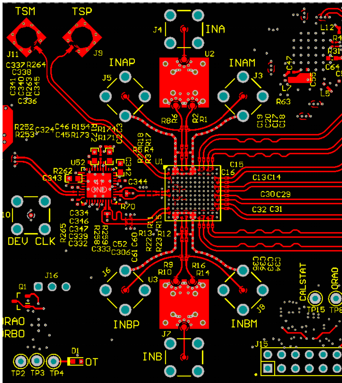
図 7-7. Top Layer Routing: Analog Inputs, CLK and SYSREF, DA0-3, DB0-3
