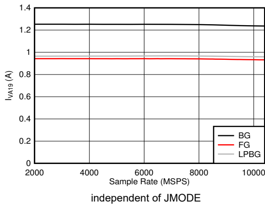
図 5-123. DES Mode: I_{VA19} vs Sample Rate
