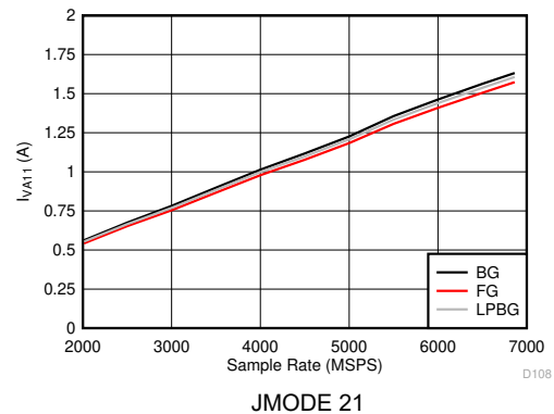
図 5-126. DES Mode: I_{VD11} vs Sample Rate
