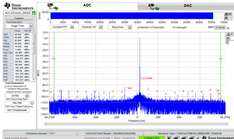
7-4. FFT for 497.77-MHz Input Signal, 2.7 GSPS, Decimation-by-16, f_{NCO} = 500 MHz, JMODE16
