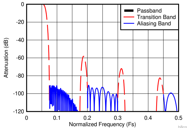
Figure 6-13. Decimate-by-8 Composite Response
