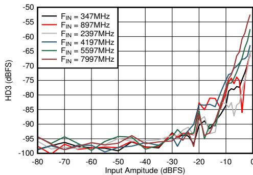
図 5-65. DES Mode: HD3 vs Input Amplitude and Frequency
