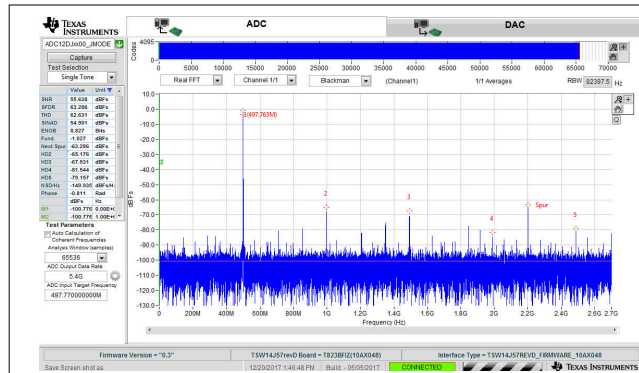
7-2. FFT for 497.77-MHz Input Signal, 5.4 GSPS, JMODE0
