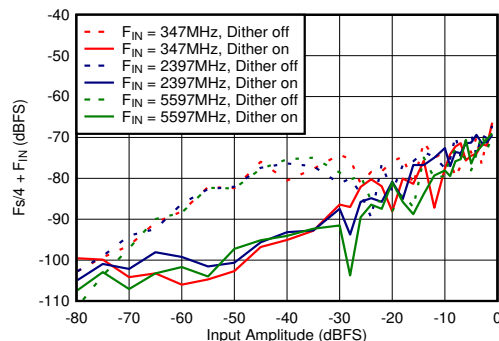
FIG 5-68. DES Mode: F_s/2 - F_{\text{IN}} vs Input Amplitude and Dither
