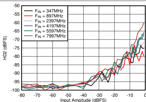
図 5-77. Dual Channel Mode: HD2 vs Input Amplitude and Frequency
