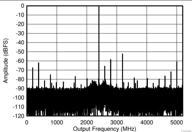
FIG 5-10. DES Mode: Single Tone FFT at 7997 MHz
