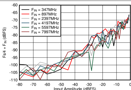
FIG 5-69. DES Mode: F_s/4 + F_{\text{IN}} vs Input Amplitude and Frequency
