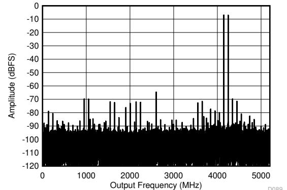
FIG 5-14. DES Mode: Two Tone FFT at 4197 MHz
