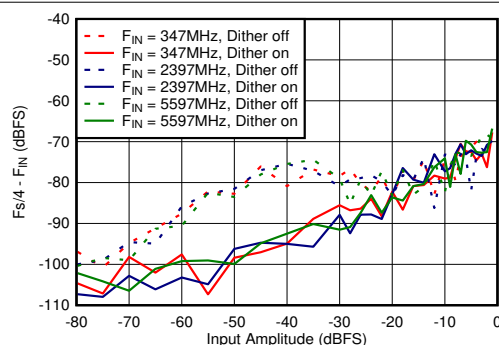
FIG 5-72. DES Mode: F_s/4 - F_{\text{IN}} vs Input Amplitude and Dither
