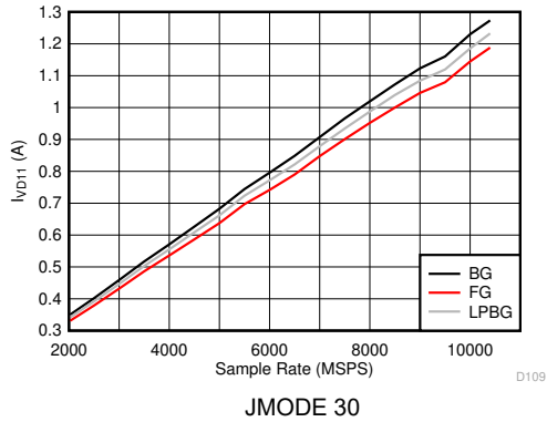
5-127. DES Mode: I_{VD11} vs Sample Rate
