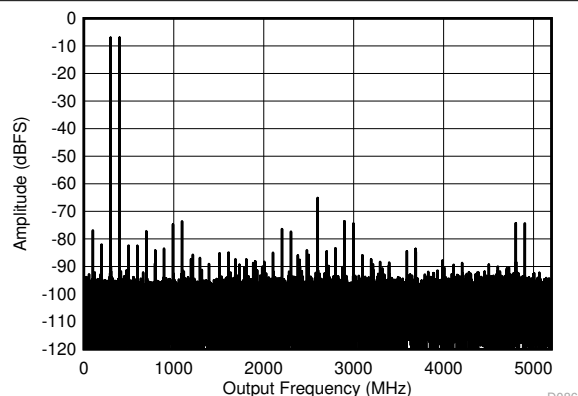
FIG 5-11. DES Mode: Two Tone FFT at 347 MHz
