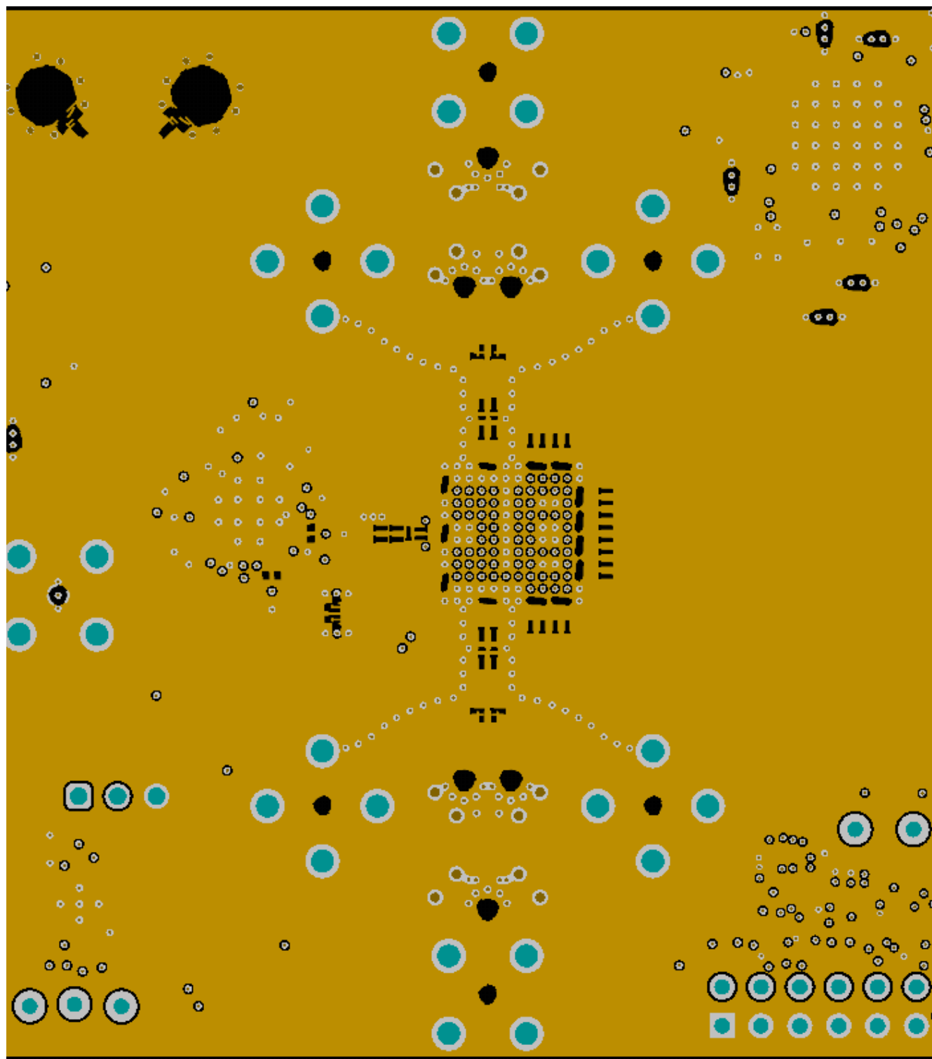
図 7-8. GND1 Cutouts to Optimize Impedance of Component Pads
