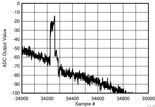
FIG 5-145. Background Calibration Core Transition (AC Signal - zoomed)
