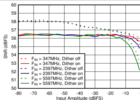
図 5-74. Dual Channel Mode: SNR vs Input Amplitude and Dither
