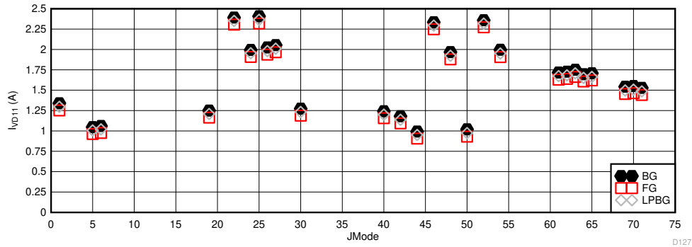
図 5-113. DES Mode: I_{VD11} vs JMODE at 10.4GSPS
