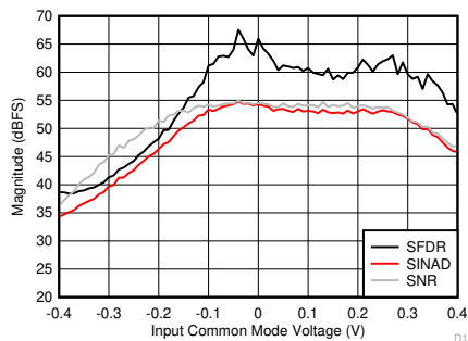
Figure 5-99. SNR, SFDR and SINAD vs Input Common Mode Voltage
