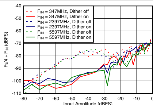
FIG 5-70. DES Mode: F_s/4 + F_{\text{IN}} vs Input Amplitude and Dither
