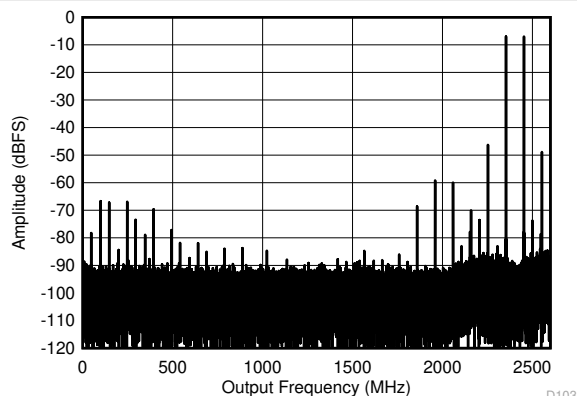
FIG 5-26. Dual Channel Mode: Two Tone FFT at 4197 MHz
