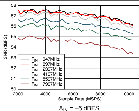
FIG 5-30. DES Mode: SNR vs Sample Rate and Input Frequency
