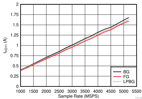
FIG 5-136. Dual Channel Mode: I_{VD11} vs Sample Rate
