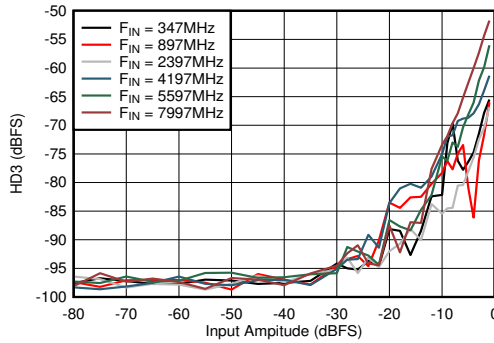
図 5-79. Dual Channel Mode: HD3 vs Input Amplitude and Frequency
