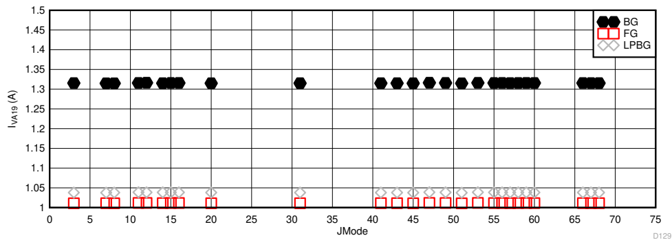
図 5-114. DES Mode: Power Dissipation vs JMODE at 10.4GSPS
