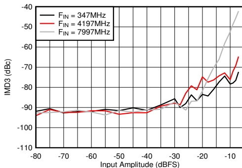
FIG 5-107. Dual Channel Mode: IMD3 vs Input Amplitude
