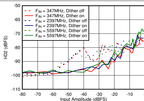
図 5-78. Dual Channel Mode: HD2 vs Input Amplitude and Dither
