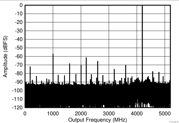
FIG 5-8. DES Mode: Single Tone FFT at 4197 MHz
