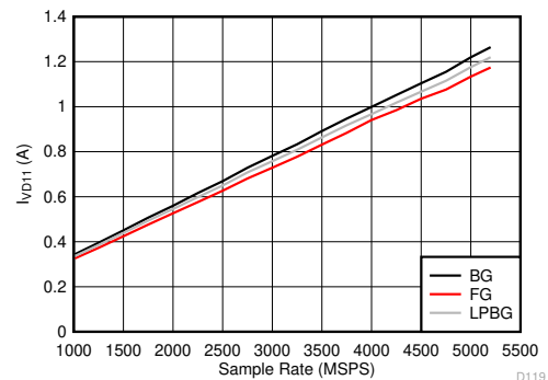
FIG 5-135. Dual Channel Mode: I_{VD11} vs Sample Rate
