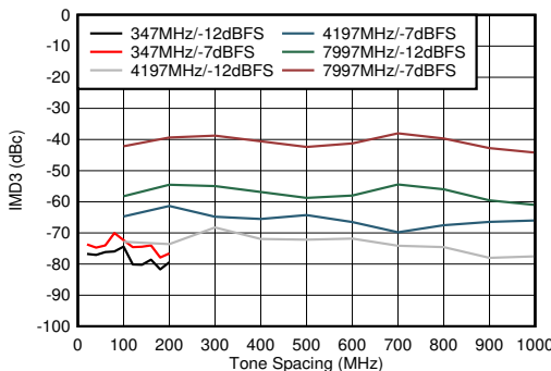
FIG 5-108. Dual Channel Mode: IMD3 vs Tone Spacing
