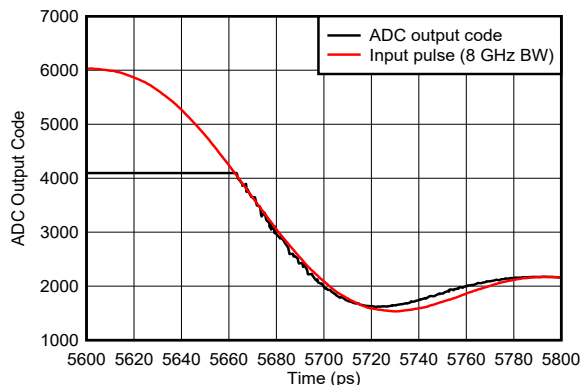
FIG 5-149. Pulse Overdrive Recovery Zoomed
