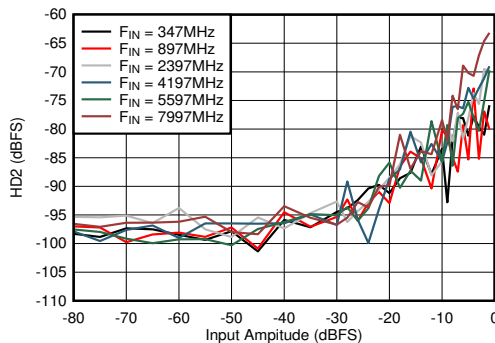
図 5-63. DES Mode: HD2 vs Input Amplitude and Frequency
