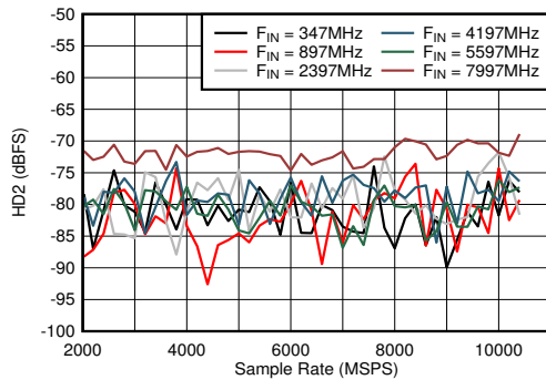
図 5-37. DES Mode: HD2 vs Sample Rate and Input Frequency
