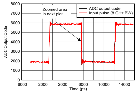
FIG 5-148. Pulse Overdrive Recovery
