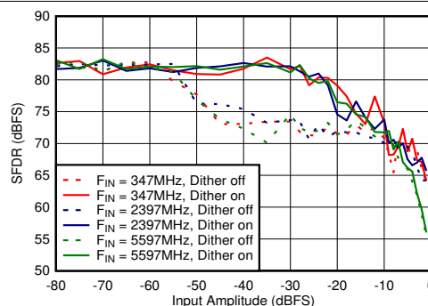
図 5-76. Dual Channel Mode: SFDR vs Input Amplitude and Dither
