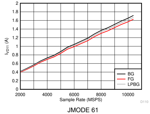
5-128. DES Mode: I_{VD11} vs Sample Rate
