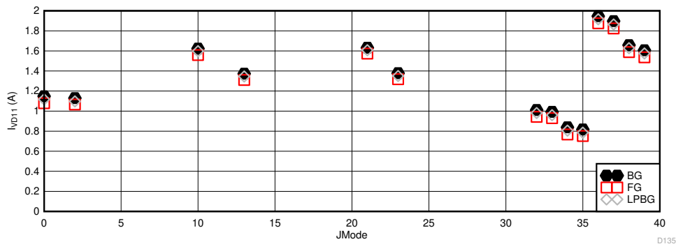
図 5-120. Other Modes with Lower Maximum FS: I_{VA11} vs JMODE
