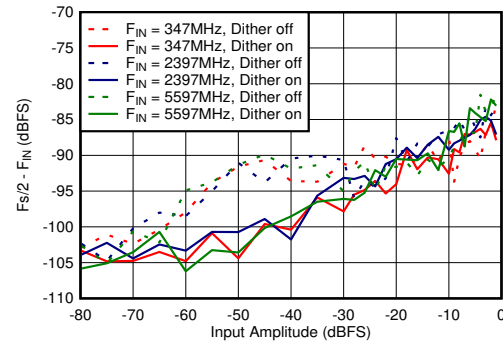
図 5-82. Dual Channel Mode: F_s/2 - F_{\text{IN}} vs Input Amplitude and Dither
