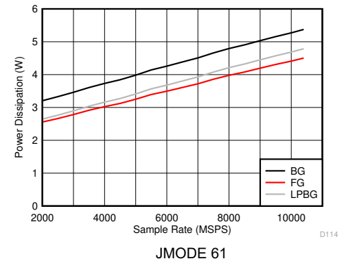
5-132. DES Mode: Power Dissipation vs Sample Rate
