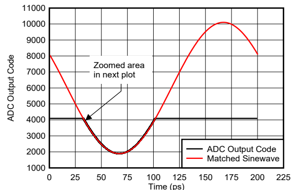
FIG 5-150. Sinewave Overdrive Recovery
