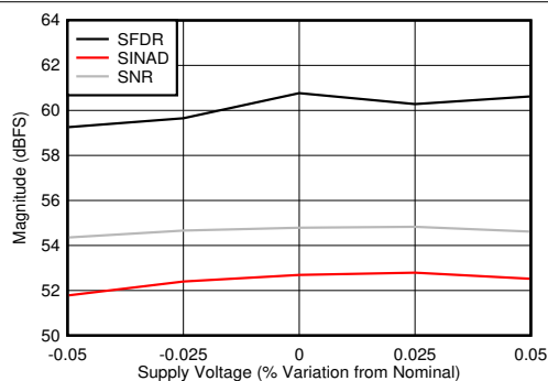
FIG 5-95. DES Mode: SNR, SINAD and SFDR vs Supply Voltage
