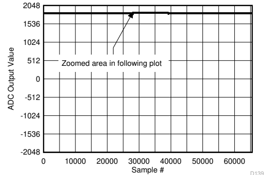
FIG 5-146. Background Calibration Core Transition (DC Signal)
