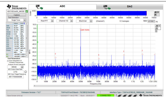
7-3. FFT for 497.77-MHz Input Signal, 2.7 GSPS, JMODE2
