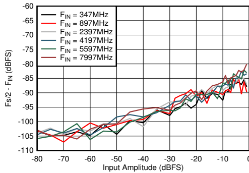
図 5-81. Dual Channel Mode: F_s/2 - F_{\text{IN}} vs Input Amplitude and Frequency
