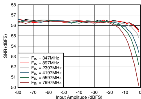
図 5-73. Dual Channel Mode: SNR vs Input Amplitude and Frequency
