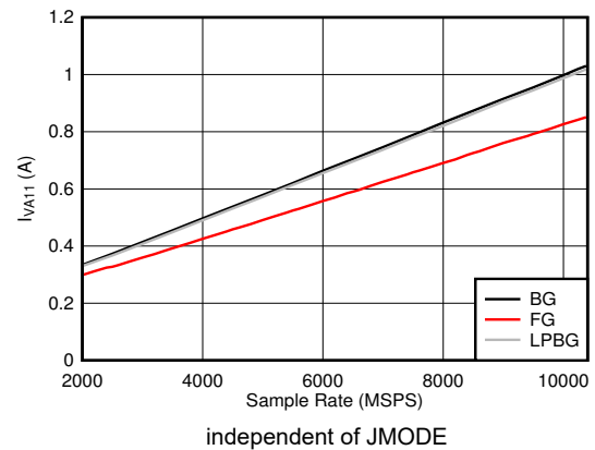
図 5-124. DES Mode: I_{VA11} vs Sample Rate
