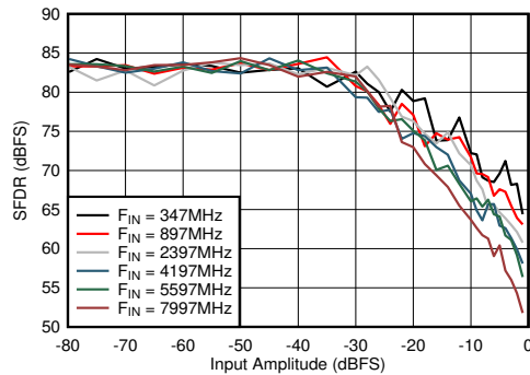
図 5-61. DES Mode: SFDR vs Input Amplitude and Frequency
