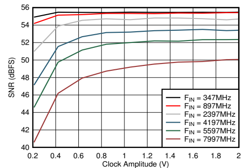
図 5-83. DES Mode: SNR vs Clock Amplitude
