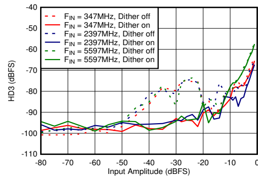
図 5-66. DES Mode: HD3 vs Input Amplitude and Dither
