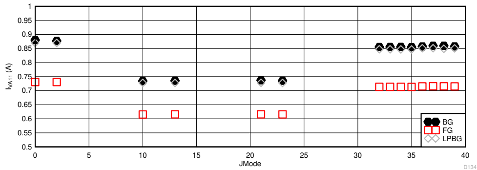
図 5-119. Other Modes with Lower Maximum FS: I_{VA19} vs JMODE
