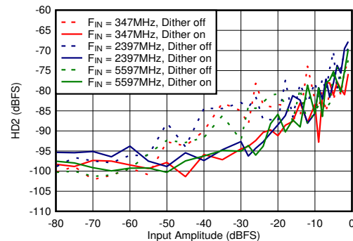
図 5-64. DES Mode: HD2 vs Input Amplitude and Dither
