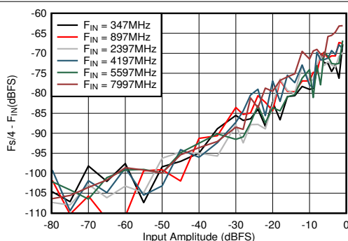
FIG 5-71. DES Mode: F_s/4 - F_{\text{IN}} vs Input Amplitude and Frequency
