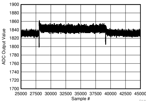
FIG 5-147. Background Calibration Core Transition (DC Signal - zoomed)
