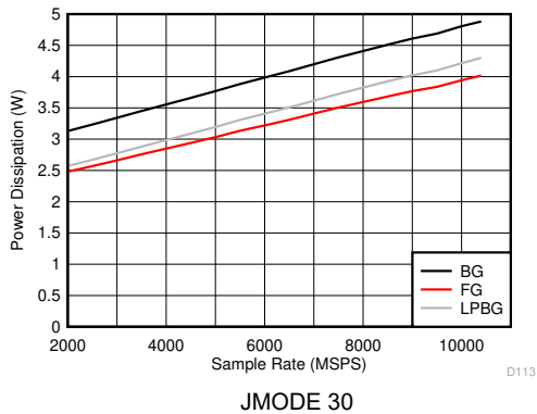
5-131. DES Mode: Power Dissipation vs Sample Rate
