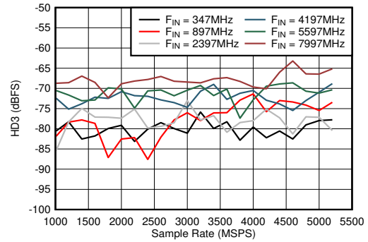
5-56. Dual Channel Mode: HD3 vs Sample Rate and Input Frequency
