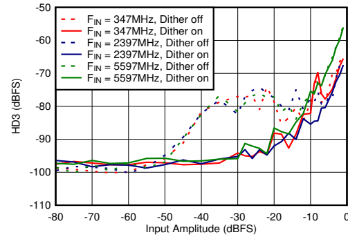
図 5-80. Dual Channel Mode: HD3 vs Input Amplitude and Dither
