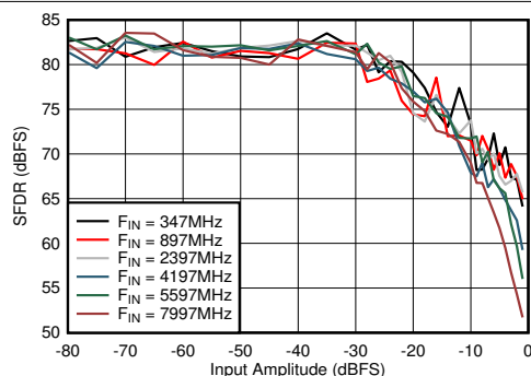
図 5-75. Dual Channel Mode: SFDR vs Input Amplitude and Frequency
