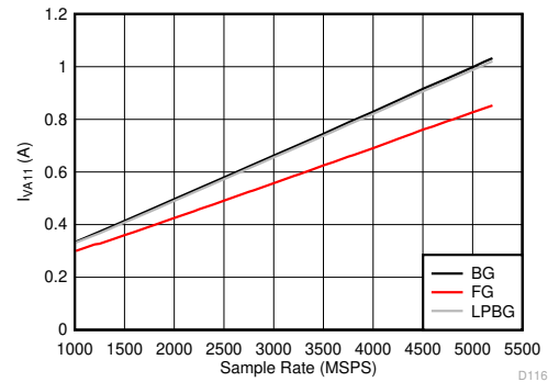
FIG 5-134. Dual Channel Mode: I_{VA11} vs Sample Rate
