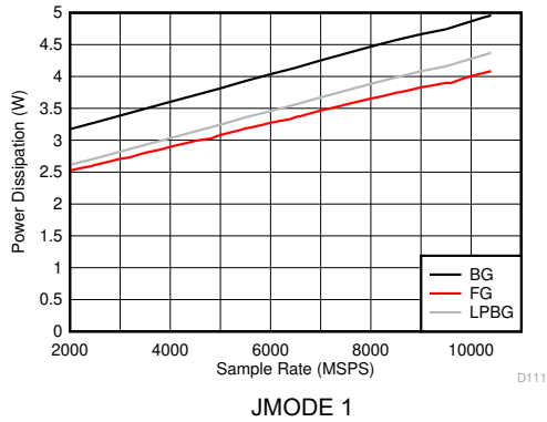
5-129. DES Mode: Power Dissipation vs Sample Rate
