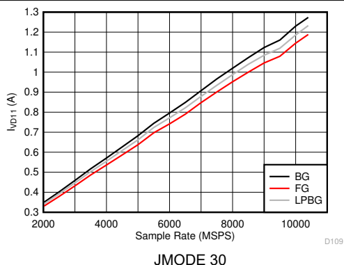
FIG 6-127. DES Mode: I_{VD11} vs Sample Rate
