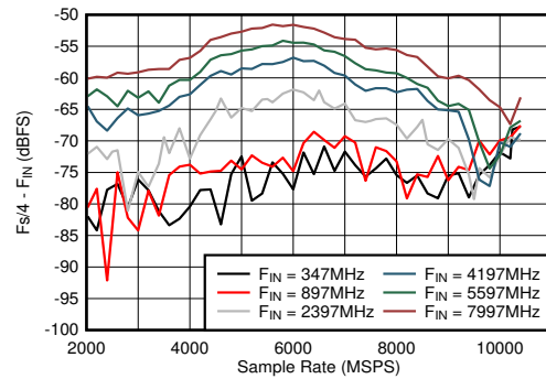
FIG 6-44. DES Mode: F_s/4 - F_{\text{IN}} vs Sample Rate and Input Frequency
