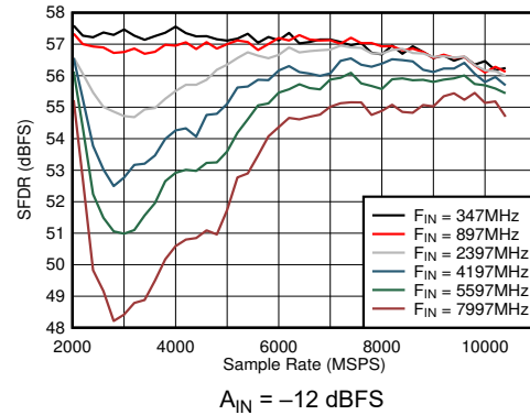
FIG 6-34. DES Mode: SFDR vs Sample Rate and Input Frequency
