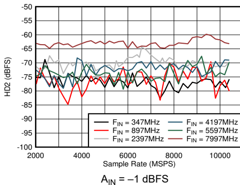
FIG 6-35. DES Mode: HD2 vs Sample Rate and Input Frequency
