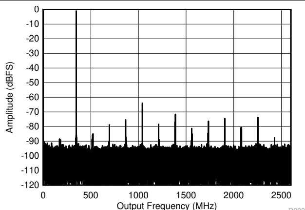
FIG 6-17. Dual Channel Mode: Single Tone FFT at 347 MHz
