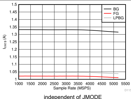
FIG 6-133. Dual Channel Mode: I_{VA19} vs Sample Rate
