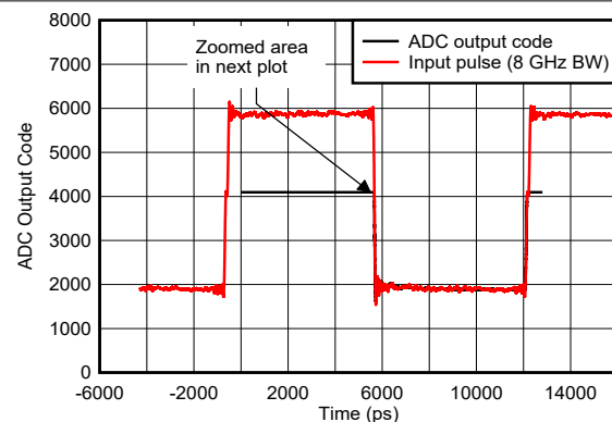
FIG 6-148. Pulse Overdrive Recovery
