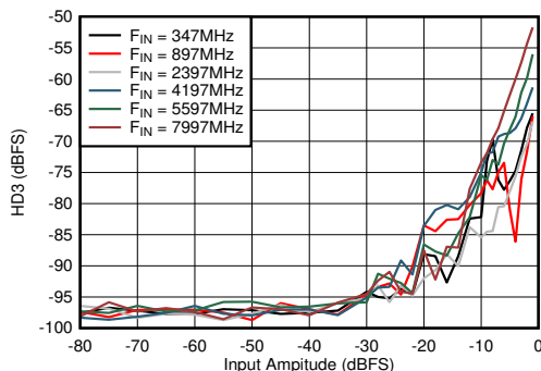
FIG 6-79. Dual Channel Mode: HD3 vs Input Amplitude and Frequency
