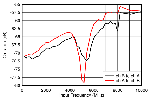
图 6-2. Crosstalk vs Input Frequency
