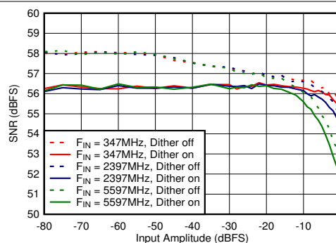
Figure 6-60. DES Mode: SNR vs Input Amplitude and Dither
