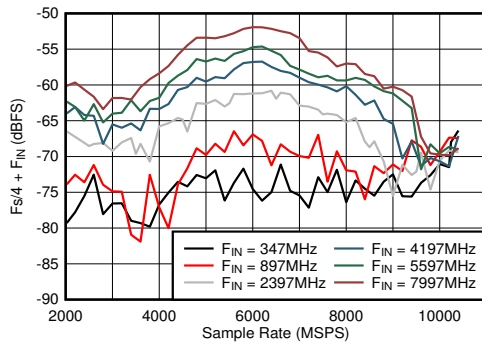
FIG 6-43. DES Mode: F_s/4 + F_{\text{IN}} vs Sample Rate and Input Frequency
