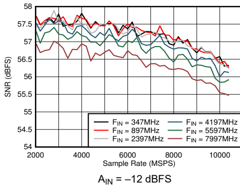
FIG 6-31. DES Mode: SNR vs Sample Rate and Input Frequency
