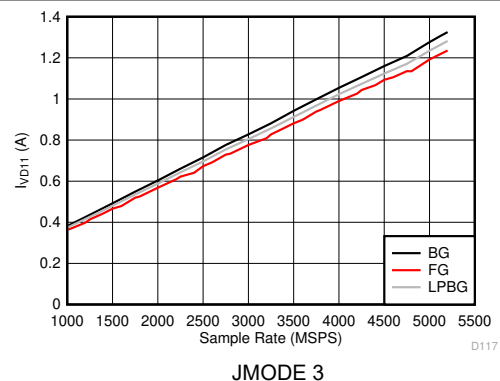
FIG 6-135. Dual Channel Mode: I_{VD11} vs Sample Rate
