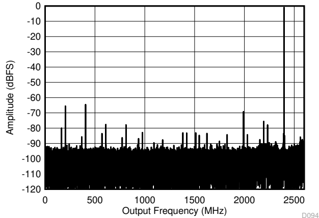
FIG 6-19. Dual Channel Mode: Single Tone FFT at 2397 MHz
