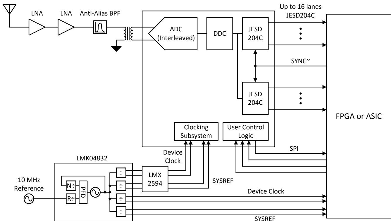
8-1. Typical Configuration for Wideband RF Sampling
