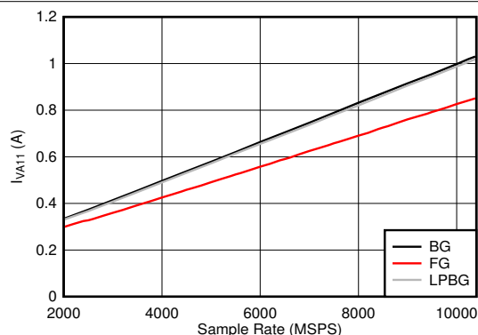
图 6-124. DES Mode: I_{VA11} vs Sample Rate
