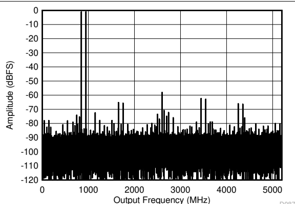
FIG 6-10. DES Mode: Single Tone FFT at 7997 MHz
