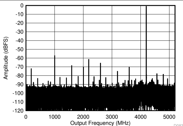
FIG 6-8. DES Mode: Single Tone FFT at 4197 MHz
