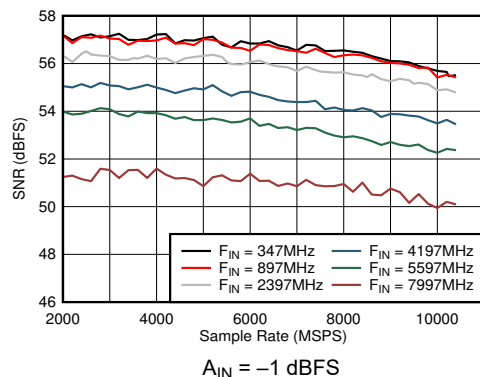
FIG 6-29. DES Mode: SNR vs Sample Rate and Input Frequency
