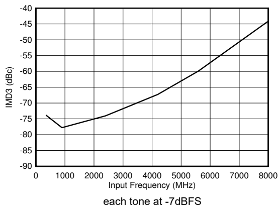
FIG 6-101. DES Mode: IMD3 vs Input Frequency
