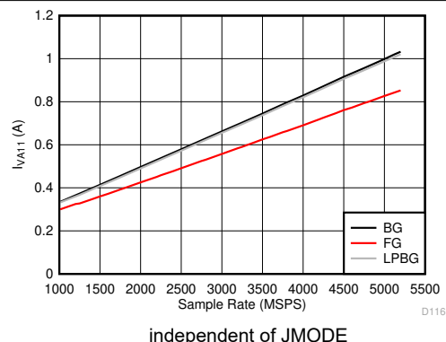
FIG 6-134. Dual Channel Mode: I_{VA11} vs Sample Rate
