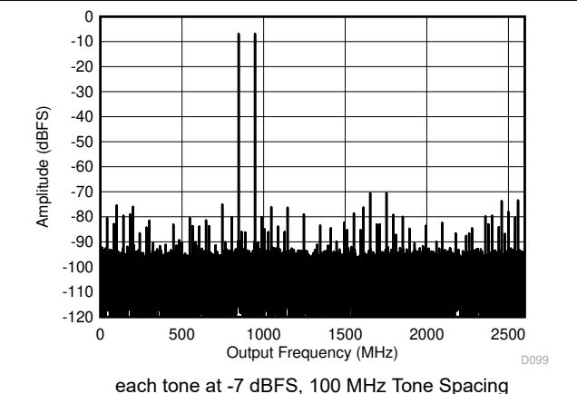
FIG 6-24. Dual Channel Mode: Two Tone FFT at 897 MHz
