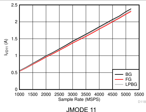
FIG 6-136. Dual Channel Mode: I_{VD11} vs Sample Rate
