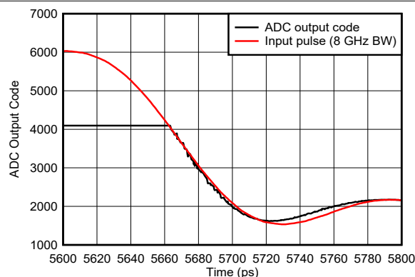
FIG 6-149. Pulse Overdrive Recovery Zoomed
