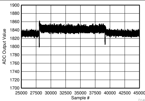
FIG 6-147. Background Calibration Core Transition (DC Signal - zoomed)
