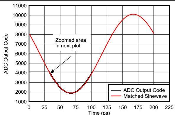
FIG 6-150. Sinewave Overdrive Recovery
