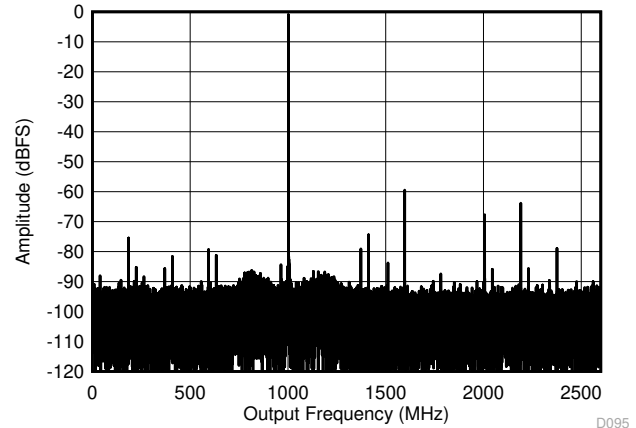
FIG 6-20. Dual Channel Mode: Single Tone FFT at 4197 MHz
