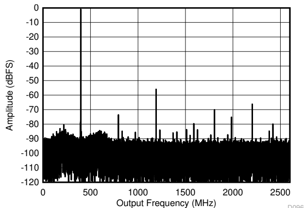
FIG 6-21. Dual Channel Mode: Single Tone FFT at 5597 MHz
