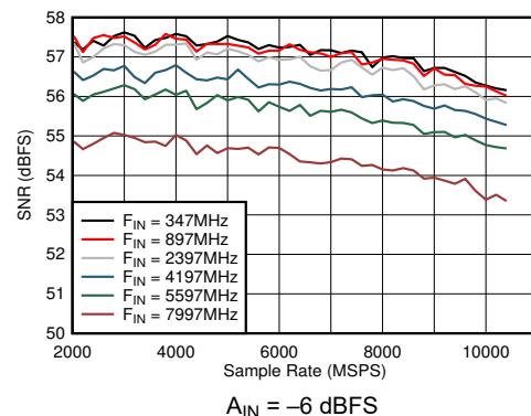
FIG 6-30. DES Mode: SNR vs Sample Rate and Input Frequency
