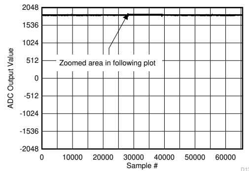
FIG 6-146. Background Calibration Core Transition (DC Signal)
