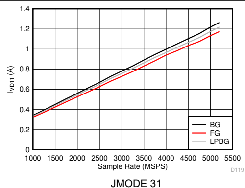
FIG 6-137. Dual Channel Mode: I_{VD11} vs Sample Rate
