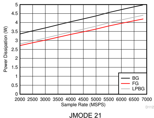
FIG 6-130. DES Mode: Power Dissipation vs Sample Rate
