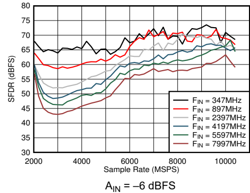
FIG 6-33. DES Mode: SFDR vs Sample Rate and Input Frequency
