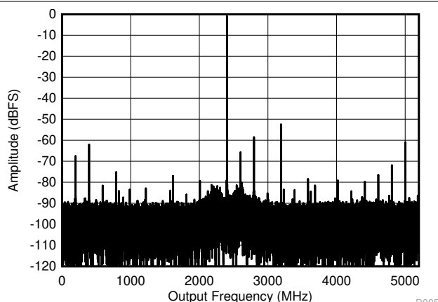
FIG 6-10. DES Mode: Single Tone FFT at 7997 MHz
