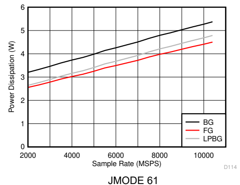
FIG 6-132. DES Mode: Power Dissipation vs Sample Rate
