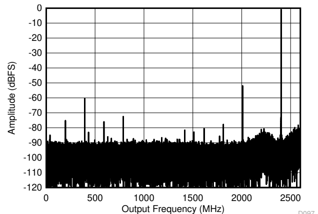
FIG 6-22. Dual Channel Mode: Single Tone FFT at 7997 MHz
