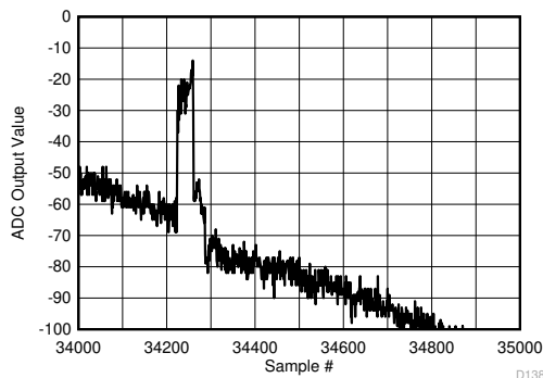
FIG 6-145. Background Calibration Core Transition (AC Signal - zoomed)
