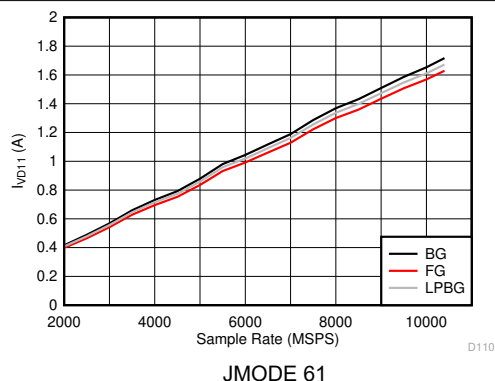
FIG 6-128. DES Mode: I_{VD11} vs Sample Rate
