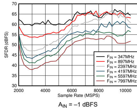
FIG 6-32. DES Mode: SFDR vs Sample Rate and Input Frequency
