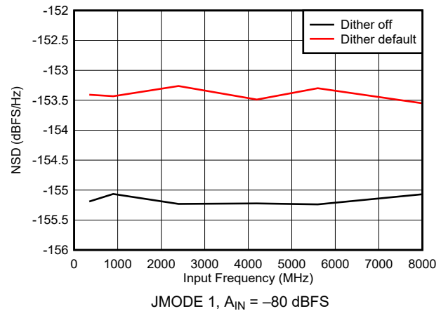
FIG 6-36. DES Mode: NSD vs Input Frequency
