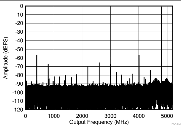
FIG 6-9. DES Mode: Single Tone FFT at 5597 MHz
