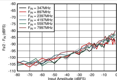
FIG 6-81. Dual Channel Mode: F_s/2 - F_{\text{IN}} vs Input Amplitude and Frequency
