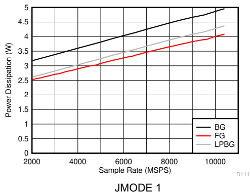
FIG 6-129. DES Mode: Power Dissipation vs Sample Rate
