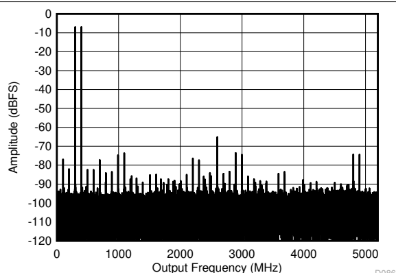
FIG 6-11. DES Mode: Two Tone FFT at 347 MHz
