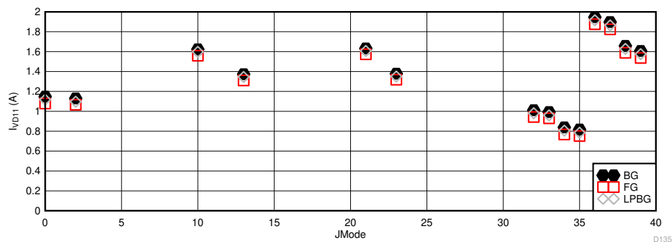
図 6-120. Other Modes with Lower Maximum F_S : I_{V_{A11}} vs JMODE
