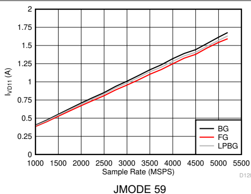
FIG 6-138. Dual Channel Mode: I_{VD11} vs Sample Rate
